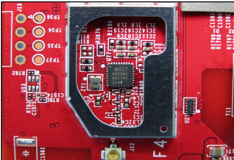
BT chip
