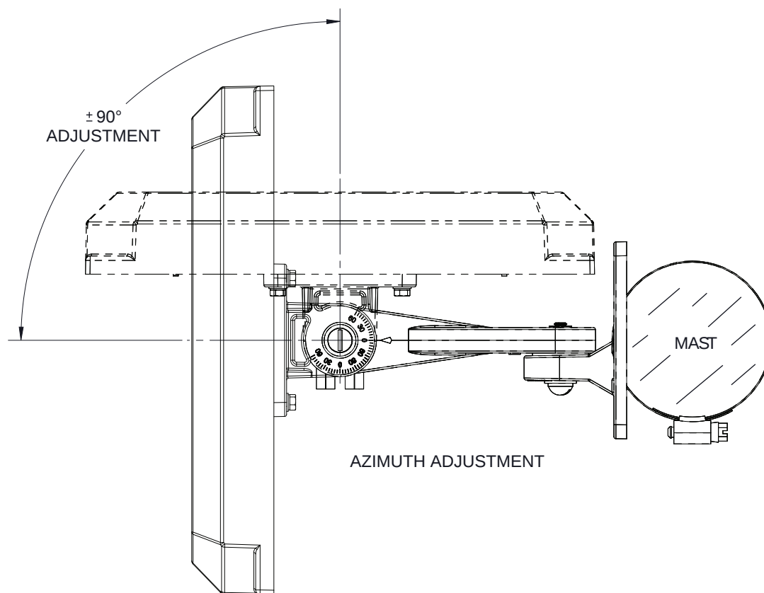
Figure 7 Azimuth Adjustment
