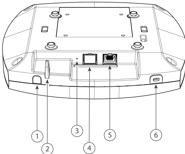
Figure 2: CW9176D1 Top View with Connectors and Ports
