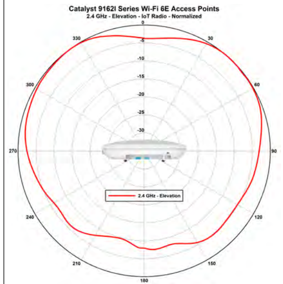
Figure 16: CW9162I - IoT Antenna-Normalized Radiation Pattern (2.4-GHz Elevation)
