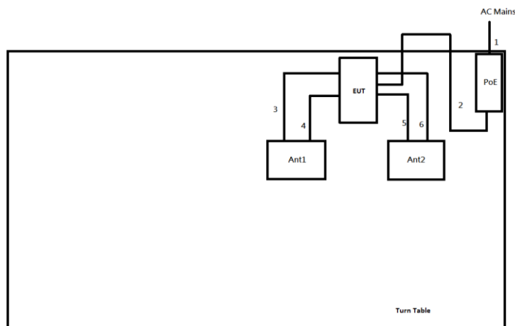
Test Setup Diagram – AC Line Conducted Emission Test (Group 2/3/4)
