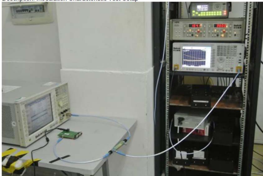
Description: Modulation Characteristic Test Setup
