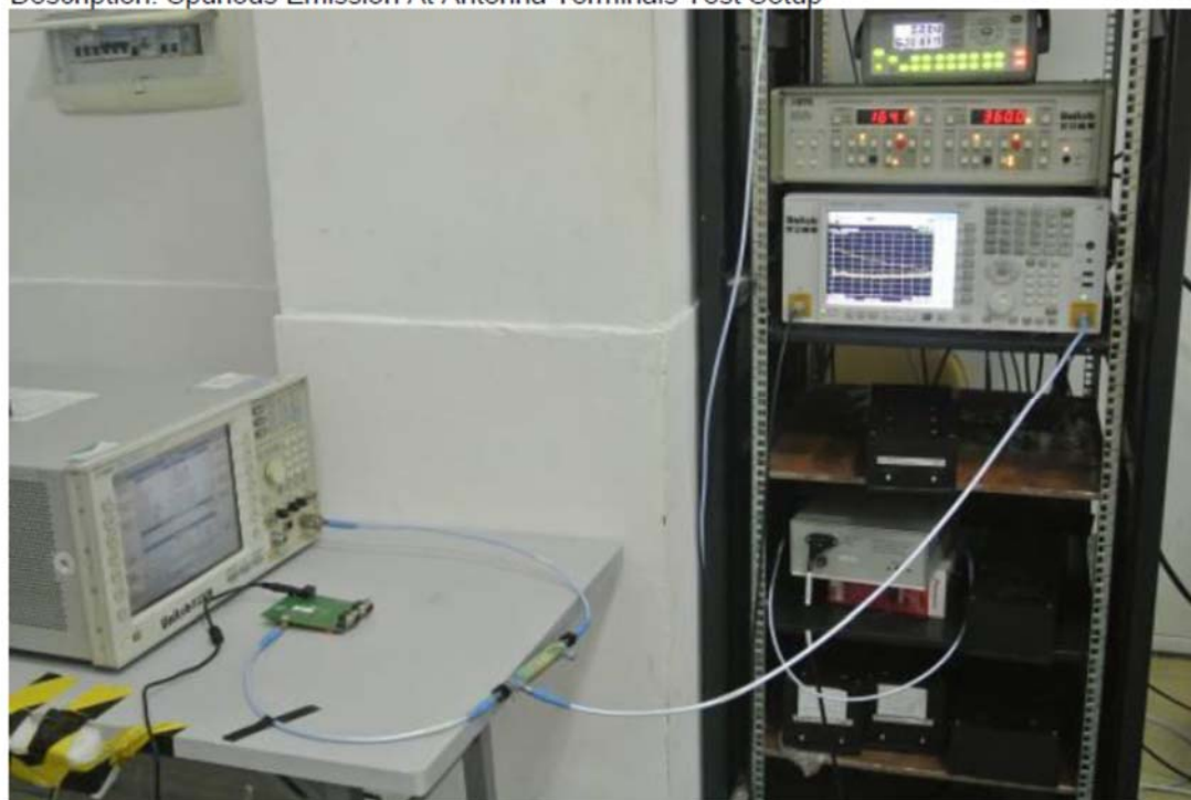
Description: Spurious Emission At Antenna Terminals Test Setup
