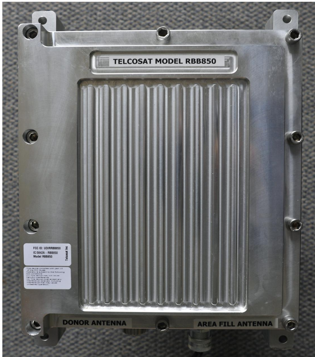
FRONT OF REPEATER WITH COVER PLATE ATTACHED
