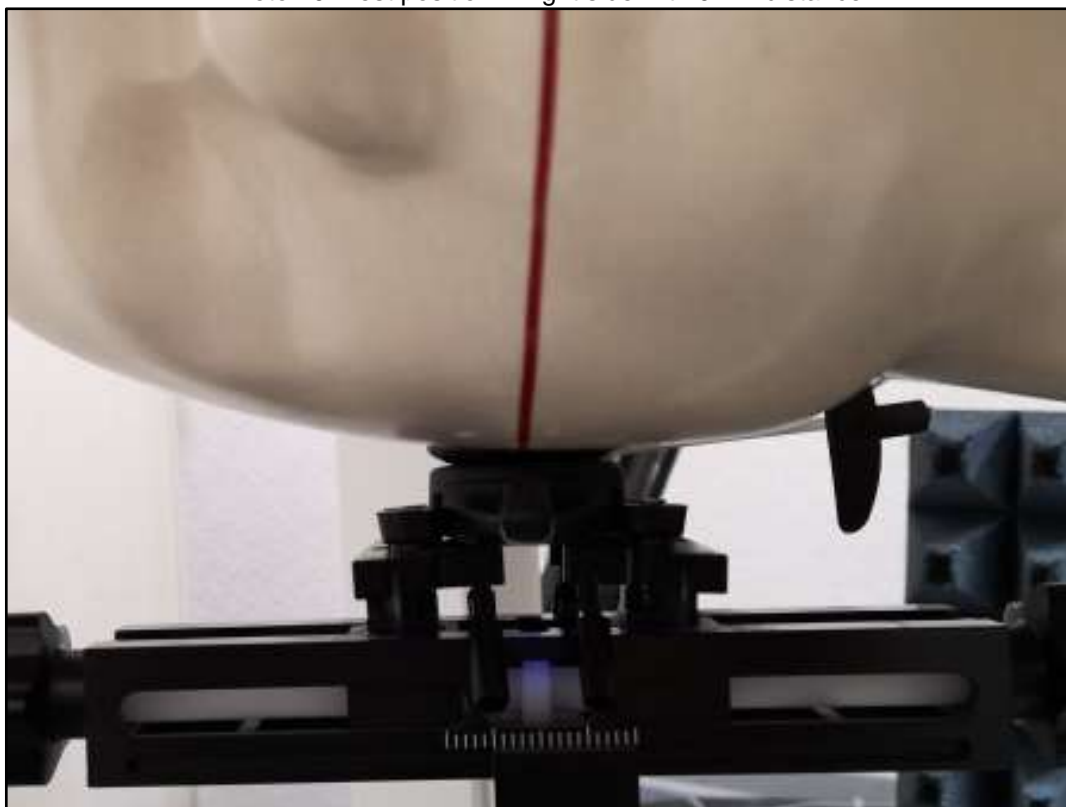
Photo 10: Test position - Right side with 0mm distance
