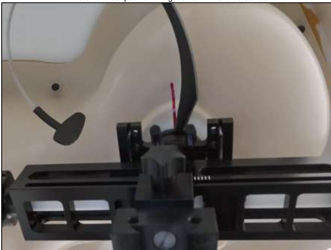
Photo 12: Test position - Right side with 0mm distance
