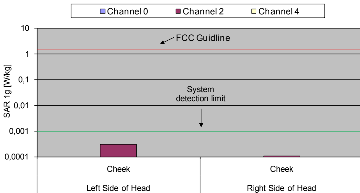
Fig. 8: The measured head phantom SAR values for the US DECT standard in comparison to the FCC exposure limit.
