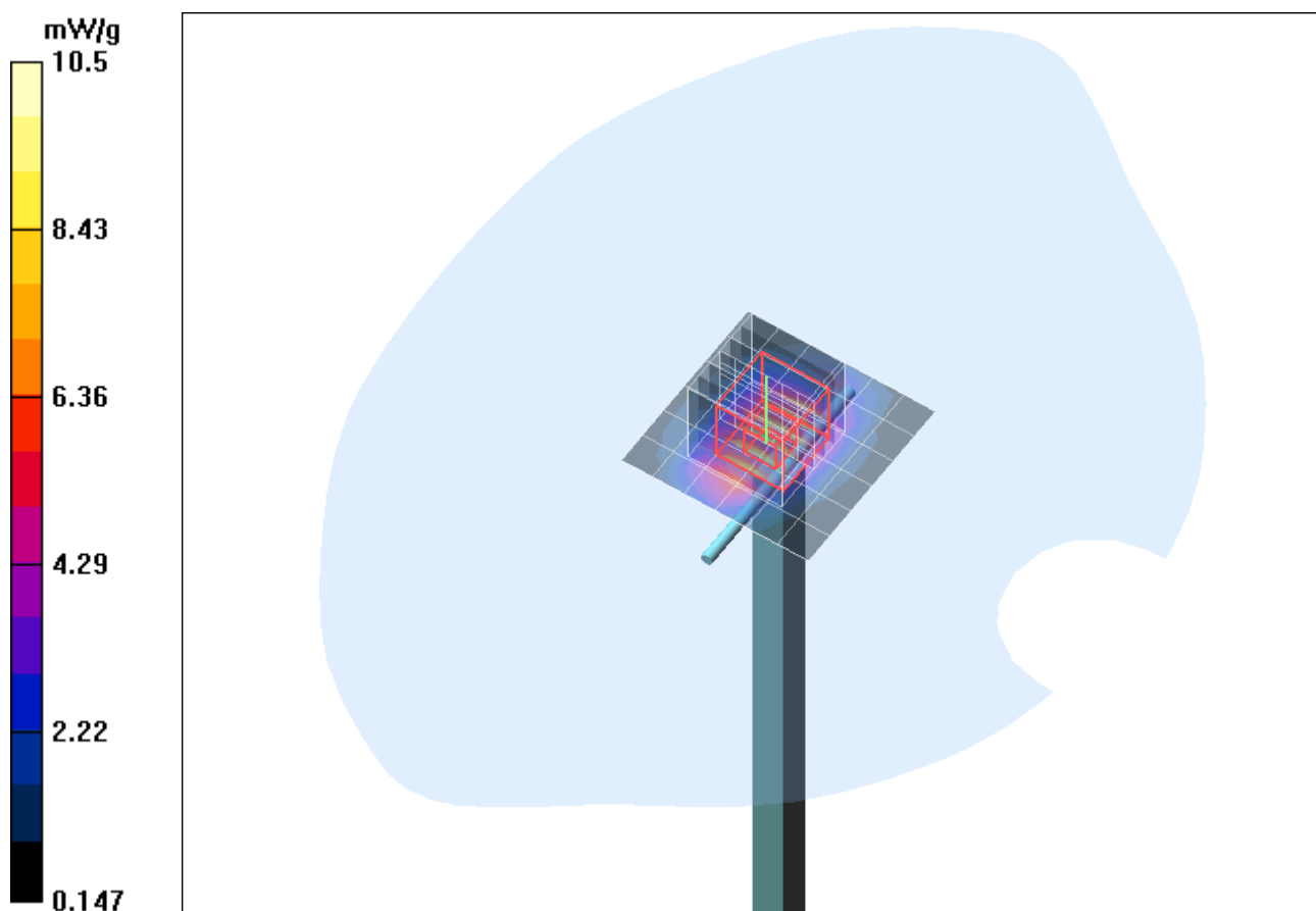
Fig. 9 Validation measurement 1900 MHz Head (January 24, 2011), coarse grid. Ambient Temperature: 21.1° C, Liquid Temperature: 20.7° C.
