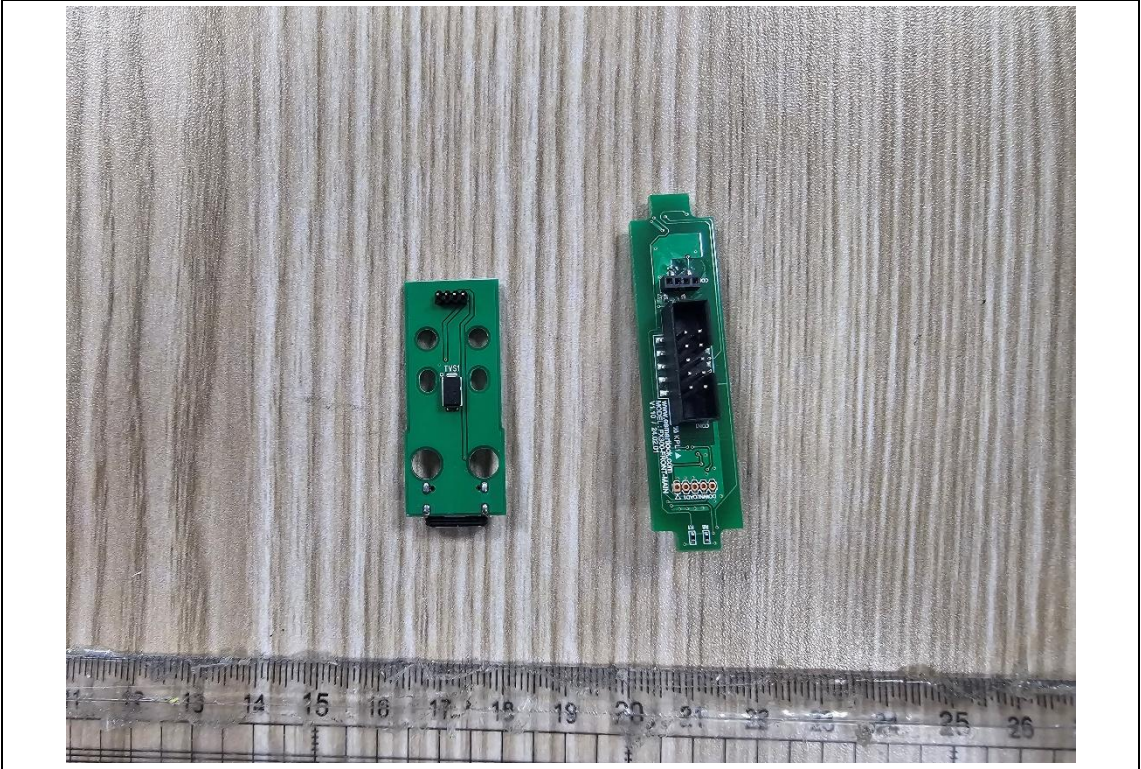
Board 3 Rear
