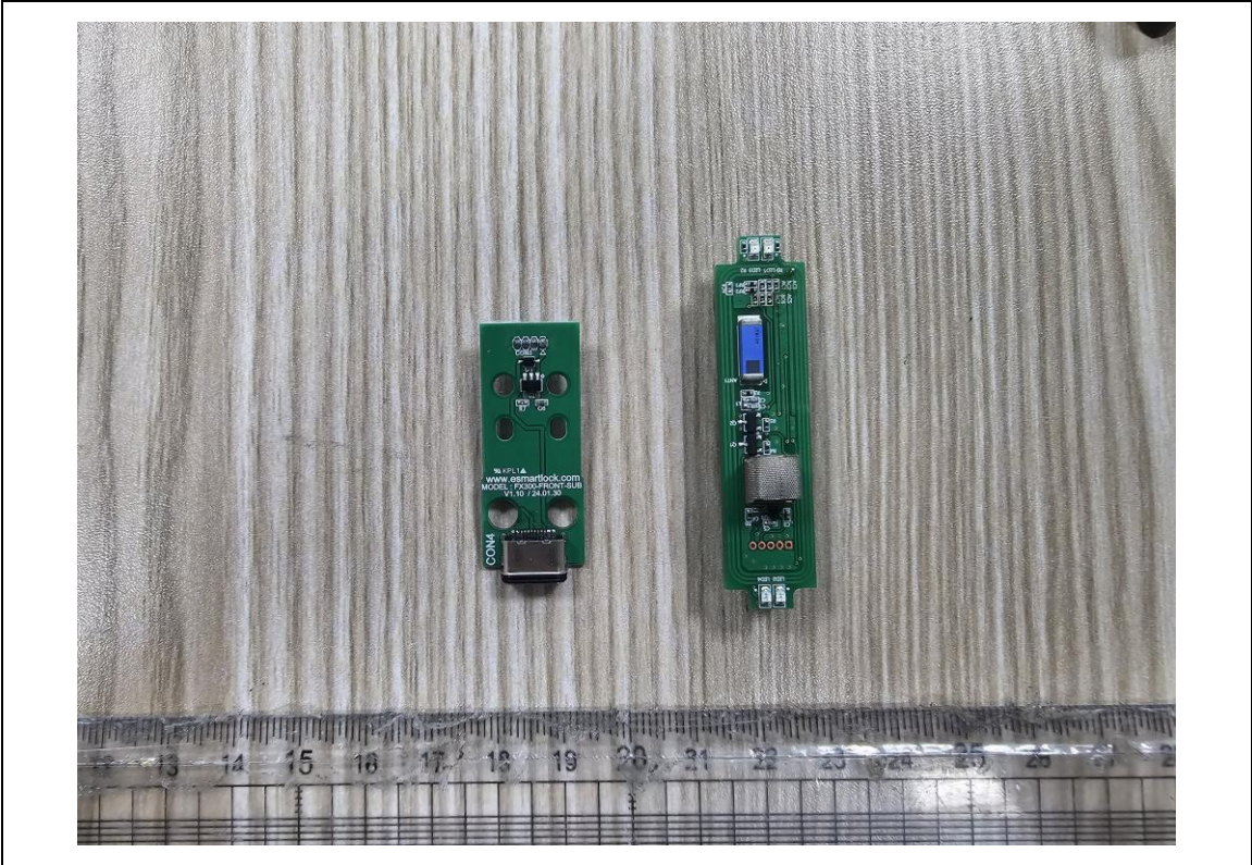
Board 2 Rear
