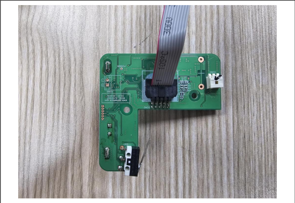
Board 1 Rear
