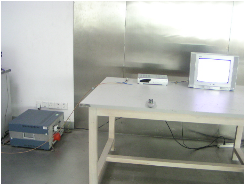
Output Signal Conducted Level -Front View
