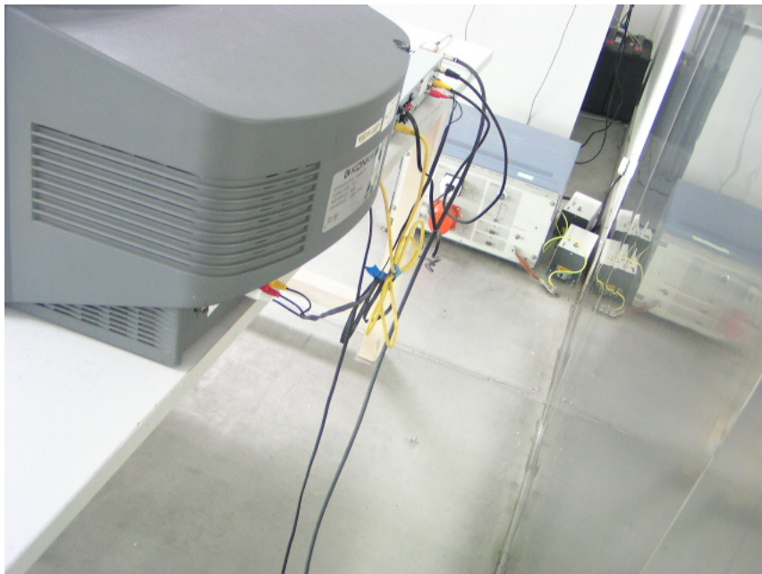
Antenna Conducted Power-Rear View
