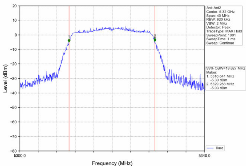
802.11ac(VHT20)_HCH_5320MHz_Ant2_NTNV
