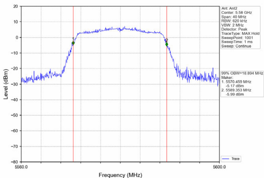
802.11ac(VHT20)_MCH_5580MHz_Ant2_NTNV
