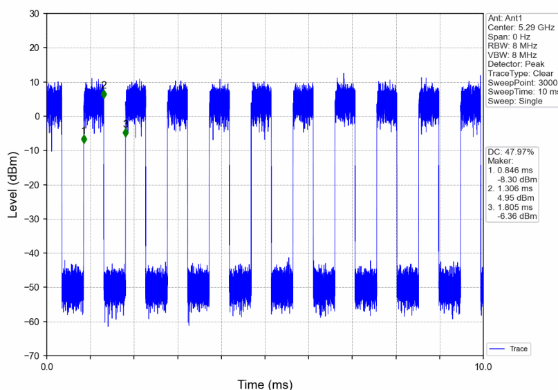
802.11ac(VHT80)_MCH_5290MHz_Ant1_NTNV
