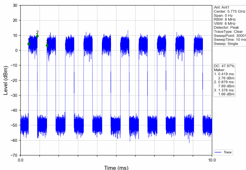
802.11ac(VHT80)_MCH_5775MHz_Ant1_NTNV
