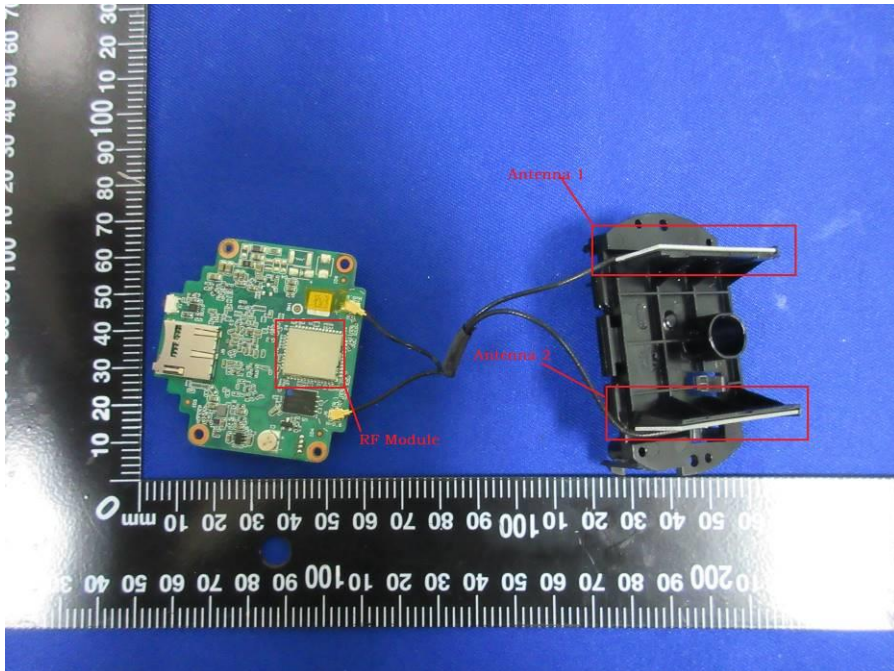
Antenna location and RF Module location
