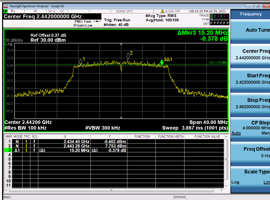
11N20SISO_Ant1_2442
