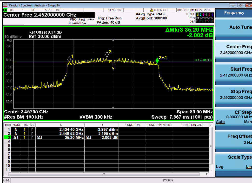
11N40SISO_Ant1_2452
