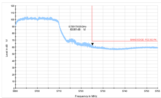
802.11ax HE20-Channel 140: Peak
