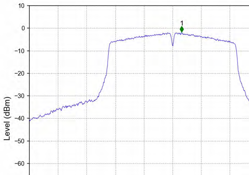
802.11ac(VHT20)_LCH_5745MHz_MIMO_NTNV
