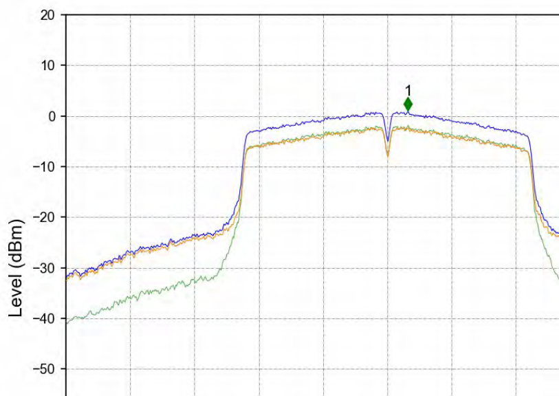
802.11ac(VHT20)_LCH_5745MHz_MIMO_NTNV
