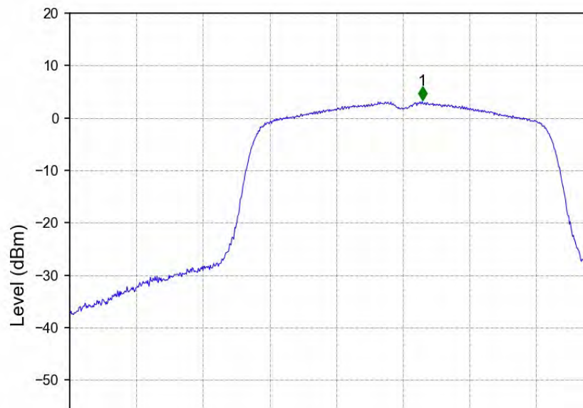
802.11ac(VHT20)_HCH_5700MHz_Ant2_NTNV
