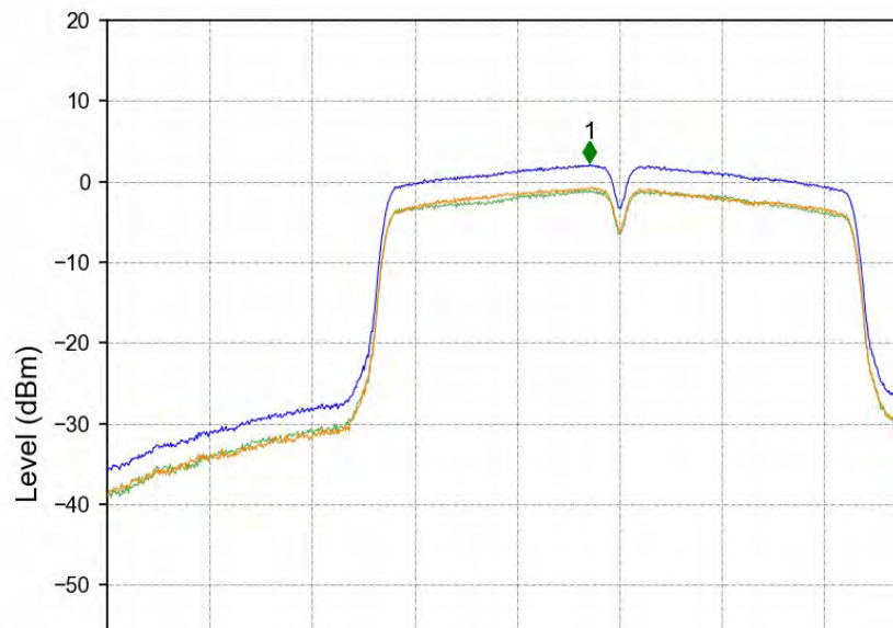
802.11ac(VHT40)_LCH_5190MHz_MIMO_NTNV
