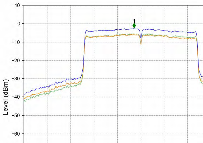
802.11ac(VHT80)_MCH_5290MHz_MIMO_NTNV
