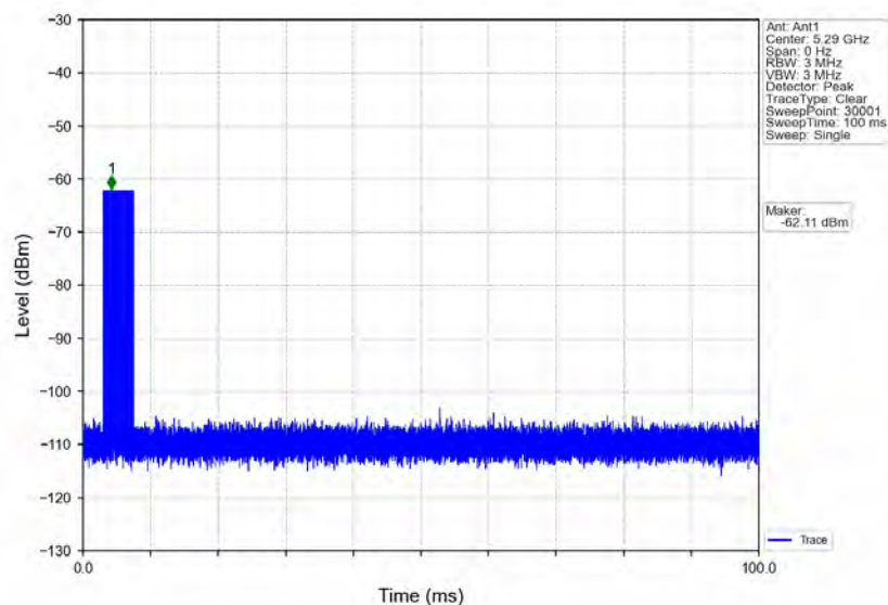
Signal Calibration_802.11ac(VHT80)_2A_5290MHz_RadarType3_Trial0
