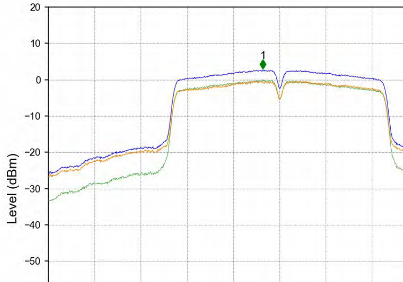
802.11ac(VHT40)_HCH_5670MHz_Ant1_NTNV
