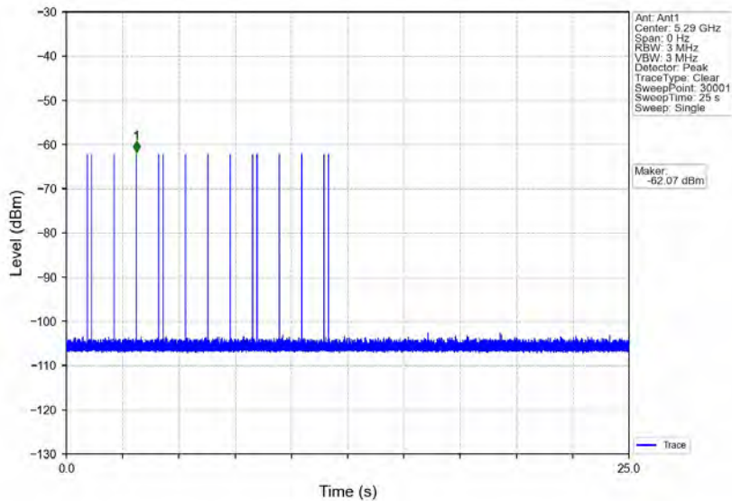
Signal Calibration_802.11ac(VHT80)_2A_5290MHz_RadarType6_Trial0
