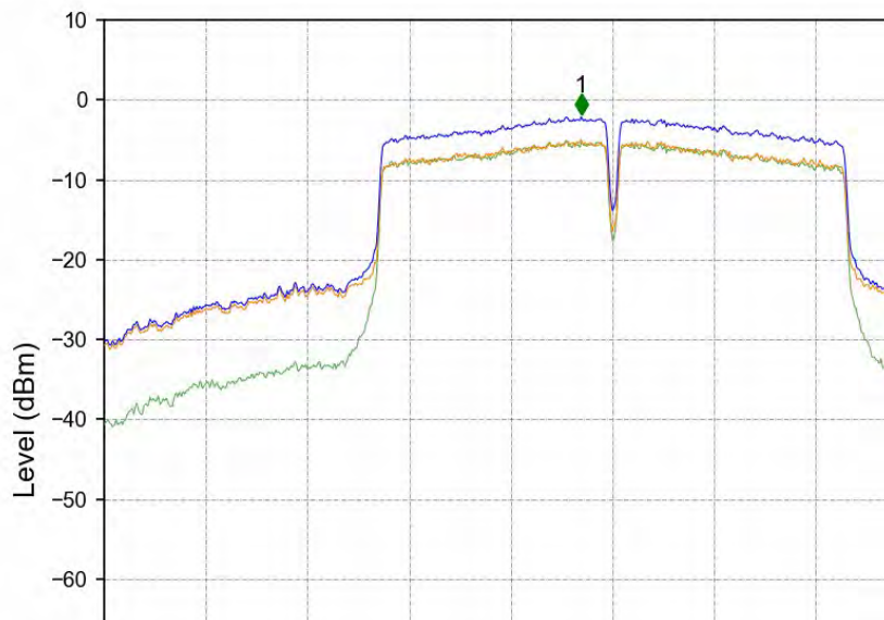
802.11ac(VHT40)_HCH_5795MHz_Ant1_NTNV
