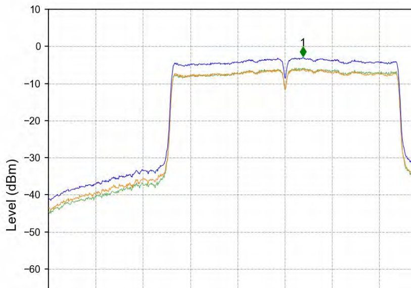
802.11ac(VHT80)_MCH_5290MHz_Ant1_NTNV
