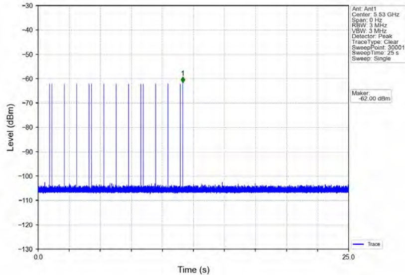
Signal Calibration_802.11ac(VHT80)_2C_5530MHz_RadarType6_Trial0
