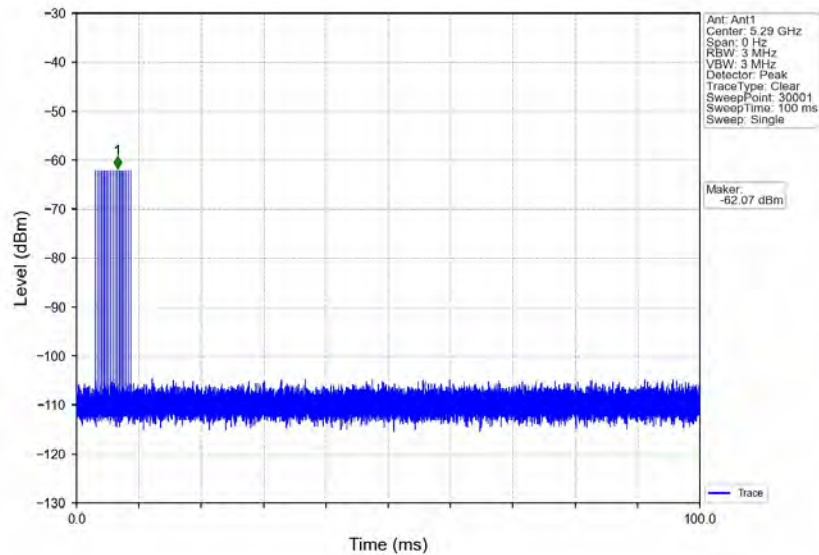
Signal Calibration_802.11ac(VHT80)_2A_5290MHz_RadarType4_Trial0
