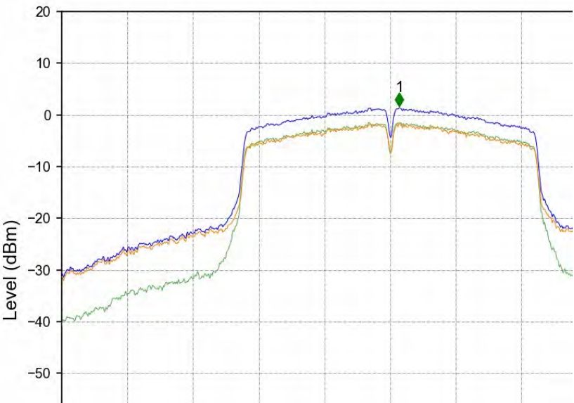
802.11ac(VHT20)_HCH_5825MHz_Ant1_NTNV
