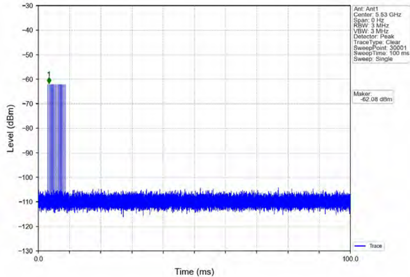
Signal Calibration_802.11ac(VHT80)_2C_5530MHz_RadarType4_Trial0
