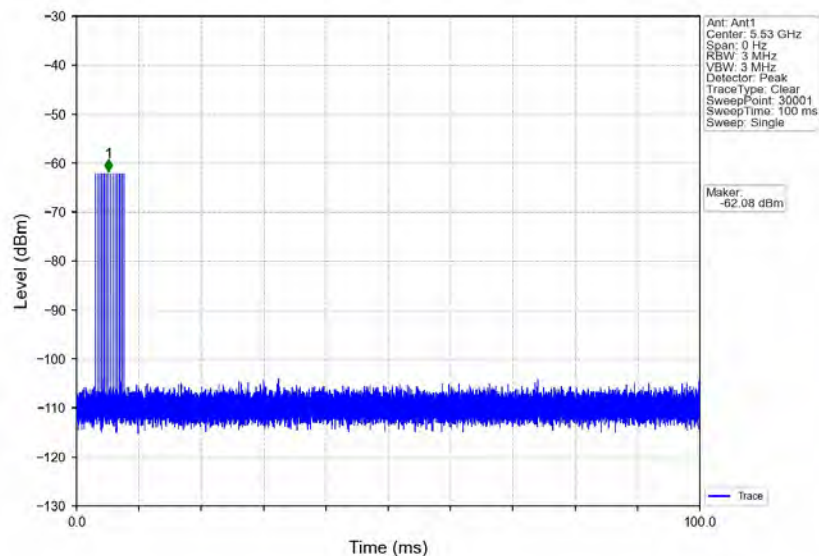
Signal Calibration_802.11ac(VHT80)_2C_5530MHz_RadarType5_Trial0
