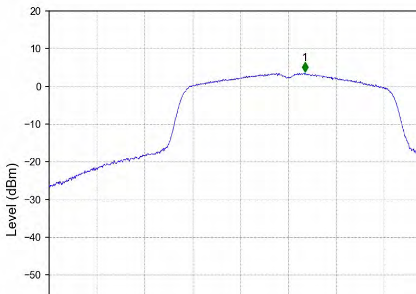
802.11ac(VHT20)_MCH_5580MHz_Ant1_NTNV
