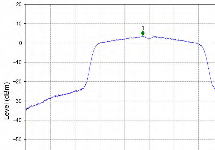
802.11ac(VHT20)_MCH_5580MHz_MIMO_NTNV
