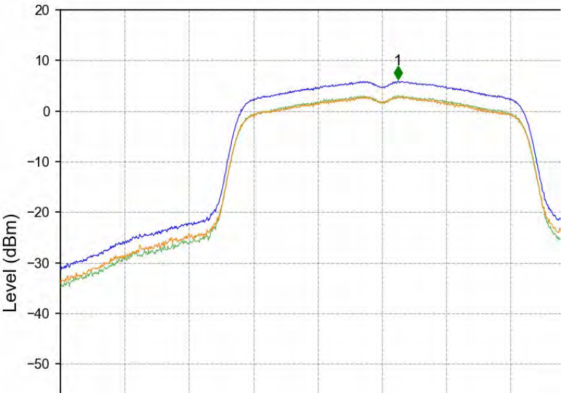
802.11ac(VHT20)_LCH_5260MHz_Ant1_NTNV
