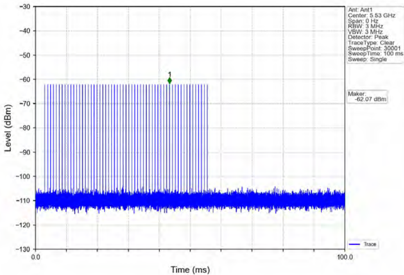
Signal Calibration_802.11ac(VHT80)_2C_5530MHz_RadarType2_Trial0
