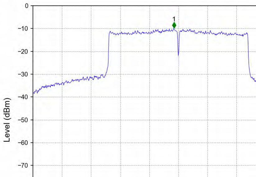
802.11ac(VHT80)_MCH_5775MHz_Ant2_NTNV
