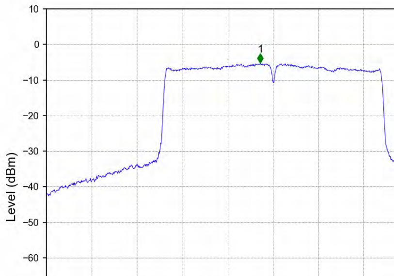
802.11ac(VHT80)_MCH_5290MHz_MIMO_NTNV
