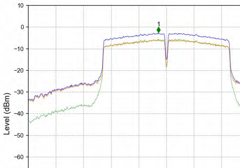
802.11ac(VHT20)_LCH_5745MHz_Ant1_NTNV
