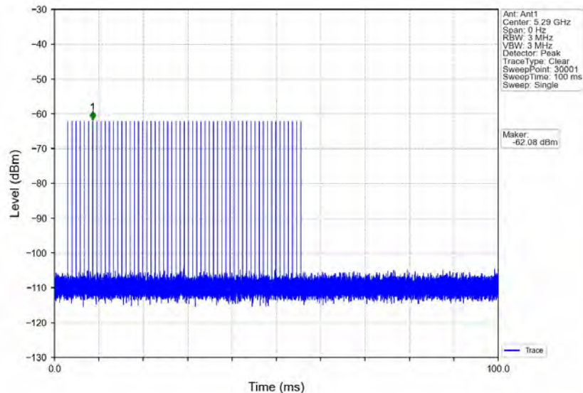
Signal Calibration_802.11ac(VHT80)_2A_5290MHz_RadarType2_Trial0
