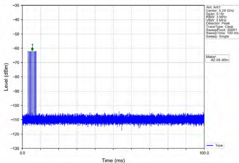
Signal Calibration_802.11ac(VHT80)_2A_5290MHz_RadarType5_Trial0
