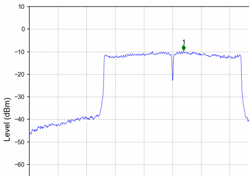
802.11ac(VHT80)_MCH_5775MHz_Ant2_NTNV
