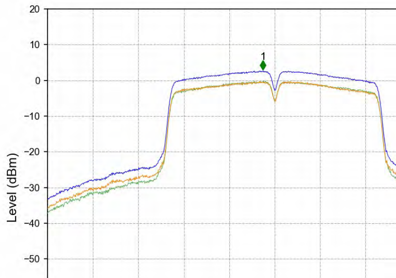
802.11ac(VHT40)_LCH_5270MHz_MIMO_NTNV
