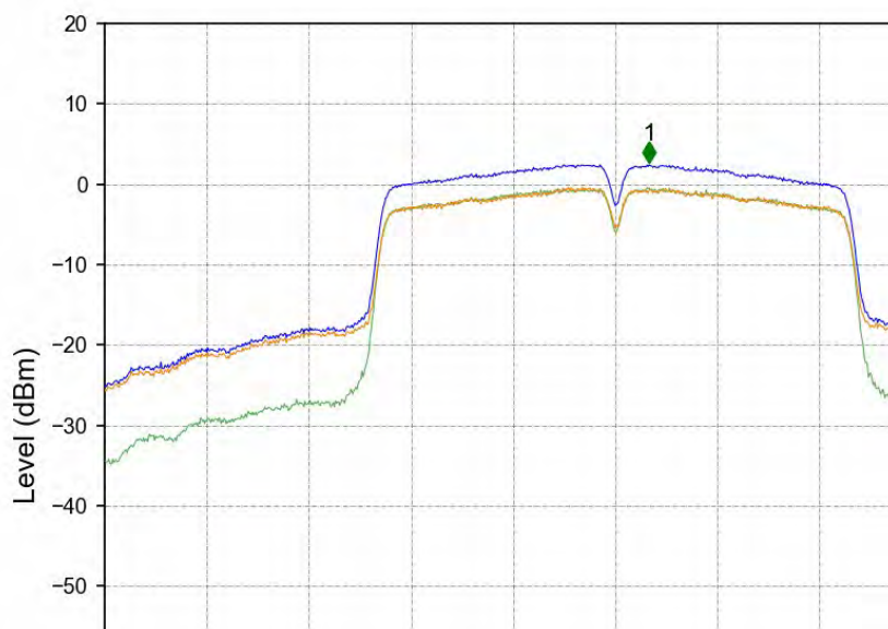
802.11n(HT40)_HCH_5670MHz_MIMO_NTNV
