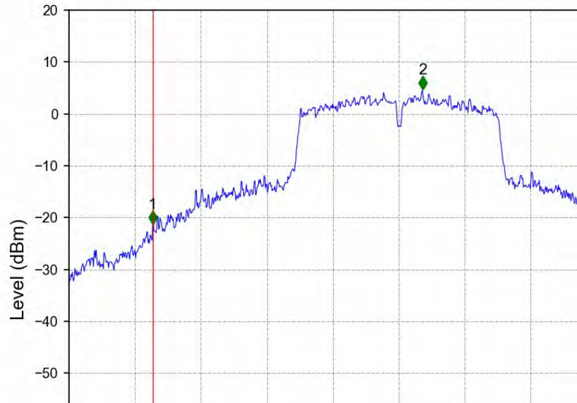
802.11ac(VHT40)_HCH_5670MHz_Ant2_NTNV
