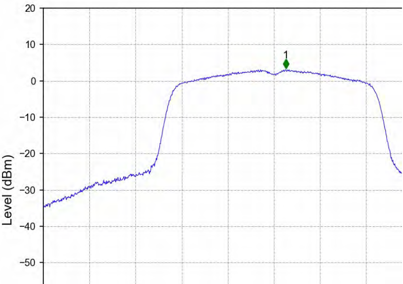
802.11ac(VHT20)_HCH_5240MHz_Ant2_NTNV
