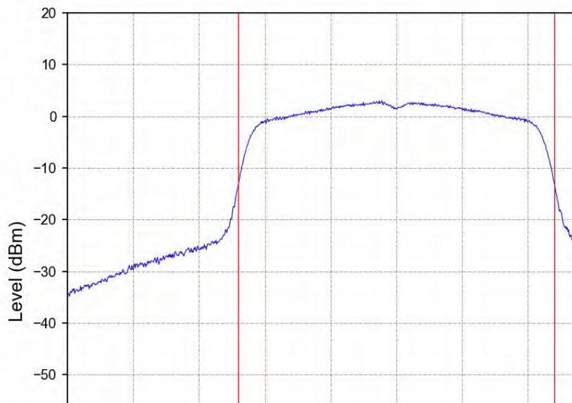
802.11n(HT20)_HCH_5240MHz_Ant2_NTNV
