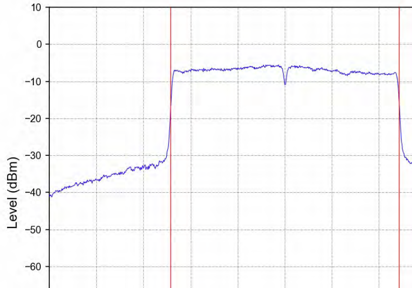
802.11ac(VHT80)_MCH_5290MHz_Ant2_NTNV
