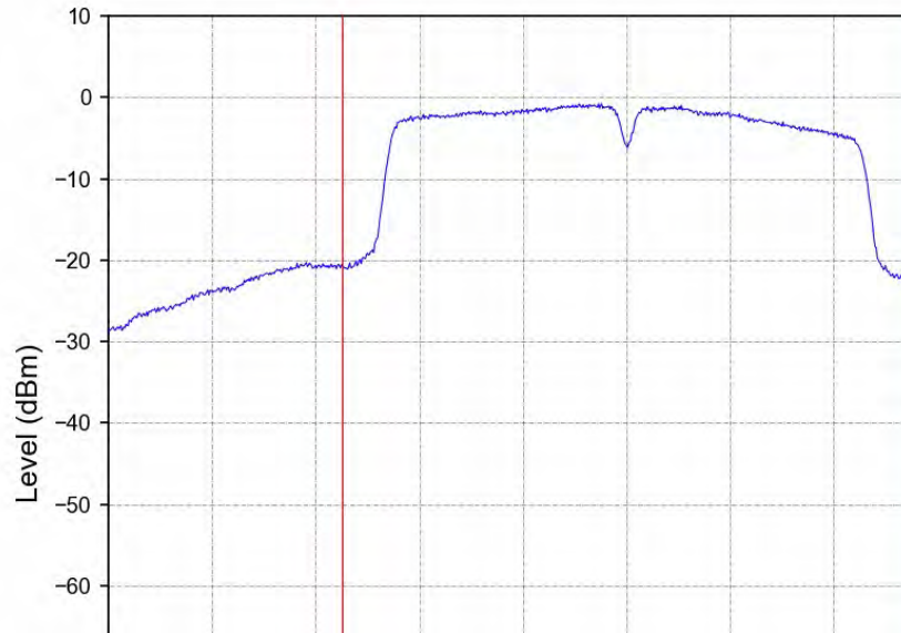
802.11ac(VHT40)_LCH_5510MHz_Ant2_NTNV
