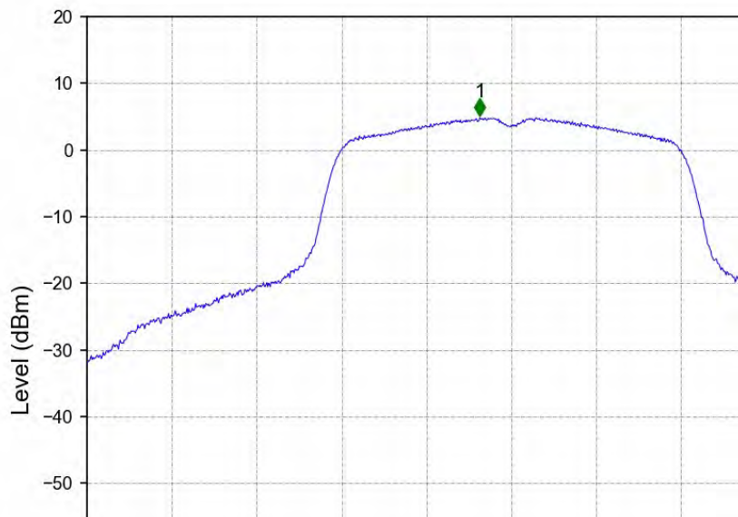
802.11a_LCH_5260MHz_Ant2_NTNV
