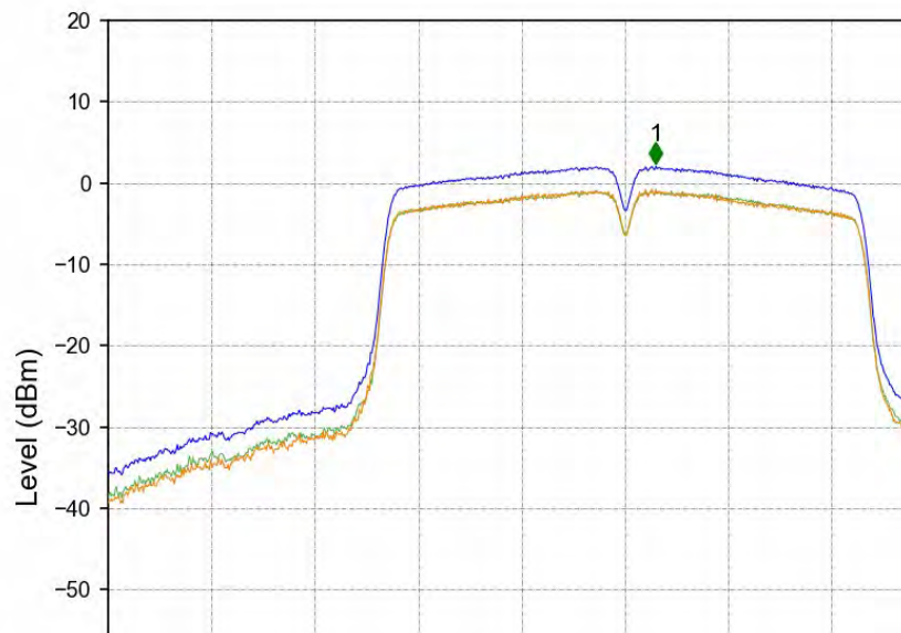
802.11n(HT40)_LCH_5190MHz_MIMO_NTNV
