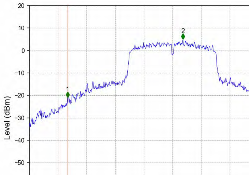
802.11ac(VHT40)_MCH_5550MHz_Ant2_NTNV
