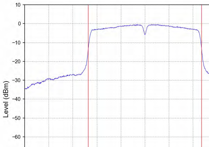
802.11n(HT40)_HCH_5670MHz_Ant2_NTNV
