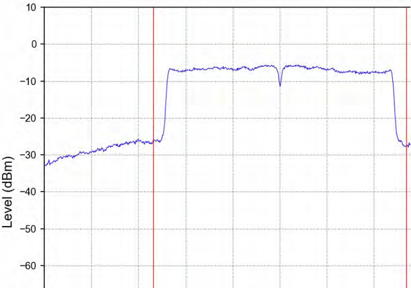
802.11ac(VHT80)_MCH_5775MHz_Ant2_NTNV
