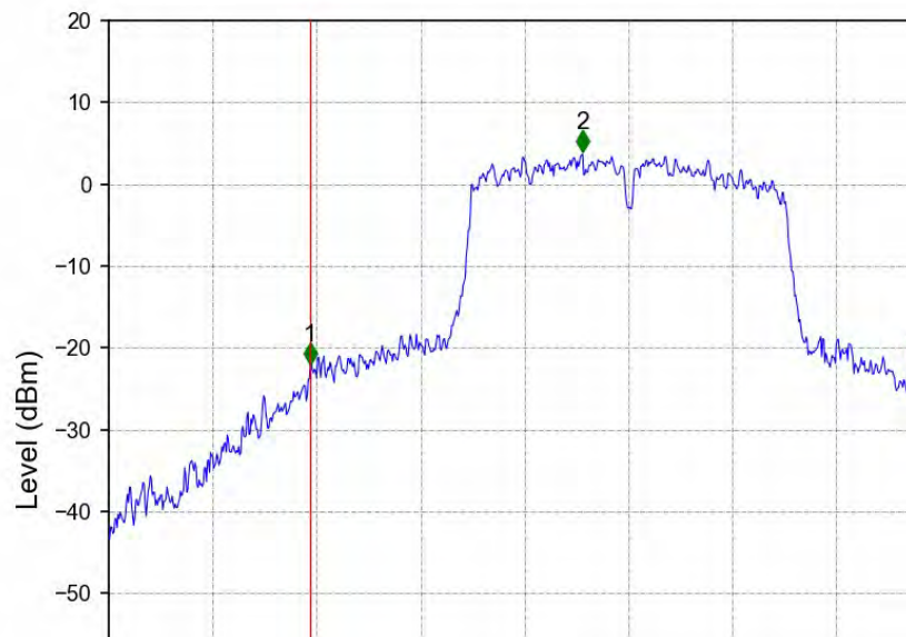
802.11ac(VHT40)_LCH_5510MHz_Ant2_NTNV
