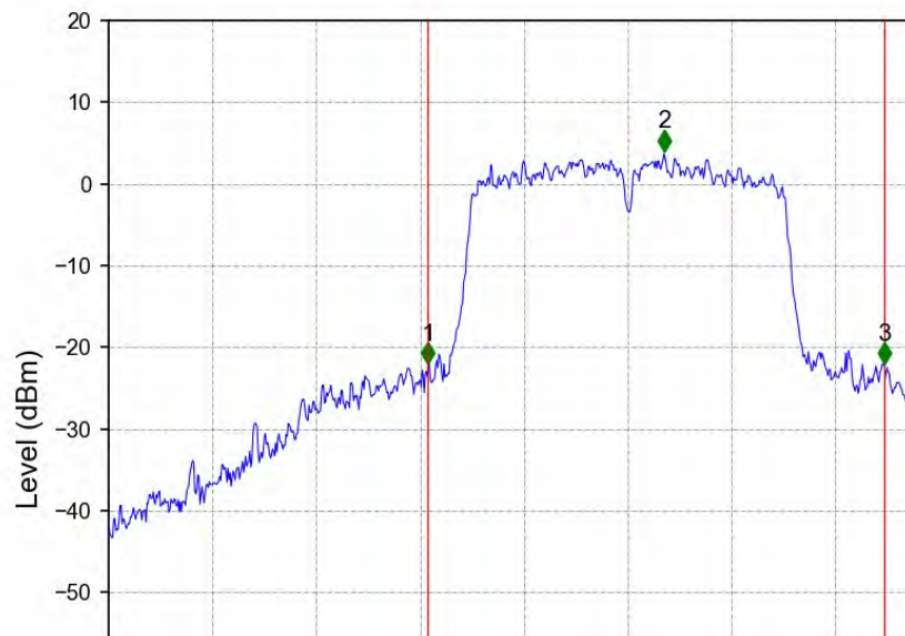
802.11ac(VHT40)_LCH_5190MHz_Ant2_NTNV
