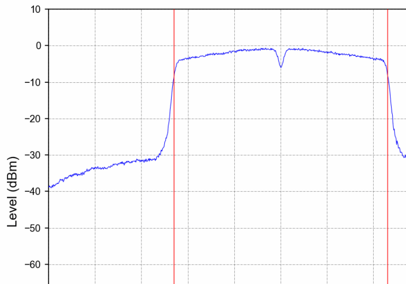
802.11ac(VHT40)_HCH_5795MHz_Ant2_NTNV
