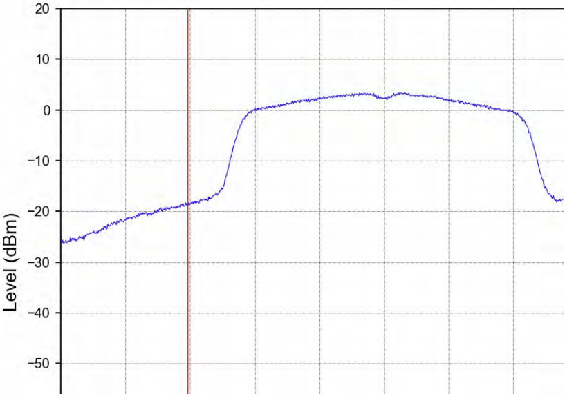
802.11ac(VHT20)_MCH_5580MHz_Ant2_NTNV
