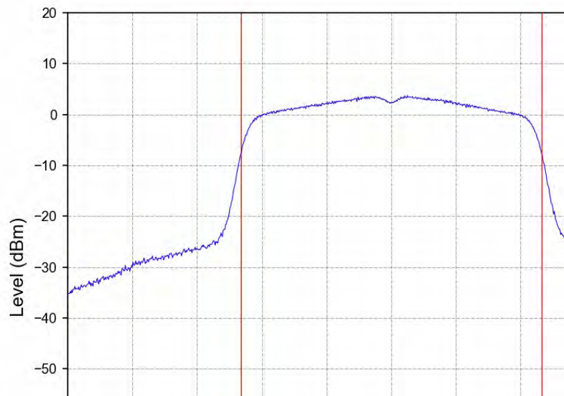
802.11ac(VHT20)_MCH_5785MHz_Ant2_NTNV
