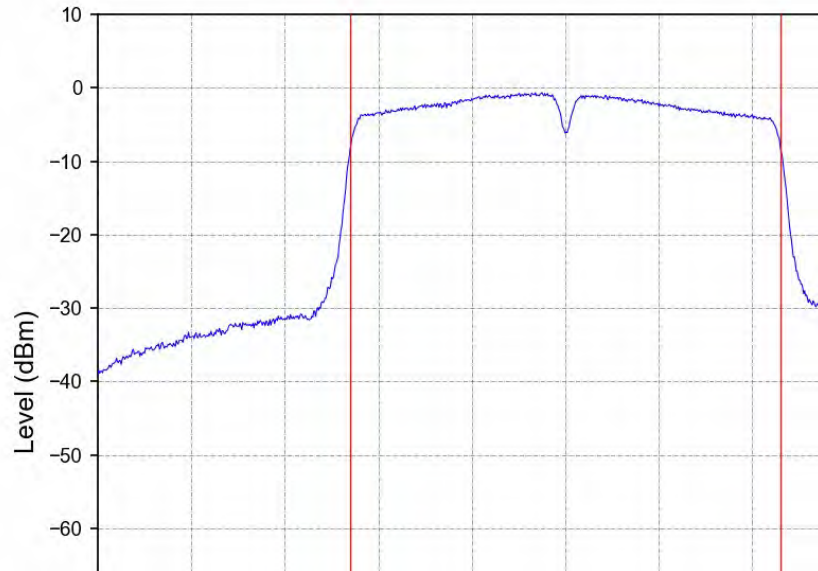
802.11ac(VHT40)_LCH_5190MHz_Ant2_NTNV
