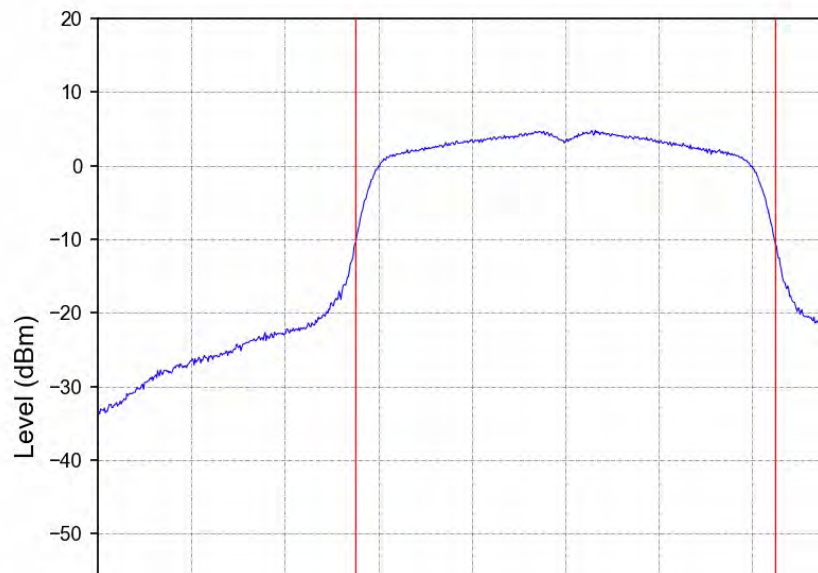
802.11a_LCH_5260MHz_Ant2_NTNV
