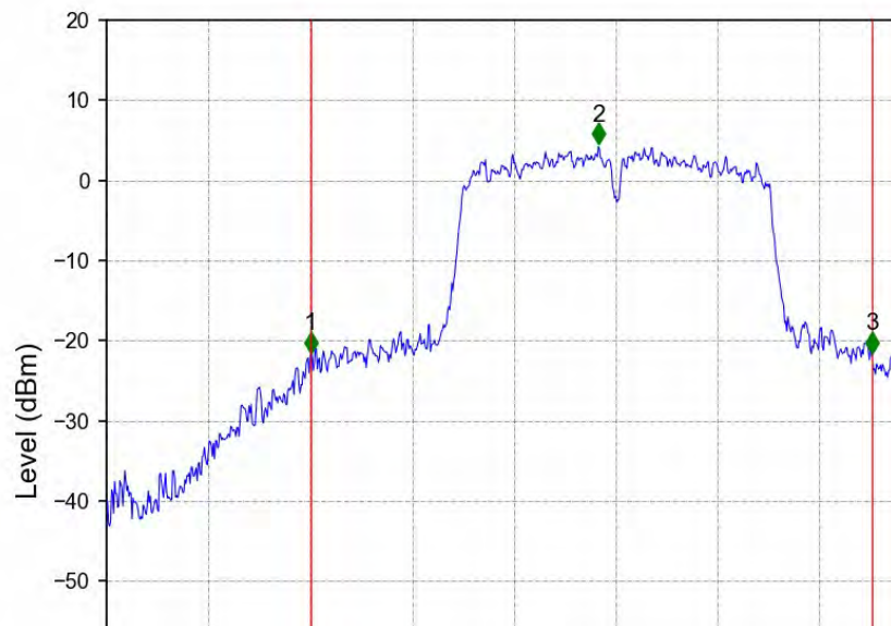
802.11ac(VHT40)_HCH_5670MHz_Ant2_NTNV
