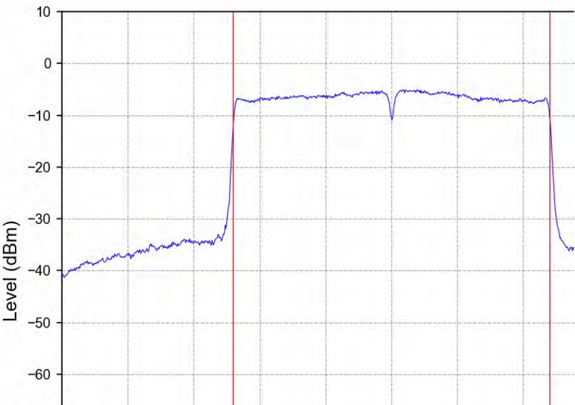
802.11ac(VHT80)_MCH_5775MHz_Ant2_NTNV
