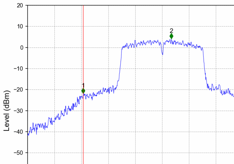
802.11ac(VHT40)_HCH_5310MHz_Ant2_NTNV
