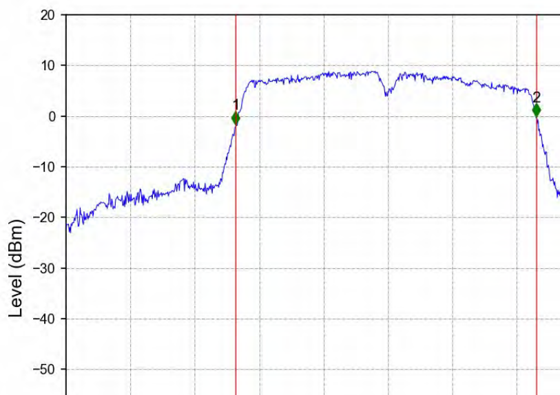
802.11ac(VHT40)_LCH_5510MHz_Ant2_NTNV
