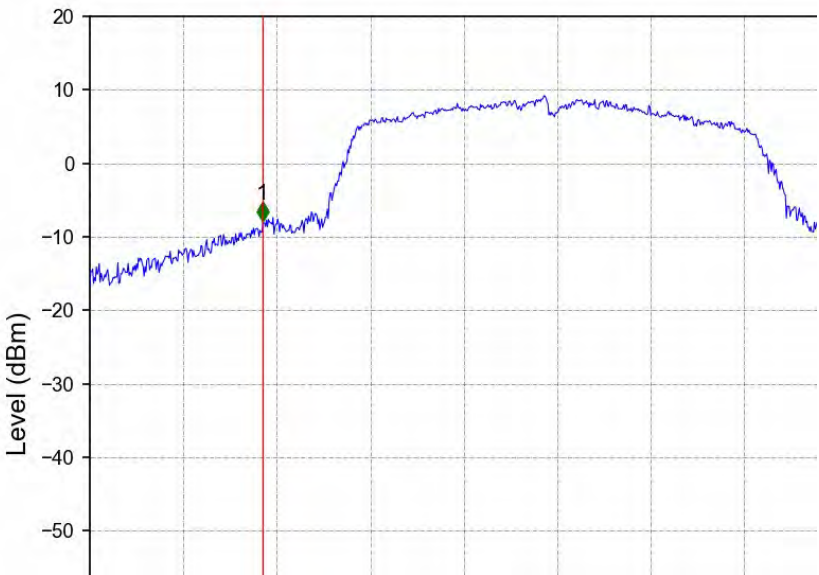
802.11ac(VHT20)_LCH_5500MHz_Ant2_NTNV
