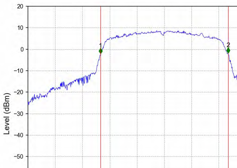
802.11n(HT20)_MCH_5785MHz_Ant2_NTNV
