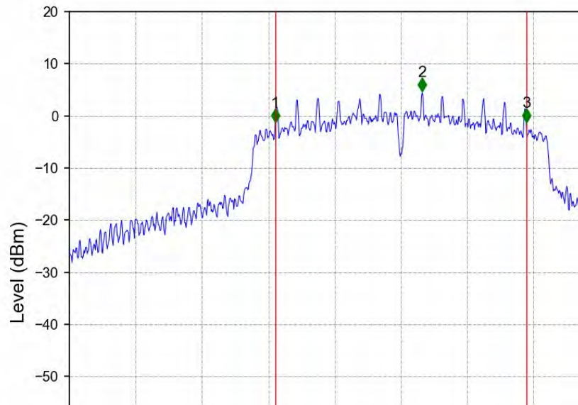
802.11n(HT20)_MCH_5785MHz_Ant2_NTNV
