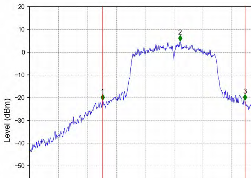
802.11ac(VHT20)_HCH_5320MHz_Ant2_NTNV
