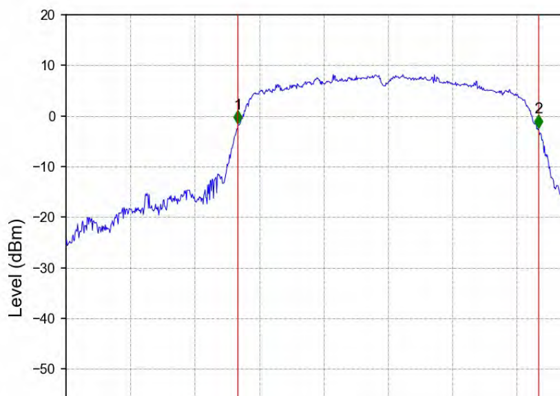
802.11ac(VHT20)_LCH_5745MHz_Ant2_NTNV
