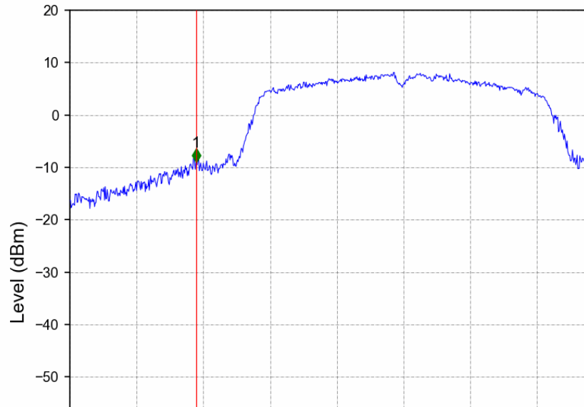
802.11n(HT20)_LCH_5745MHz_Ant2_NTNV
