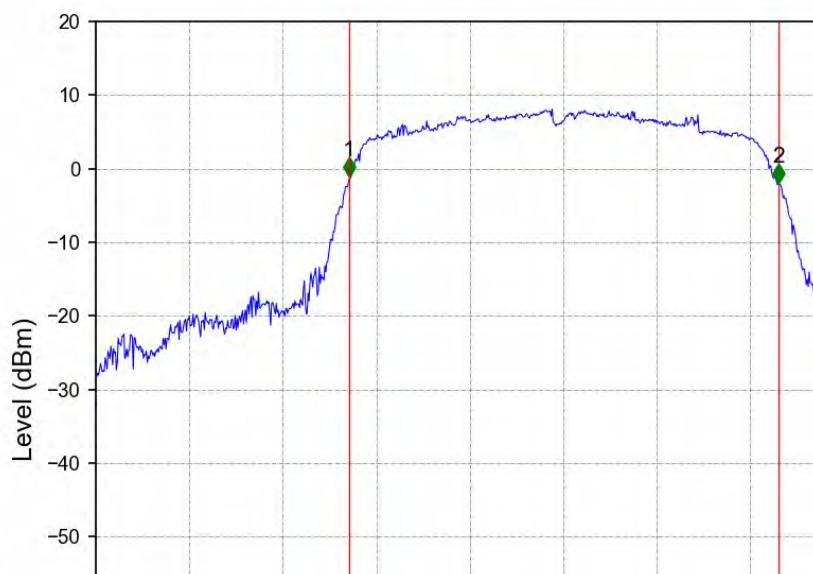
802.11ac(VHT20)_HCH_5825MHz_Ant2_NTNV
