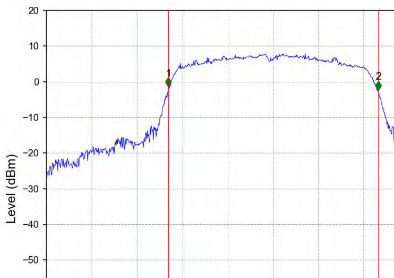
802.11ac(VHT20)_LCH_5180MHz_Ant2_NTNV
