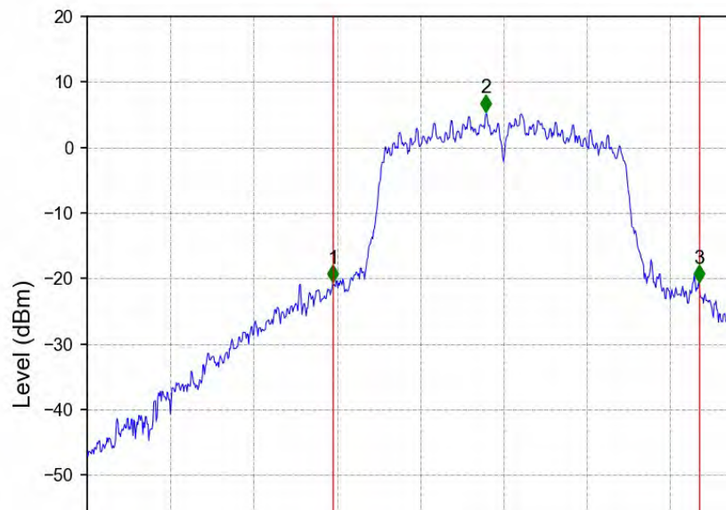
802.11n(HT20)_MCH_5580MHz_Ant2_NTNV
