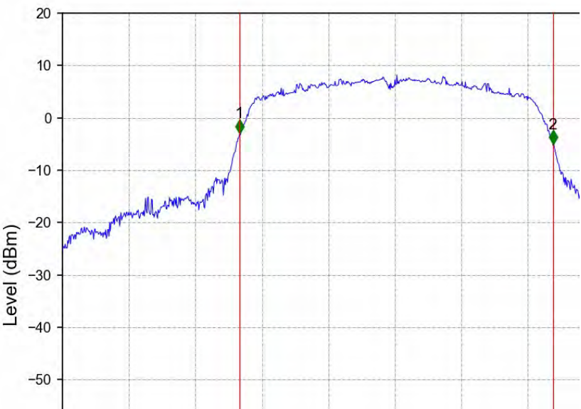
802.11ac(VHT20)_MCH_5200MHz_Ant2_NTNV
