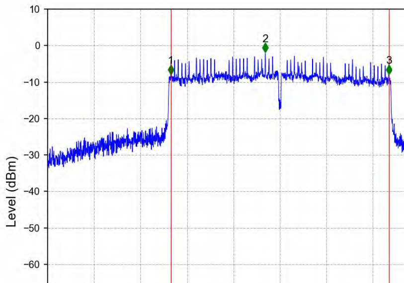
802.11ac(VHT80)_MCH_5775MHz_Ant2_NTNV
