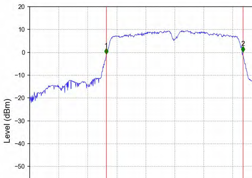
802.11n(HT40)_HCH_5670MHz_Ant2_NTNV
