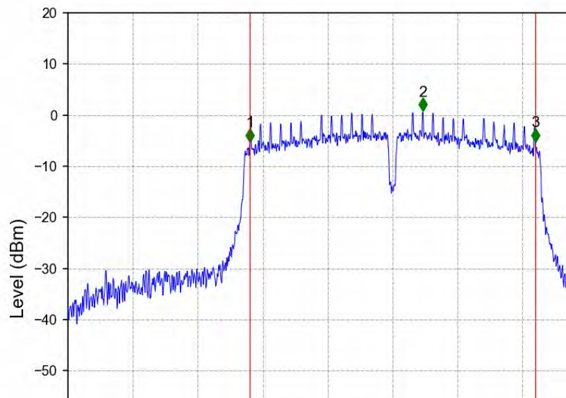
802.11ac(VHT40)_HCH_5795MHz_Ant2_NTNV
