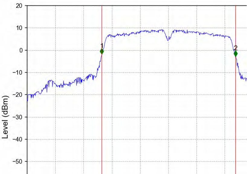
802.11n(HT40)_HCH_5310MHz_Ant2_NTNV
