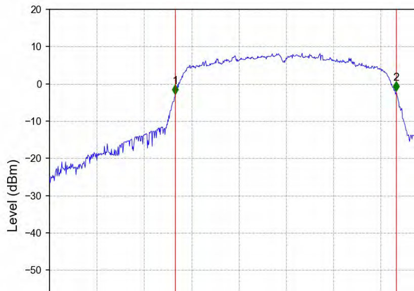
802.11n(HT20)_LCH_5745MHz_Ant2_NTNV
