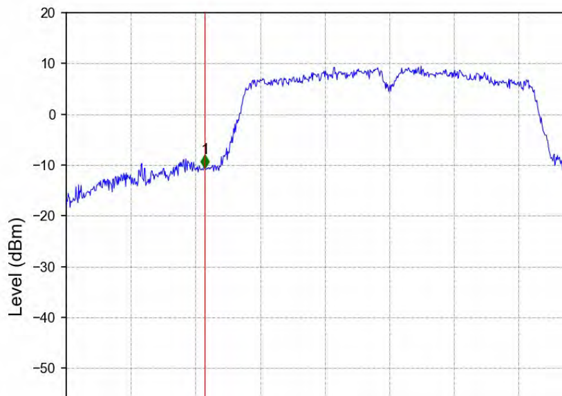
802.11ac(VHT40)_HCH_5795MHz_Ant2_NTNV
