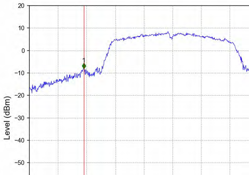
802.11ac(VHT20)_LCH_5745MHz_Ant2_NTNV
