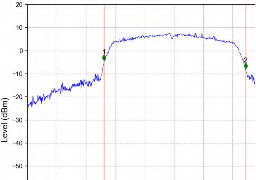
802.11ac(VHT20)_MCH_5300MHz_Ant2_NTNV
