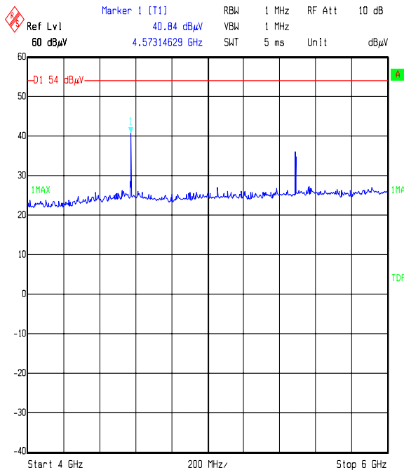
Title: Stewart Golf EUT: Robokaddy, FCC P15.249 Rad Emissions Comment A: 47810JD01 Transmitter Date: 12.MAY 2006 17:43:25
