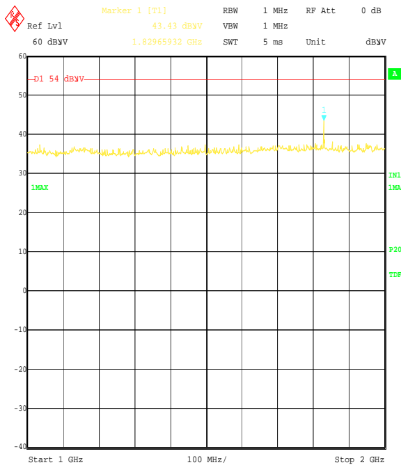
Title: Stewart Golf EUT: Robokaddy, FCC P15.249 Radiated Emissions Comment A: 47810JD01 Tx Mode Date: 21.APR.2006 18:16:55
