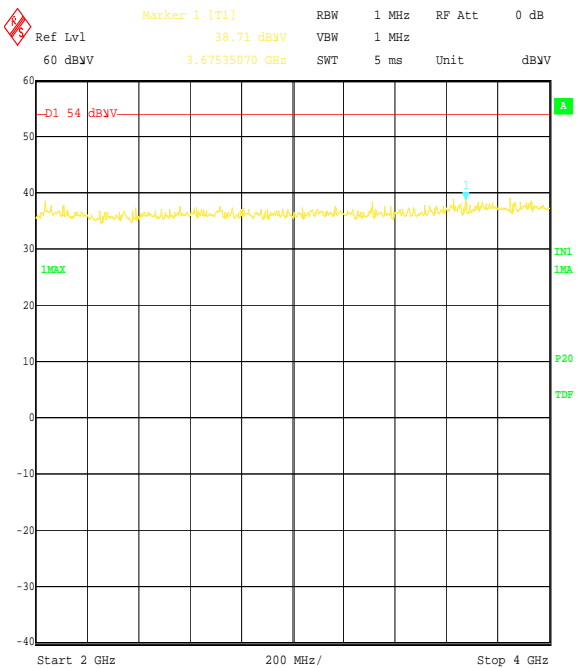
Title: Stewart Golf EUT: Robokaddy, FCC P15.249 Radiated Emissions Comment A: 47810JD01 Tx Mode Date: 21.APR.2006 18:17:40
