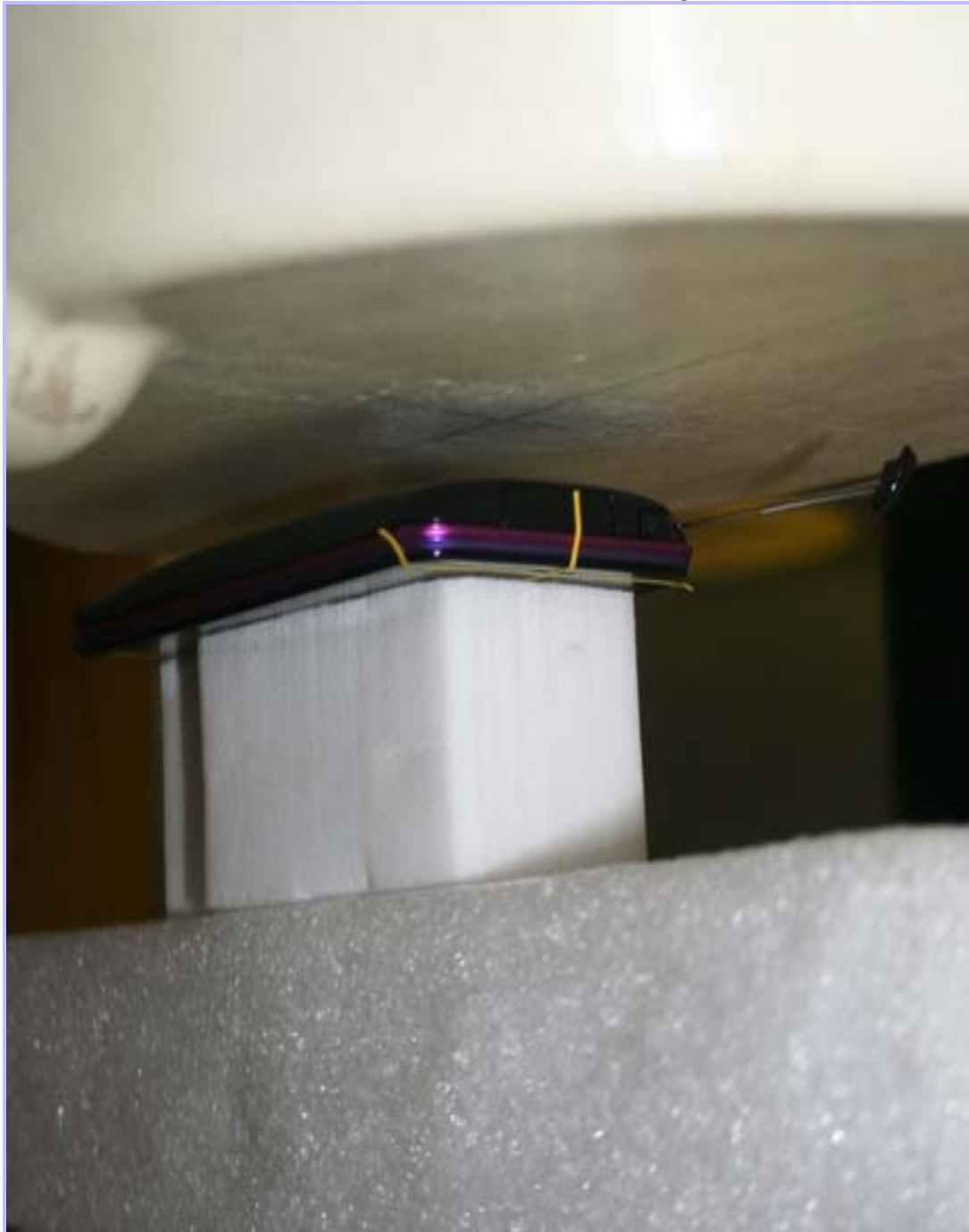
PHT/81533JD05/013: Rear of EUT With Antenna Extended Facing Phantom
