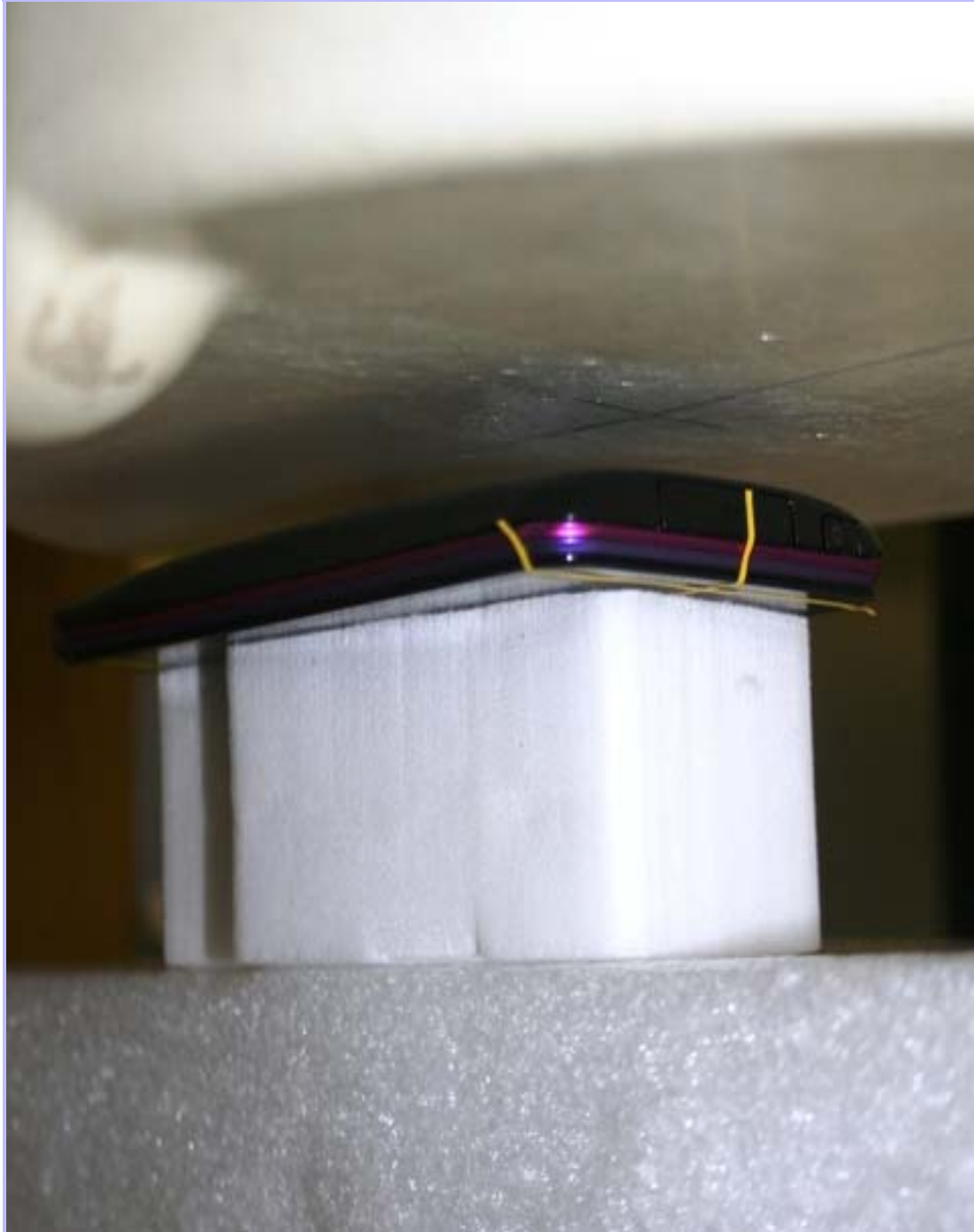
PHT/81533JD05/012: Rear of EUT With Antenna Retracted Facing Phantom
