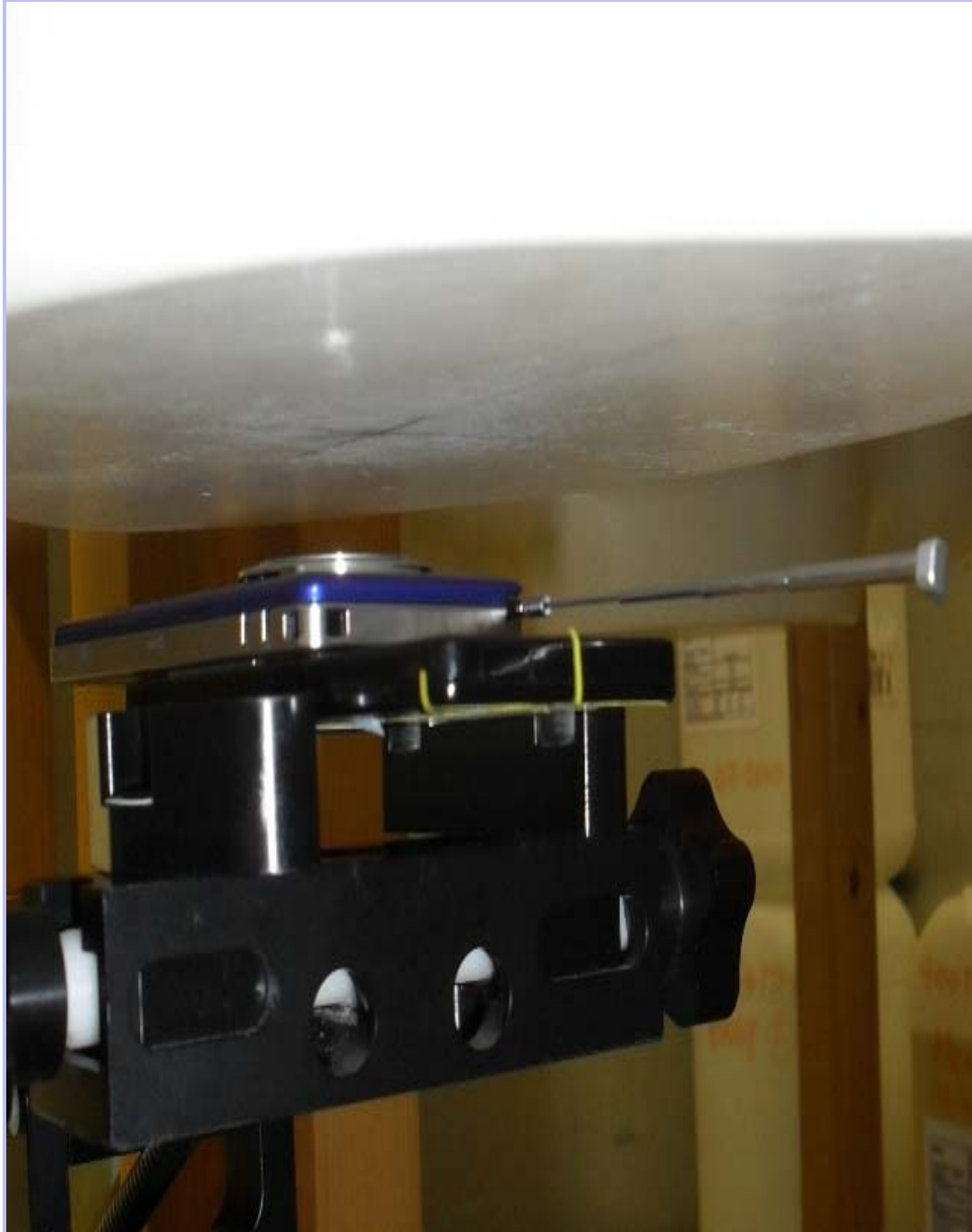
PHT/79566JD17/025: Rear of EUT Facing Phantom With Slide Open Antenna Extended
