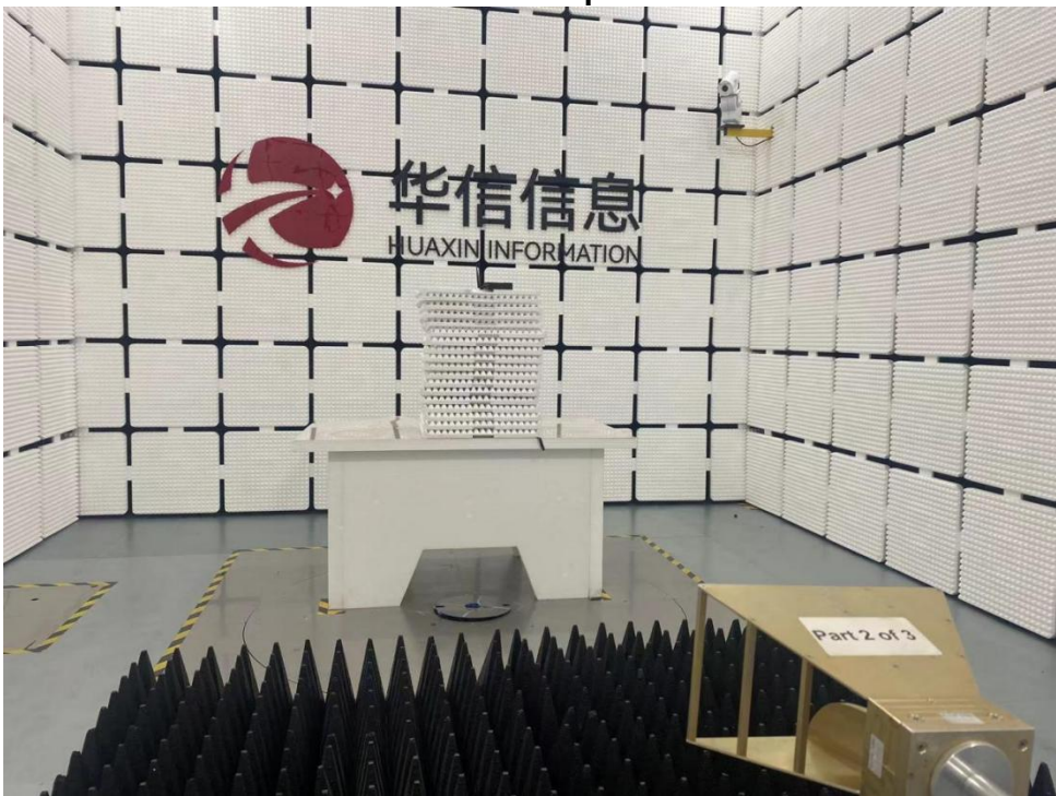
Radiated Emission Test Setup Photo - Above 1GHz
