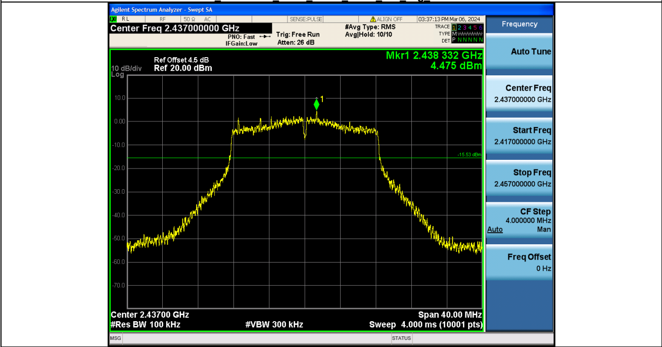
2_Spurious_Emission_NVNT_ANT1_802_11g_2437
