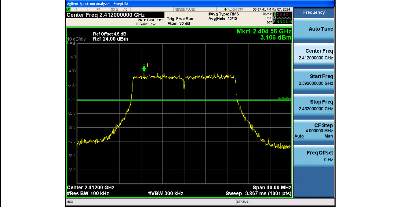
2 Spurious Emission HVNT ANT1 802 11ax(HE20) 2412
