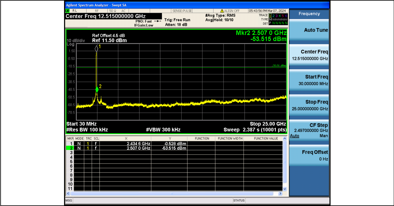
1 Reference Level HVNT ANT1 802 11ax(HE40) 2437
