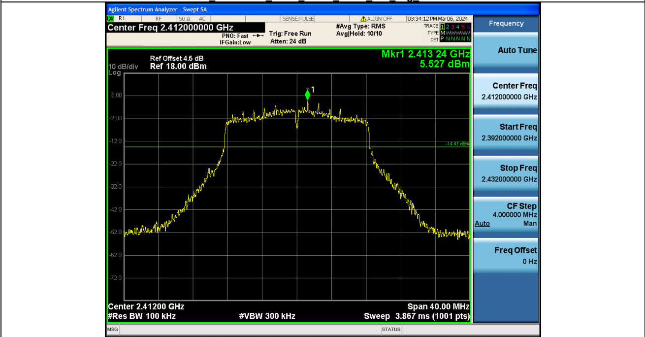
2_Spurious_Emission_NVNT_ANT1_802_11g_2412
