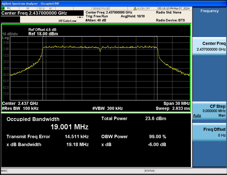
-6dB_Bandwidth_HVNT_ANT1_802_11ax(HE20)_2437
