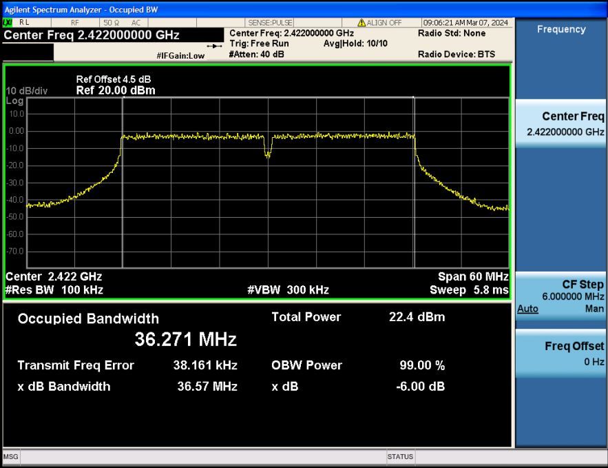
-6dB_Bandwidth_HVNT_ANT1_802_11n(HT40)_2422
