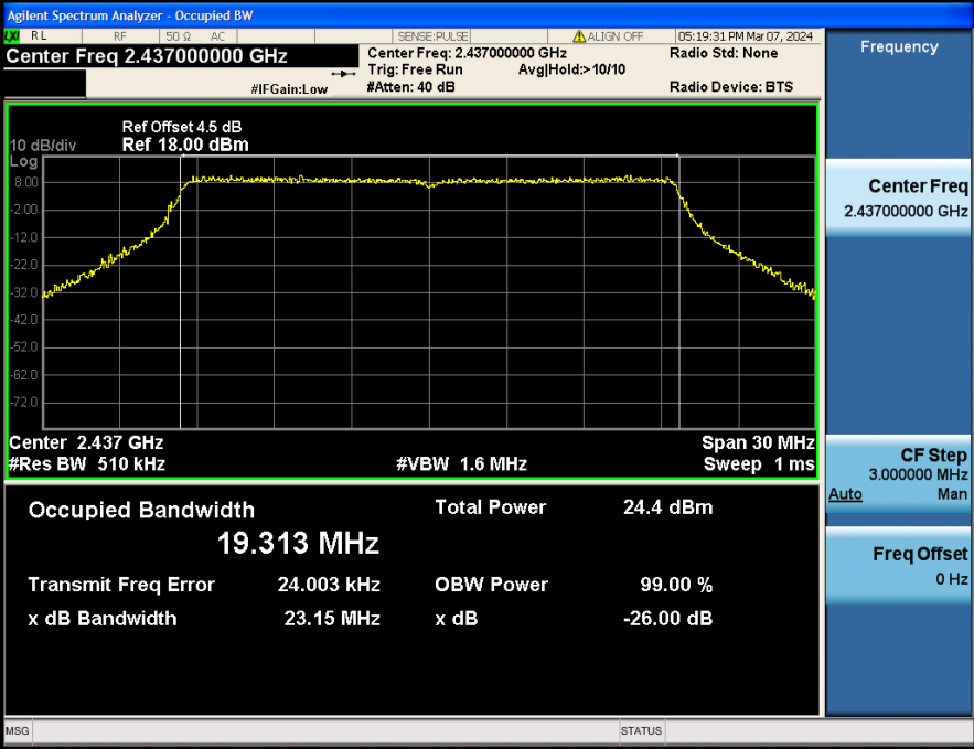
99%_Occupied_Bandwidth_HVNT_ANT1_802_11ax(HE20)_2437
