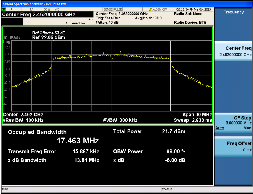
-6dB_Bandwidth_NVNT_ANT1_802_11n(HT20)_2462
