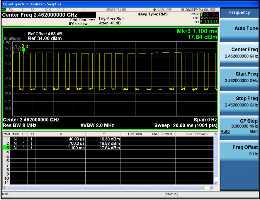
Duty Cycle NVNT_ANT1_802_11b_2462
