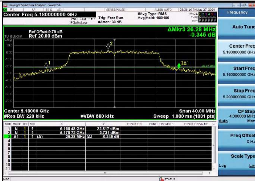
11AX20SISO-Ant2-5180
