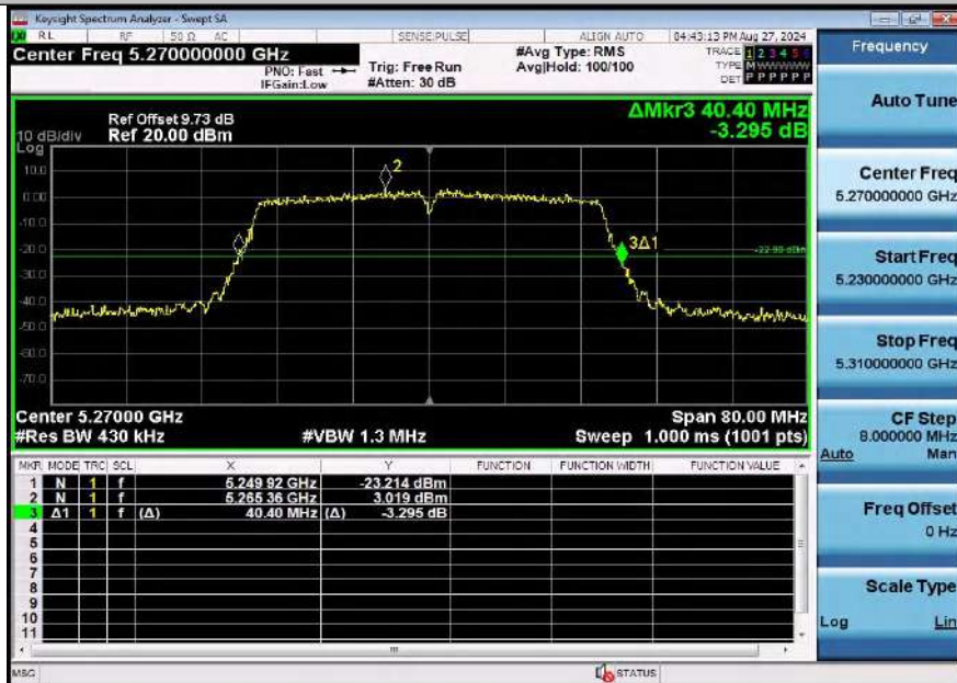
11AC40SISO-Ant2-5270
