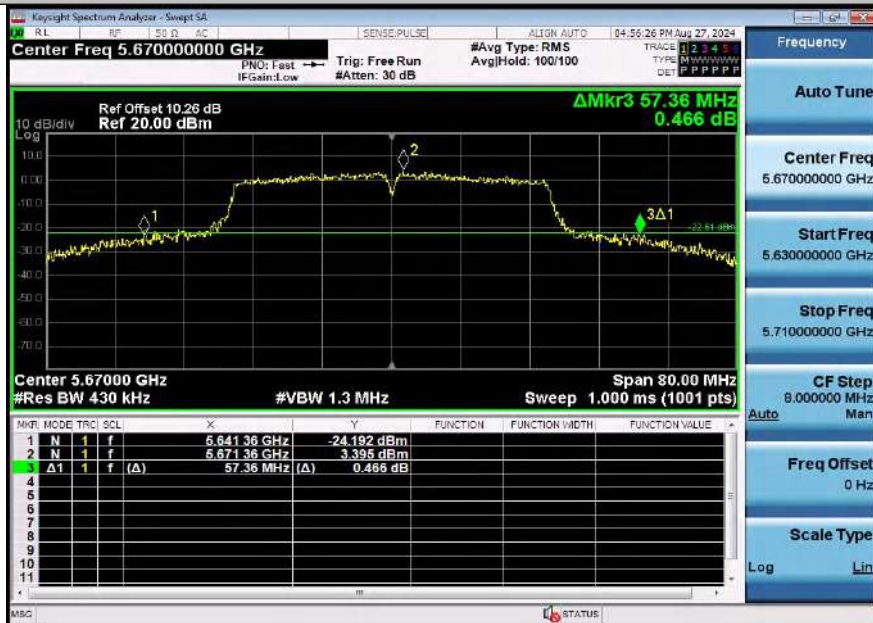
11AC40SISO-Ant2-5670
