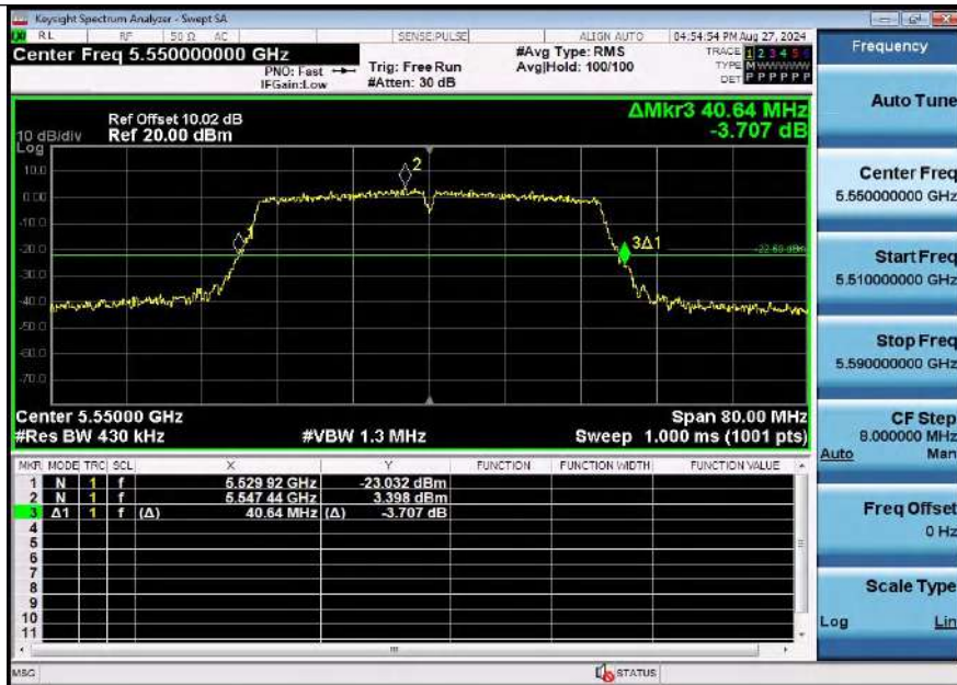
11AC40SISO-Ant2-5550
