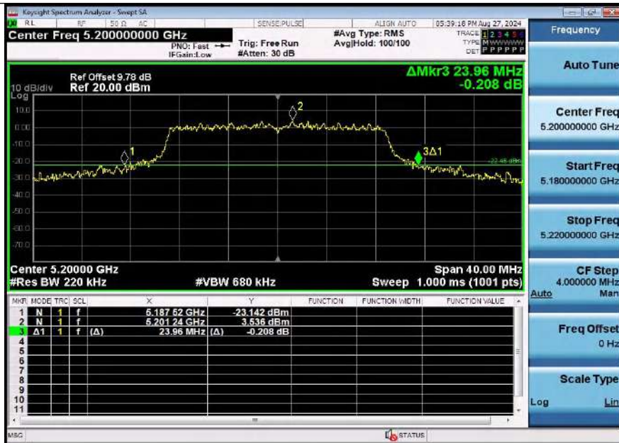
11AX20SISO-Ant2-5200
