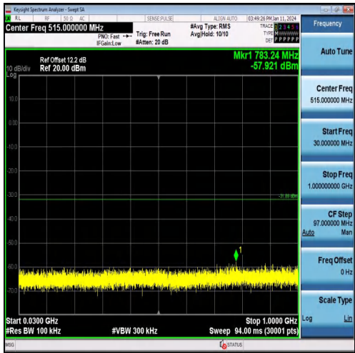
30MHz-1GHz
