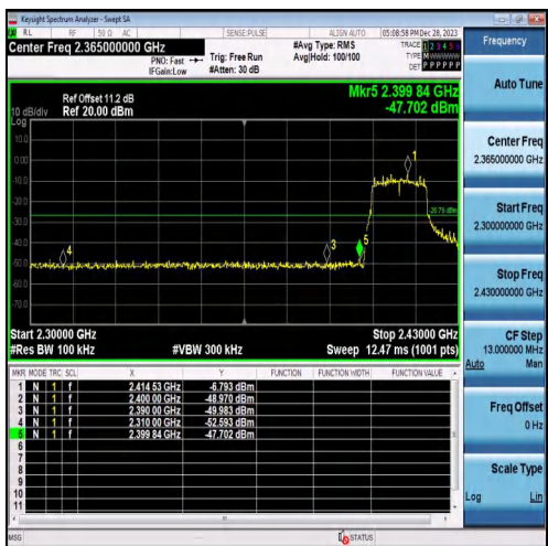
Left bandedge
