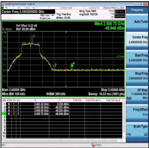
Right bandedge
