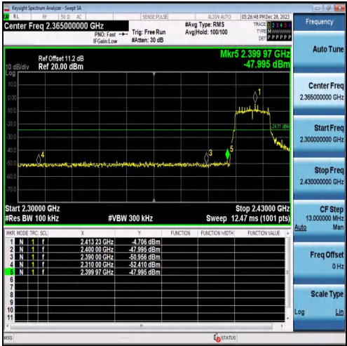
Left bandedge
