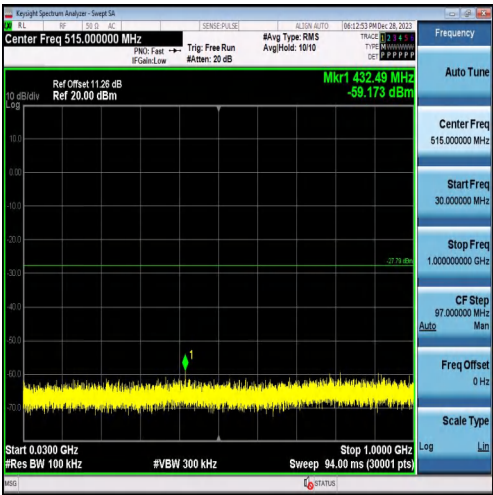
30MHz-1GHz
