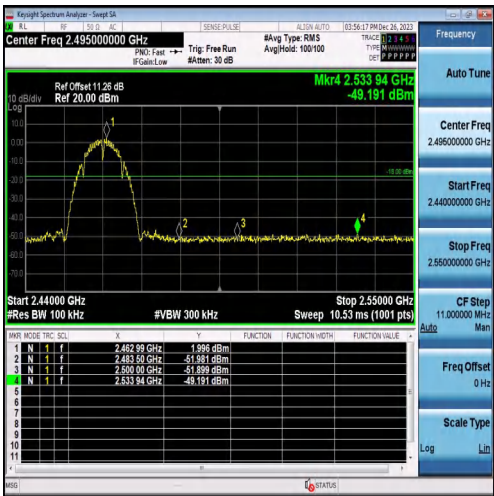
Right bandedge
