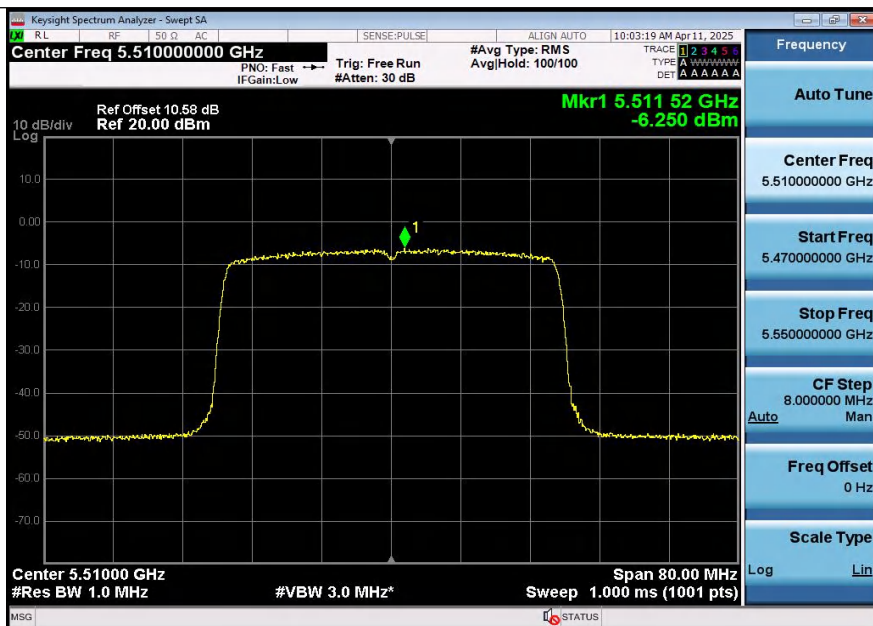
11AX40SISO-Ant2-5510-PASS
