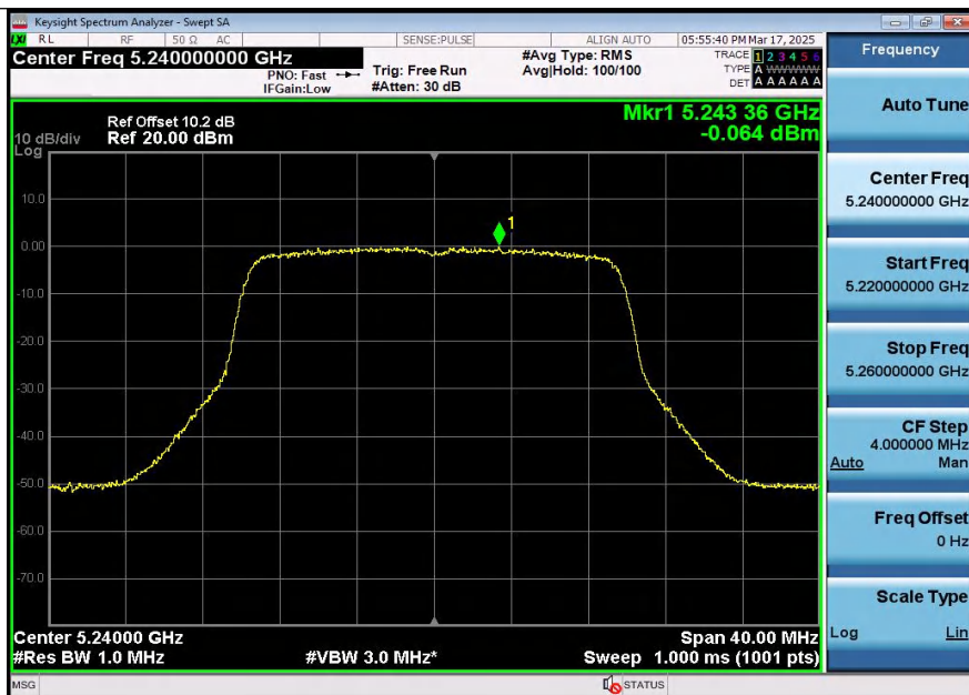
11AX20SISO-Ant1-5240-PASS
