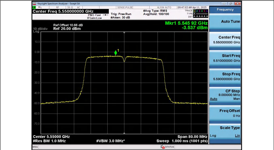
11N40SISO-Ant1-5550-PASS
