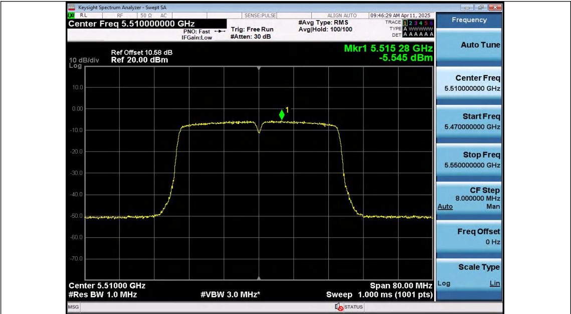
11N40SISO-Ant1-5510-PASS
