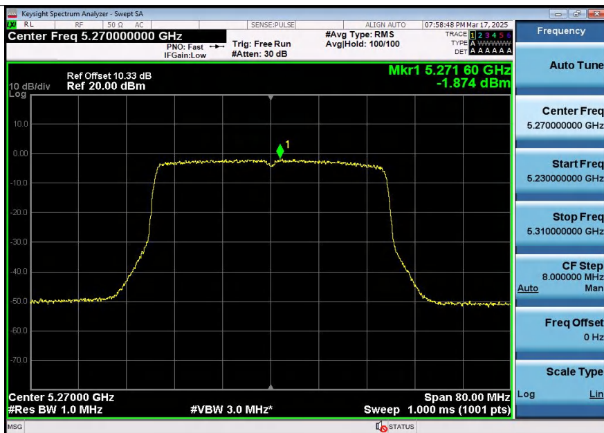
11AX40SISO-Ant1-5270-PASS
