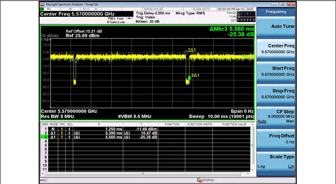
NTNV-11AC160SISO-Ant2-5570
