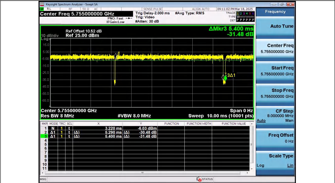
NTNV-11AX40SISO-Ant2-5755
