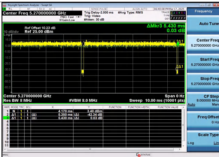
NTNV-11N40SISO-Ant2-5270
