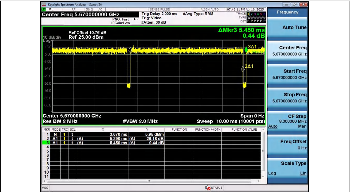
NTNV-11AX40SISO-Ant2-5670
