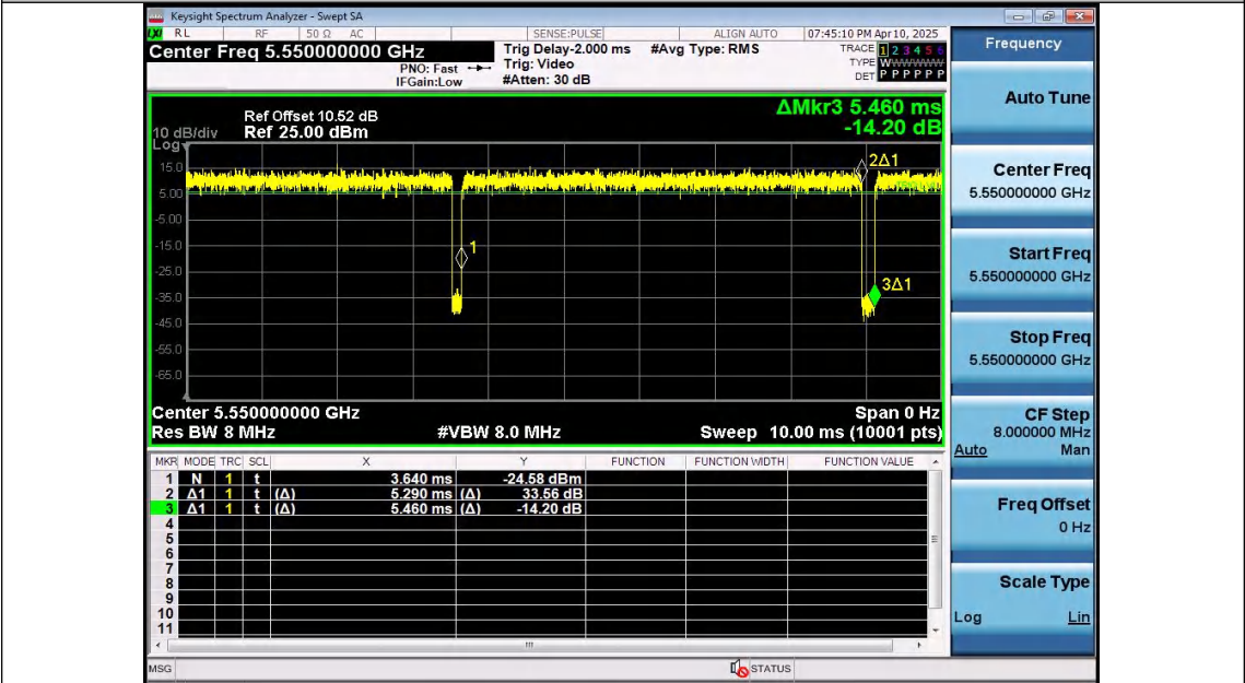
NTNV-11AX40SISO-Ant2-5550
