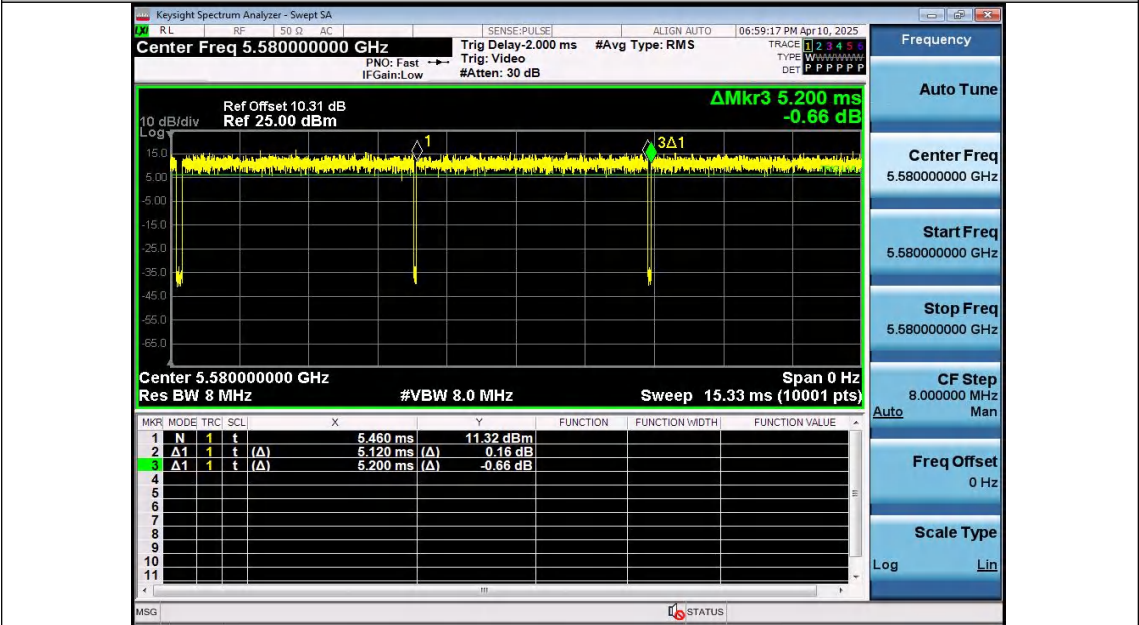
NTNV-11AX20SISO-Ant2-5580
