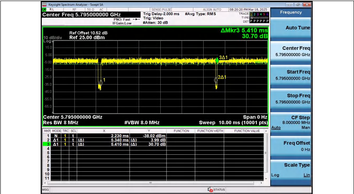
NTNV-11N40SISO-Ant2-5795
