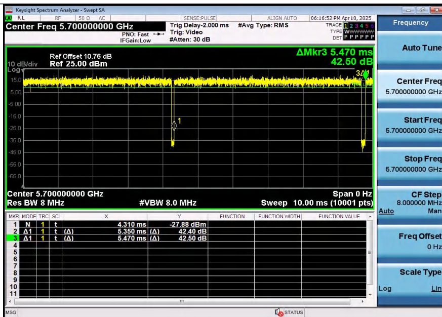
NTNV-11N20SISO-Ant2-5700
