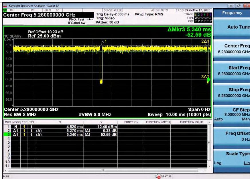
NTNV-11AX20SISO-Ant2-5280
