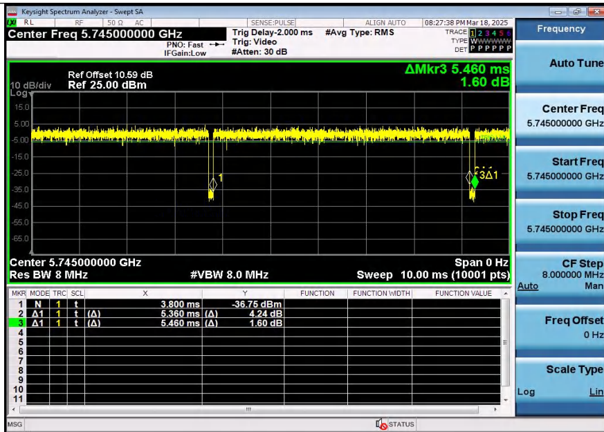
NTNV-11AC20SISO-Ant2-5745
