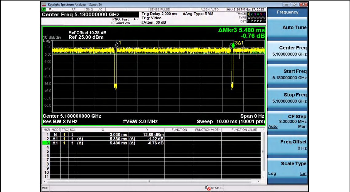
NTNV-11AC20SISO-Ant2-5180
