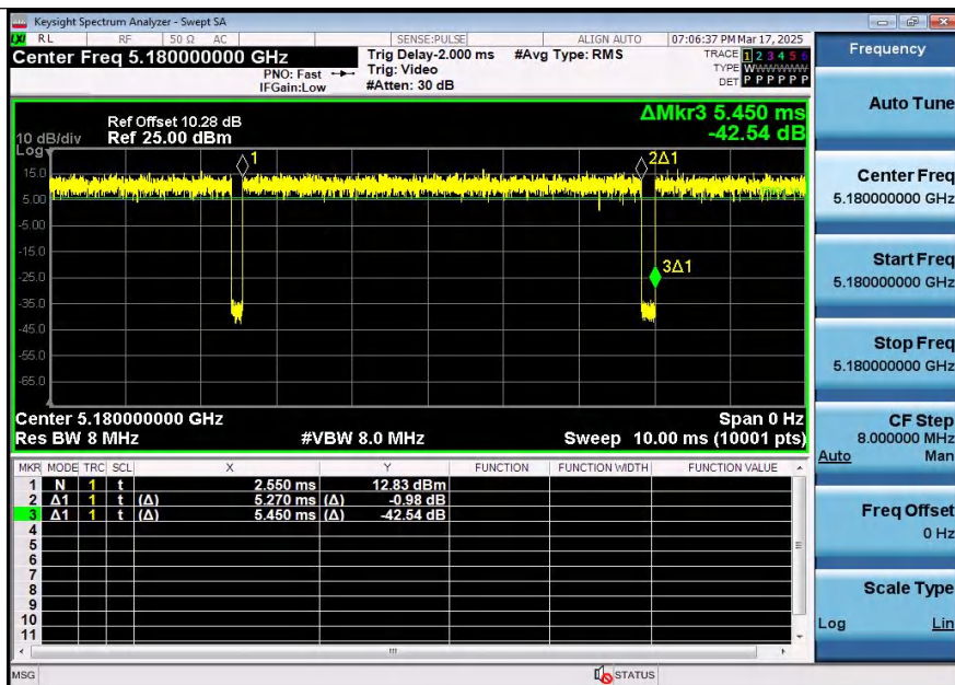
NTNV-11AX20SISO-Ant2-5180
