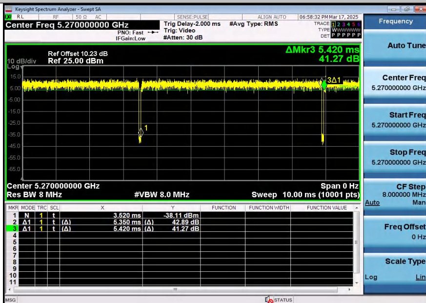
NTNV-11AC40SISO-Ant2-5270
