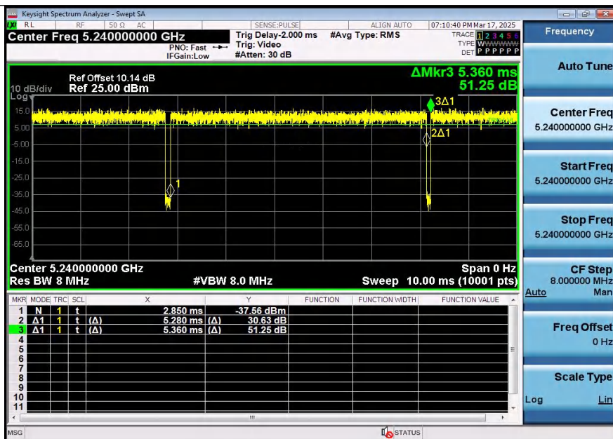
NTNV-11AX20SISO-Ant2-5240
