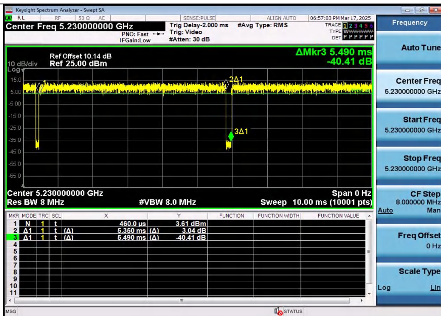
NTNV-11AC40SISO-Ant2-5230
