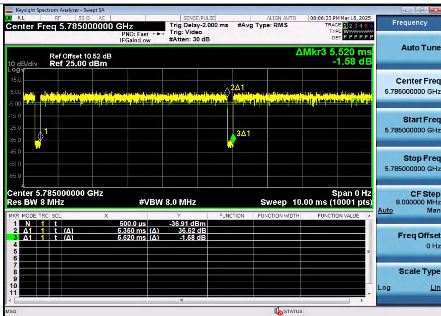
NTNV-11N20SISO-Ant2-5785
