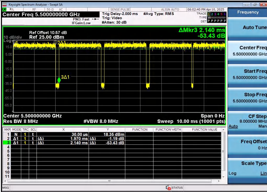
NTNV-11A-Ant2-5500
