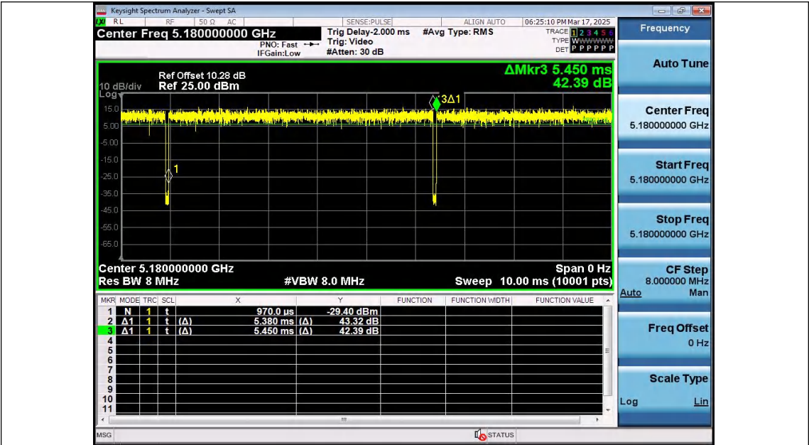
NTNV-11N20SISO-Ant2-5180
