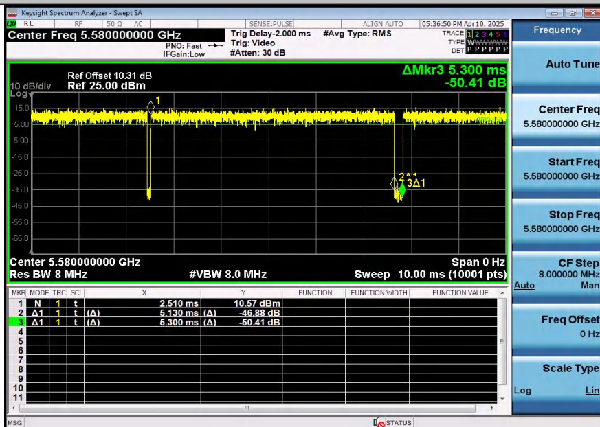
NTNV-11AX20SISO-Ant1-5580
