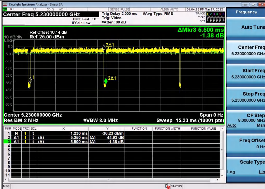
NTNV-11AX40SISO-Ant1-5230
