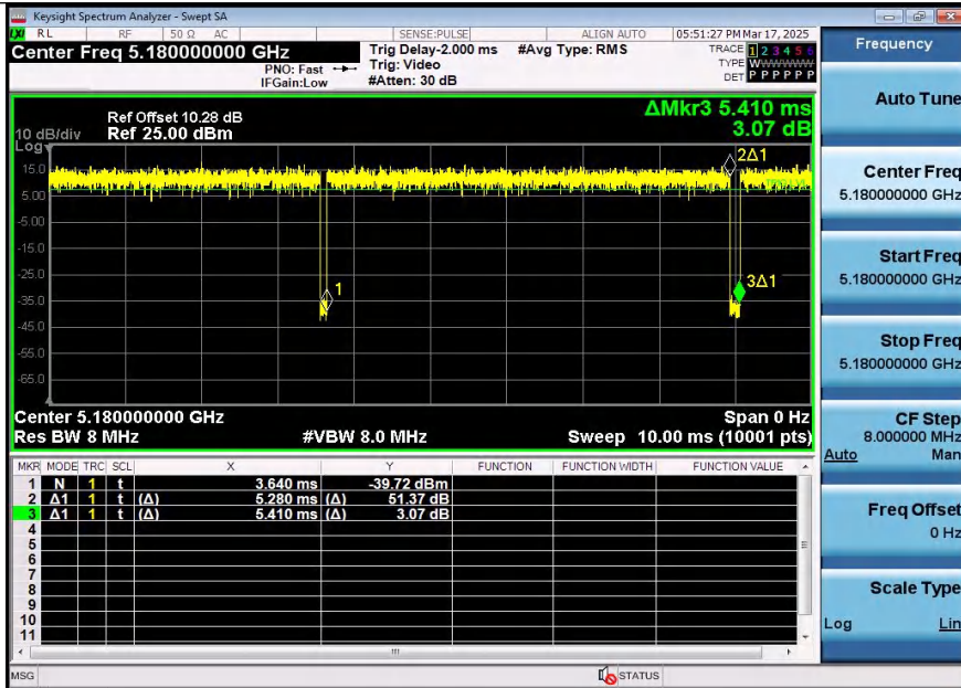
NTNV-11AX20SISO-Ant1-5180
