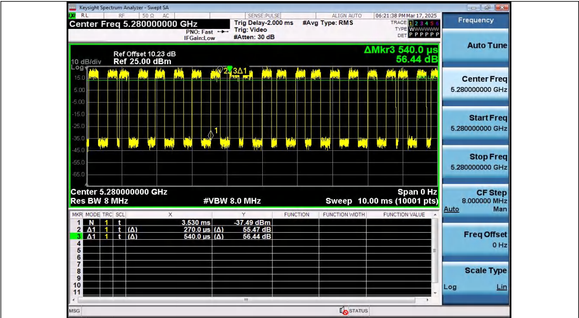
NTNV-11A-Ant2-5280
