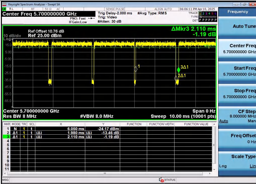
NTNV-11A-Ant2-5700
