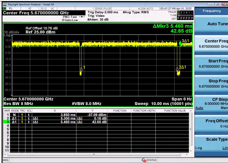
NTNV-11AX40SISO-Ant1-5670
