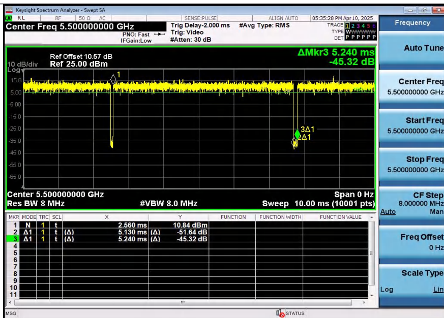
NTNV-11AX20SISO-Ant1-5500
