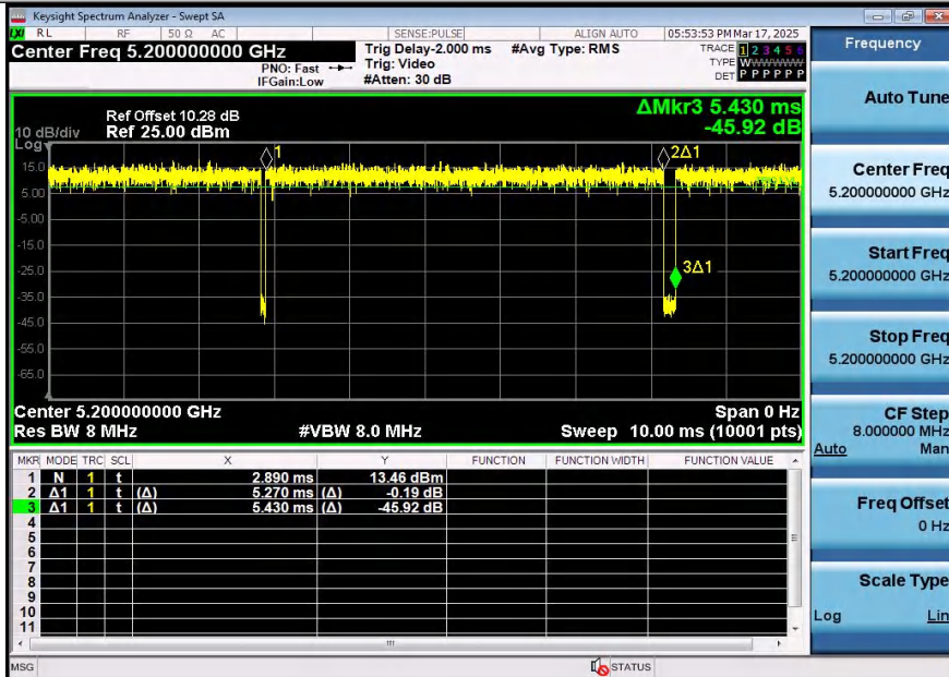
NTNV-11AX20SISO-Ant1-5200
