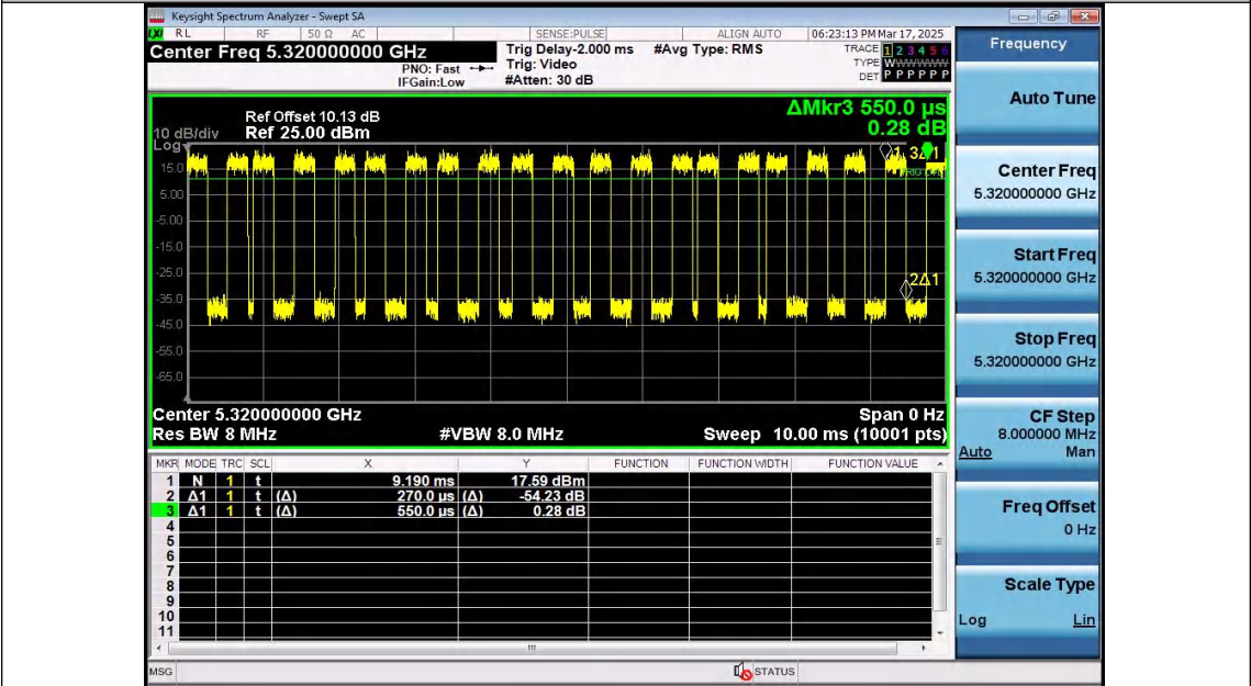
NTNV-11A-Ant2-5320
