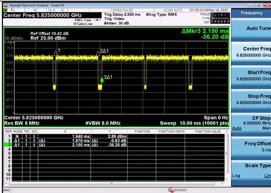
NTNV-11A-Ant2-5825
