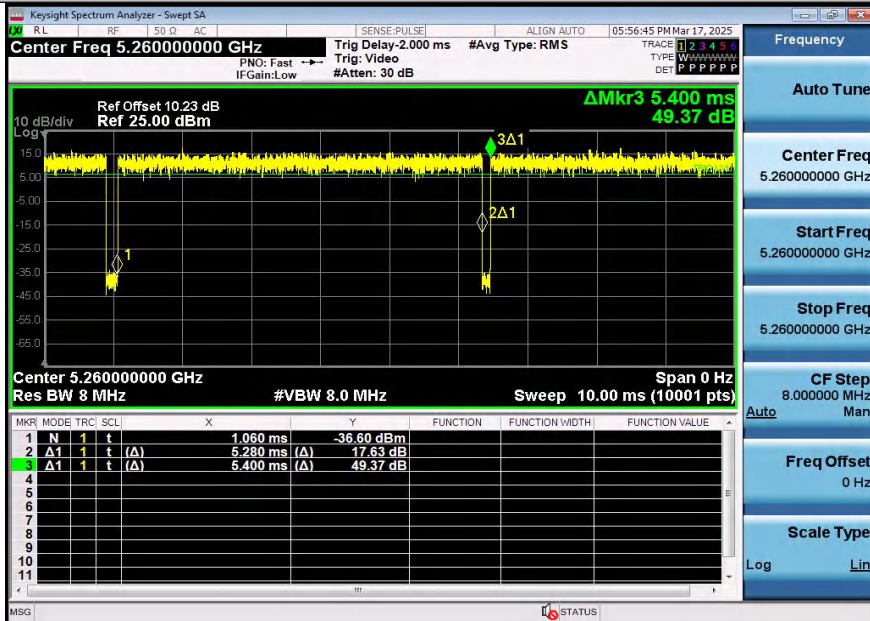
NTNV-11AX20SISO-Ant1-5260
