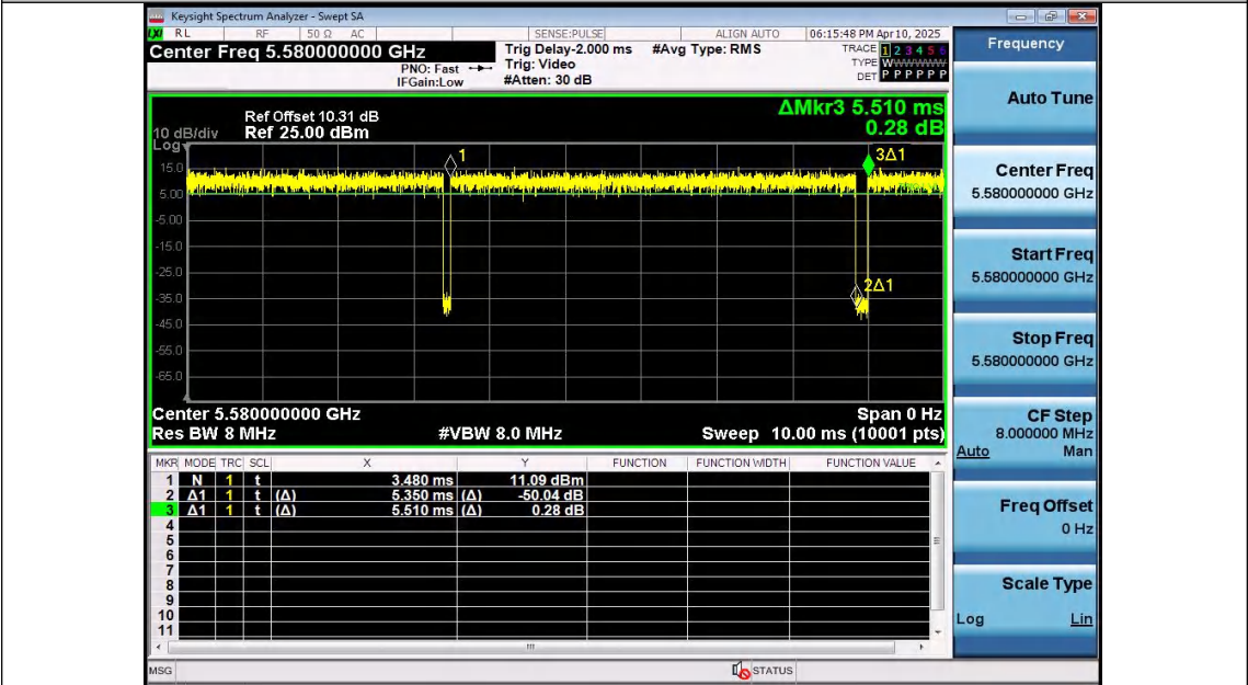
NTNV-11N20SISO-Ant2-5580
