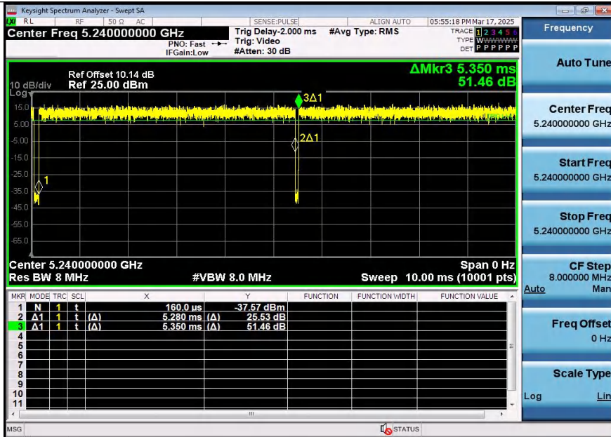
NTNV-11AX20SISO-Ant1-5240
