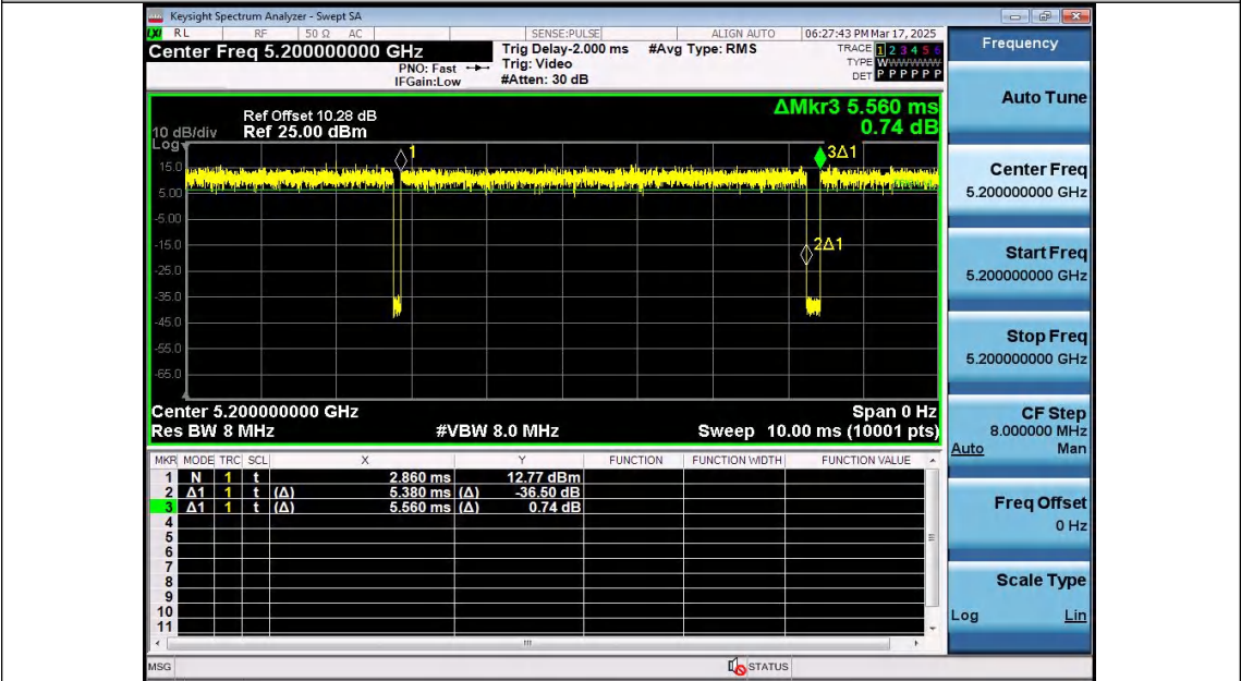
NTNV-11N20SISO-Ant2-5200
