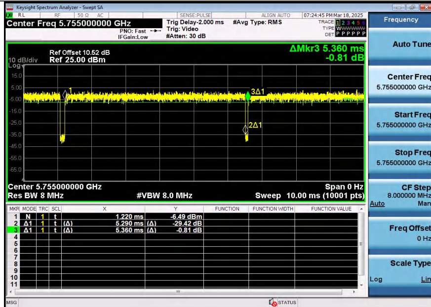
NTNV-11AX40SISO-Ant1-5755
