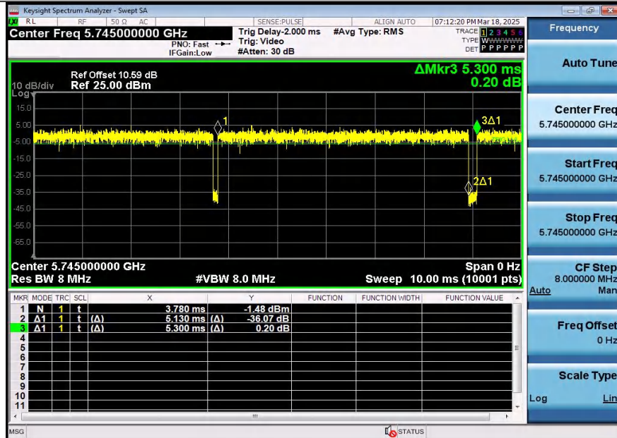
NTNV-11AX20SISO-Ant1-5745
