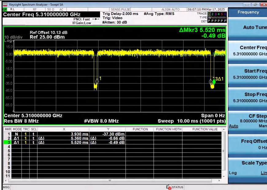
NTNV-11AX40SISO-Ant1-5310
