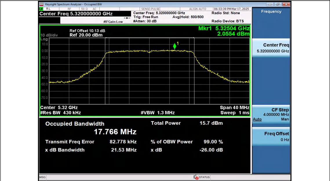
11N20SISO-Ant2-5320
