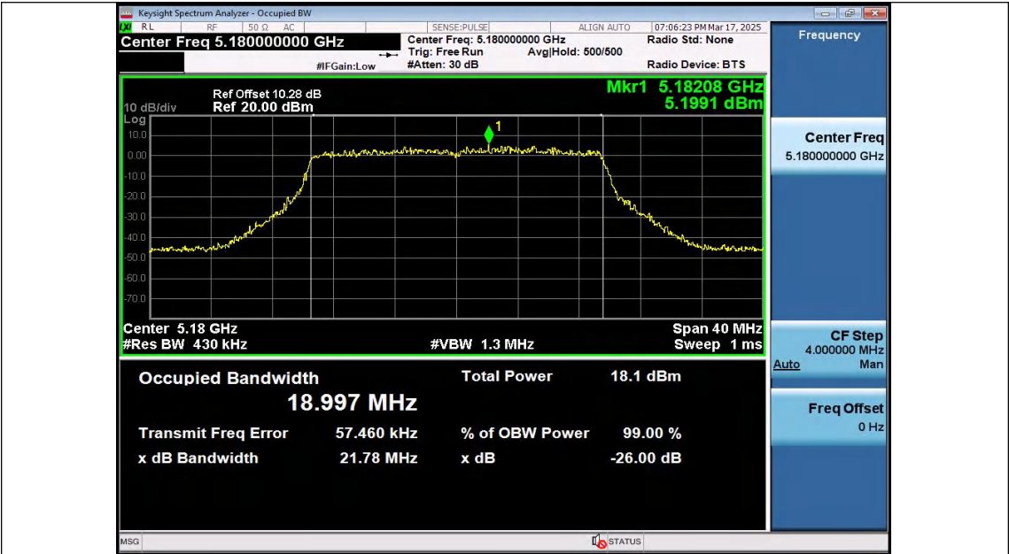
11AX20SISO-Ant2-5180
