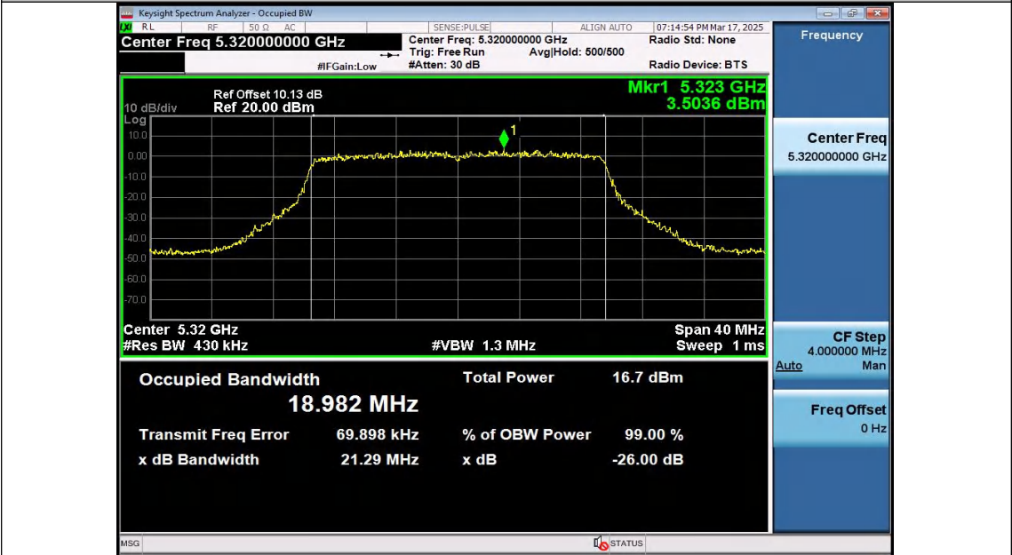
11AX20SISO-Ant2-5320
