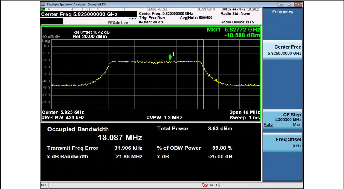
11N20SISO-Ant2-5825
