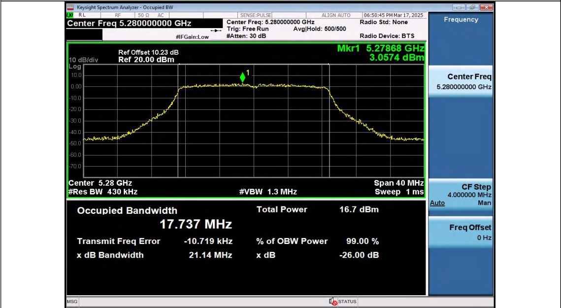
11AC20SISO-Ant2-5280
