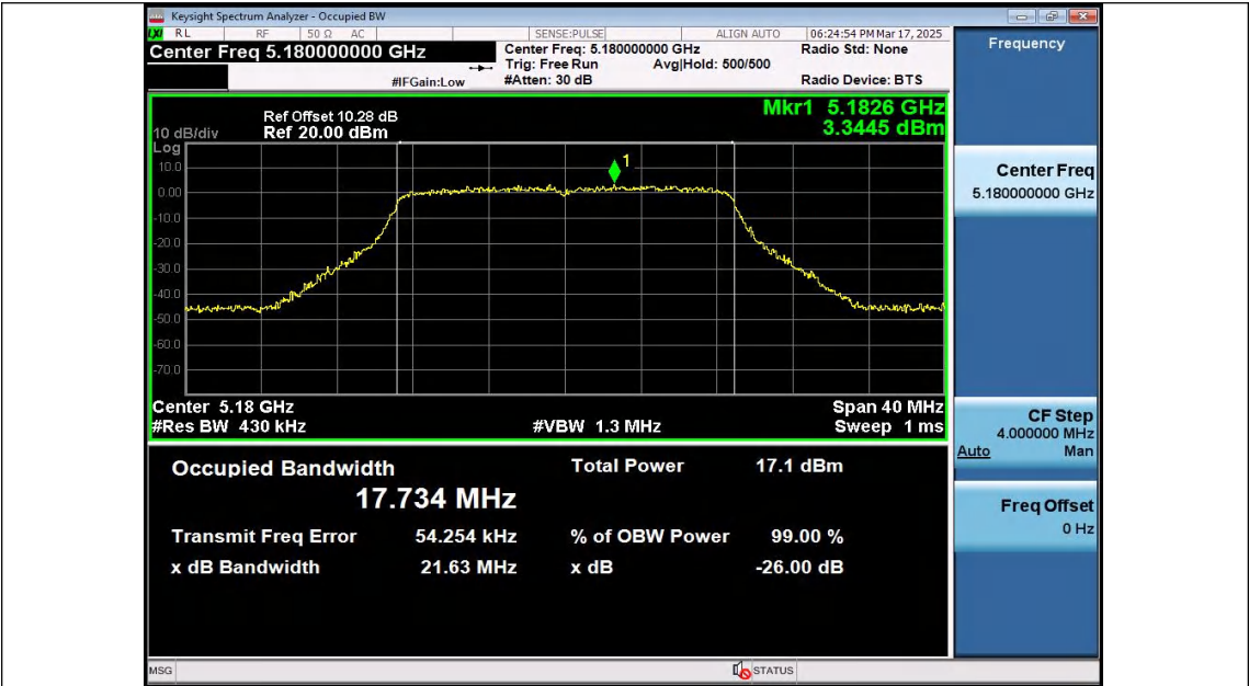
11N20SISO-Ant2-5180
