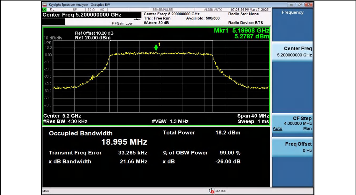
11AX20SISO-Ant2-5200
