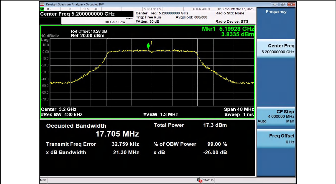
11N20SISO-Ant2-5200
