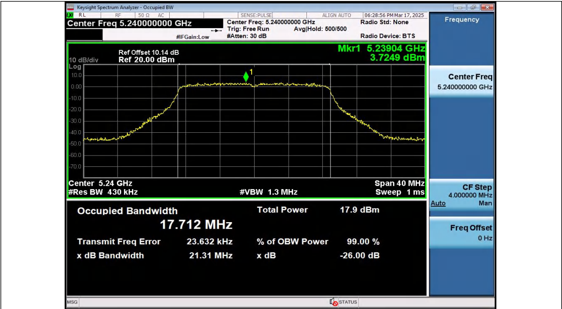
11N20SISO-Ant2-5240
