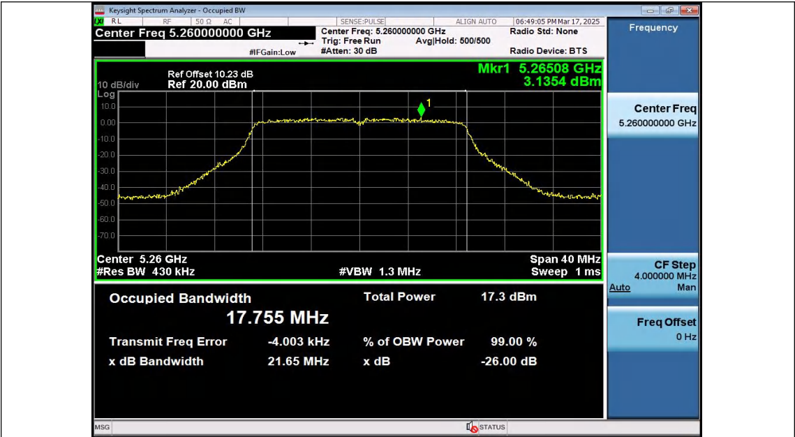
11AC20SISO-Ant2-5260
