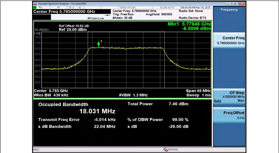
11N20SISO-Ant2-5785
