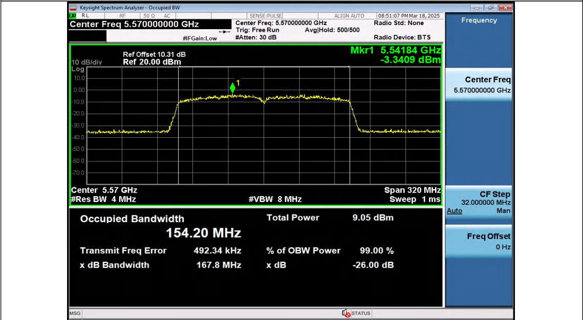
11AC160SISO-Ant2-5570
