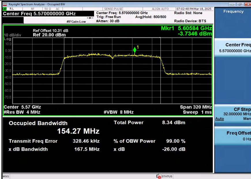
11AC160SISO-Ant1-5570
