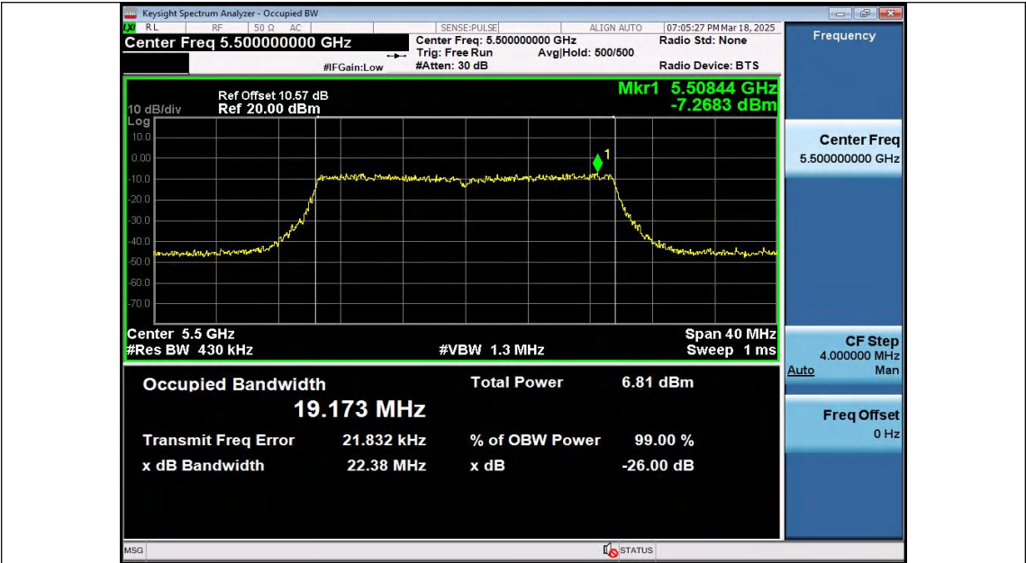
11AX20SISO-Ant1-5500
