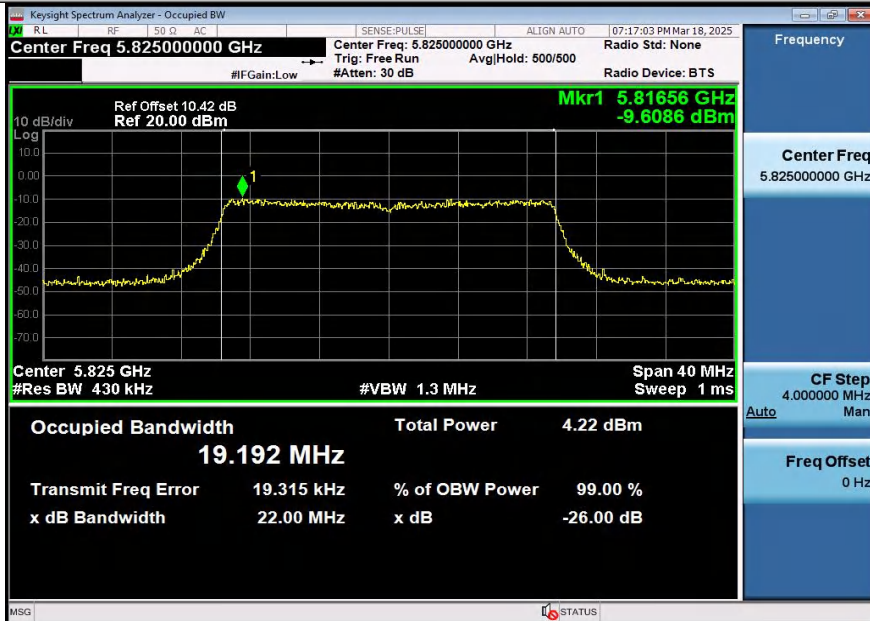
11AX20SISO-Ant1-5825
