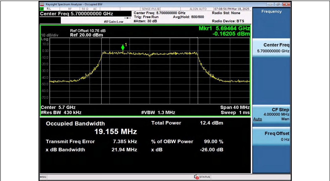
11AX20SISO-Ant1-5700
