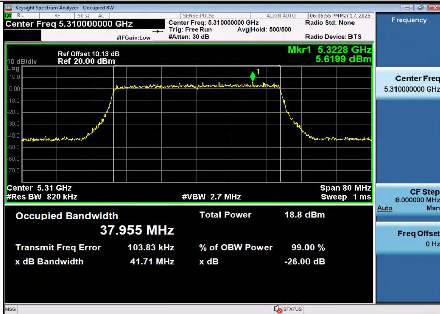
11AX40SISO-Ant1-5310
