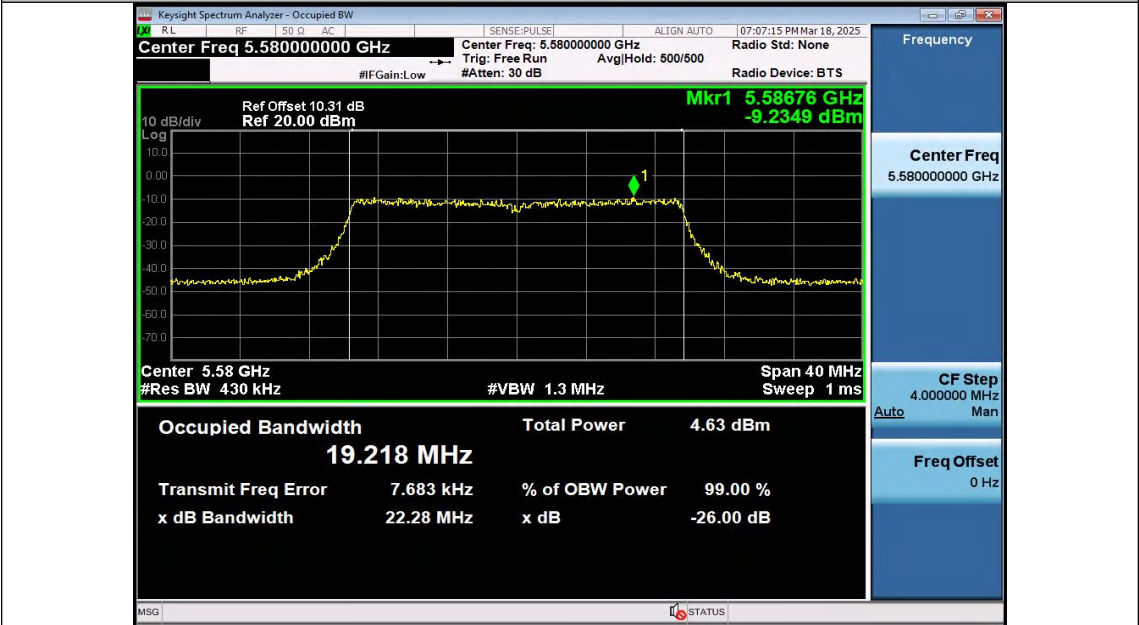
11AX20SISO-Ant1-5580
