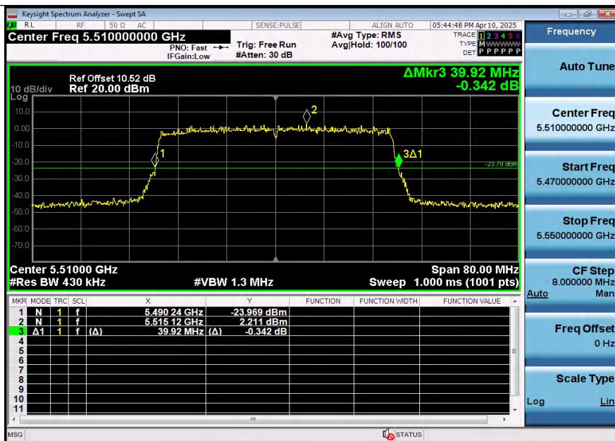
11AX40SISO-Ant1-5510
