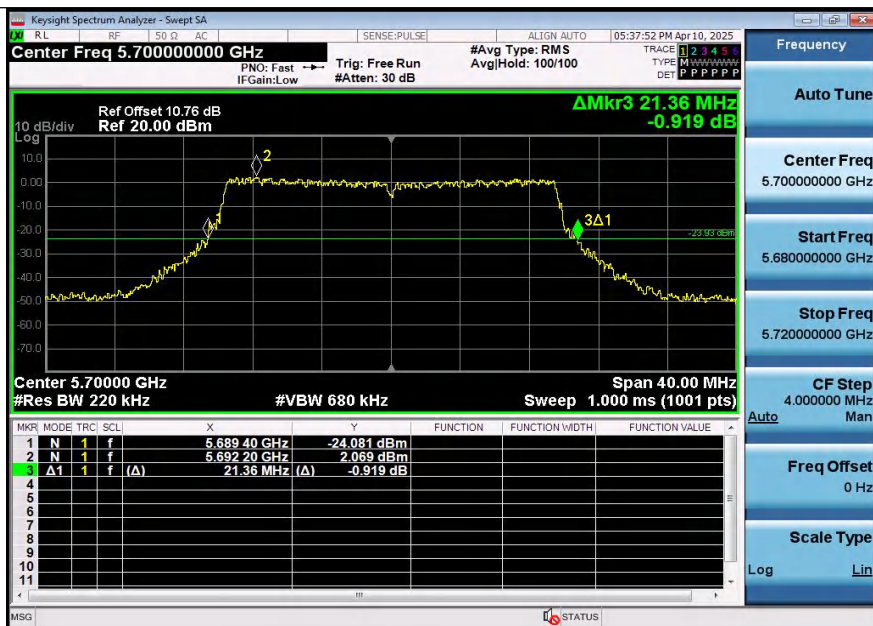
11AX20SISO-Ant1-5700
