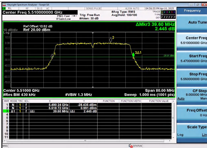
11N40SISO-Ant1-5510
