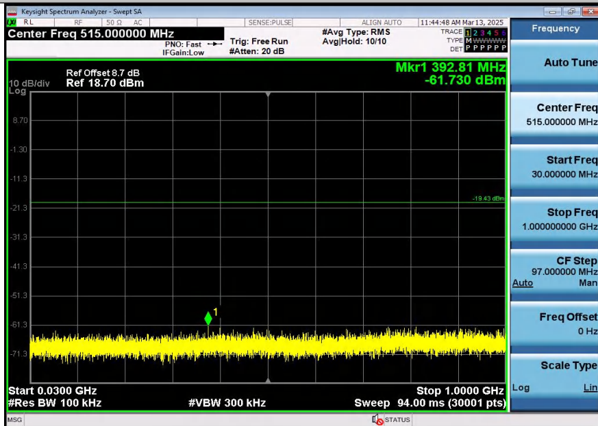
11N20SISO-Ant2-2462-30~1000-PASS
