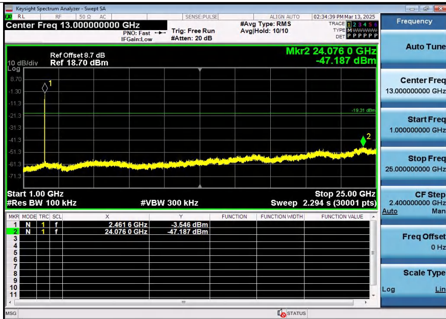
11AX20SISO-Ant2-2462-1000~25000-PASS
