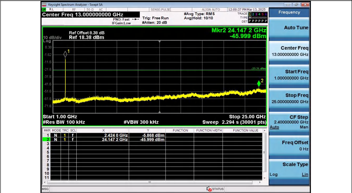
11N40SISO-Ant2-2422-1000~25000-PASS
