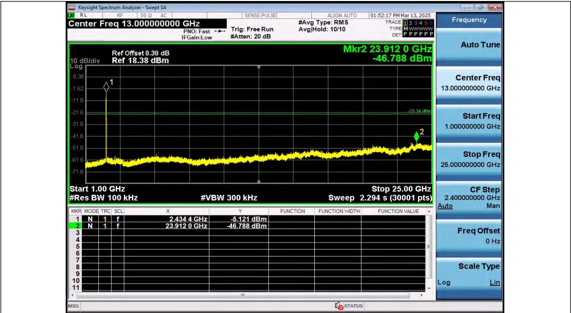
11N40SISO-Ant2-2437-1000~25000-PASS
