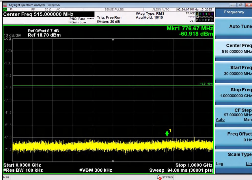
11AX20SISO-Ant2-2462-30~1000-PASS
