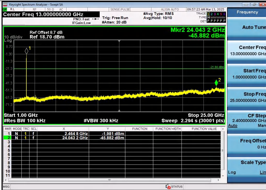
11AX20SISO-Ant1-2462-1000~25000-PASS
