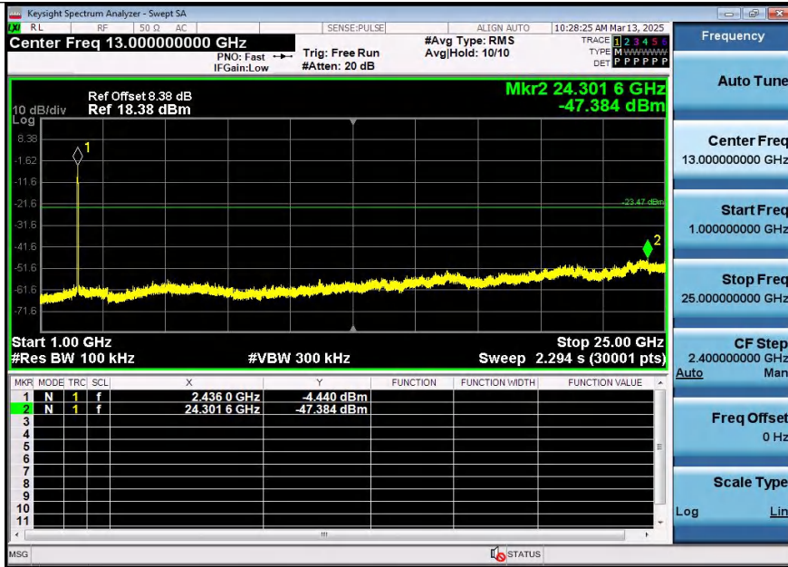
11AX40SISO-Ant1-2437-1000~25000-PASS
