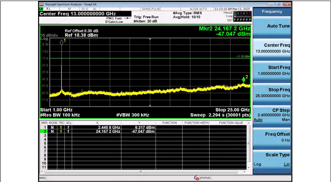
11G-Ant2-2437-1000~25000-PASS
