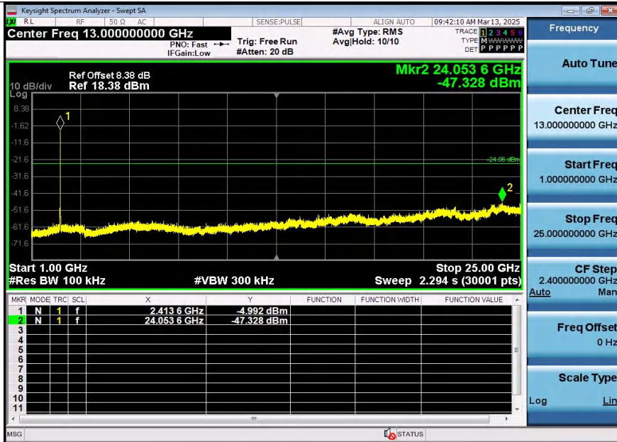
11AX20SISO-Ant1-2412-1000~25000-PASS
