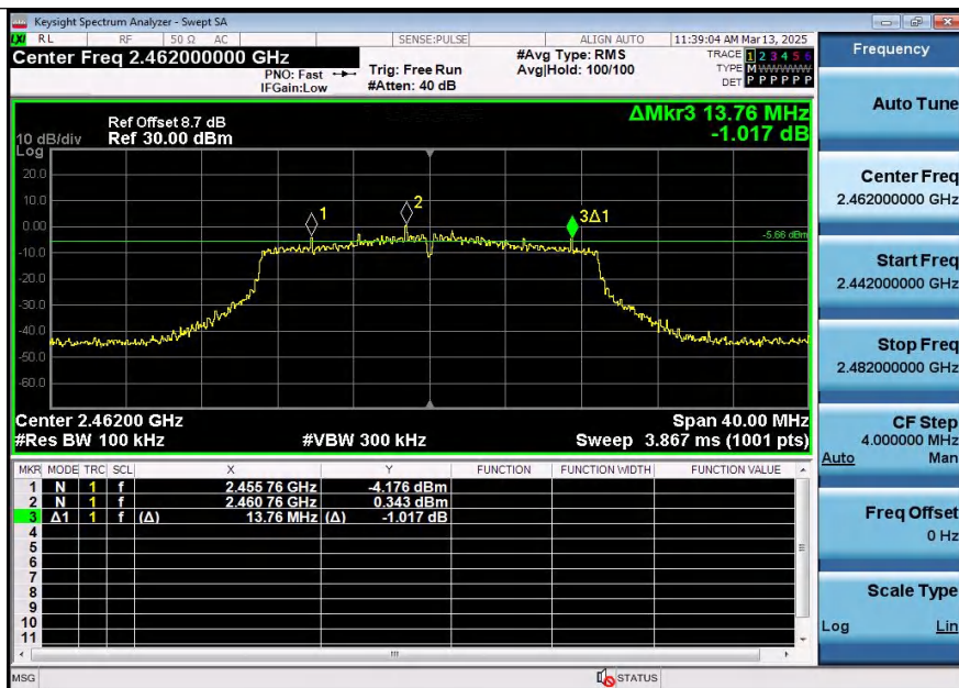
11N20SISO-Ant2-2462-PASS
