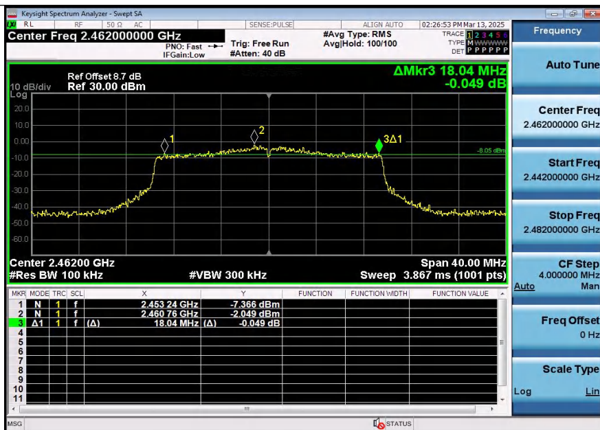
11AX20SISO-Ant2-2462-PASS
