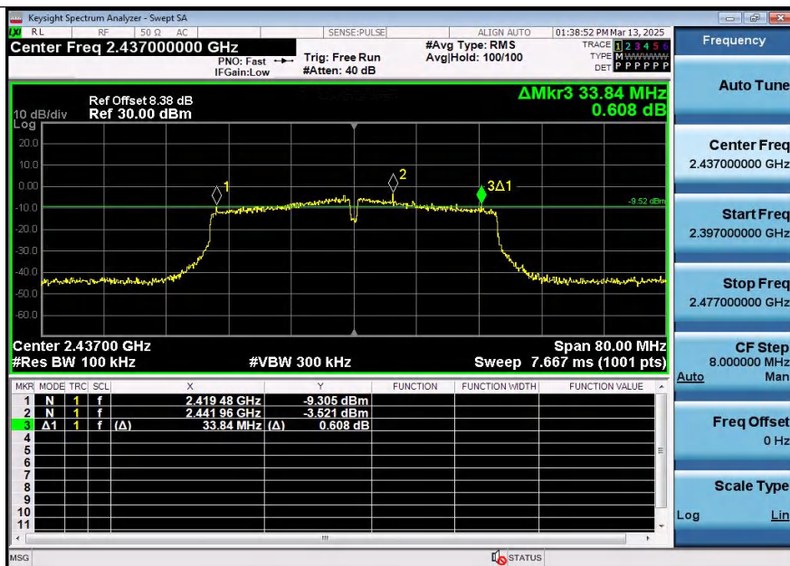
11N40SISO-Ant2-2437-PASS
