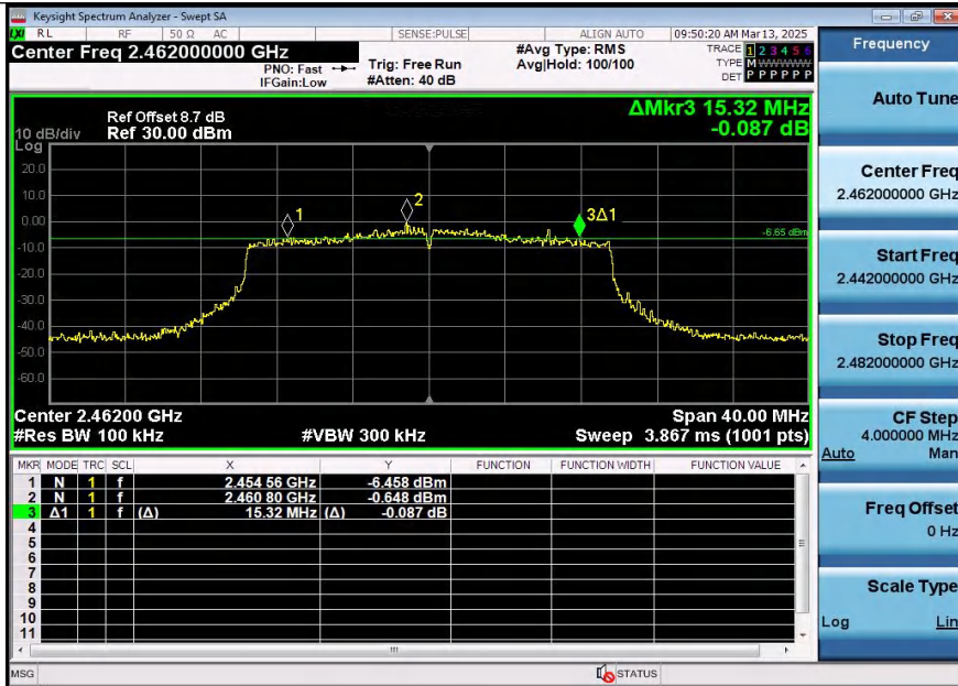
11AX20SISO-Ant1-2462-PASS
