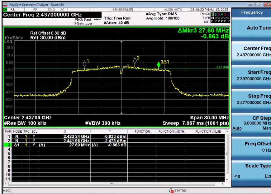
11N40SISO-Ant1-2437-PASS
