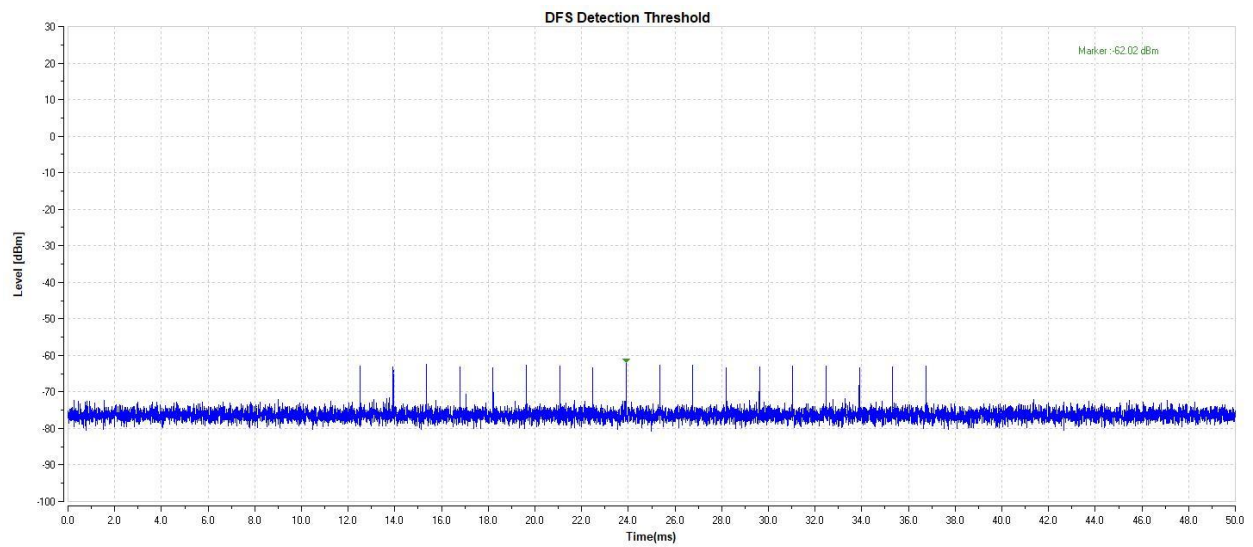
11AC80-5290-Type0-PASS
