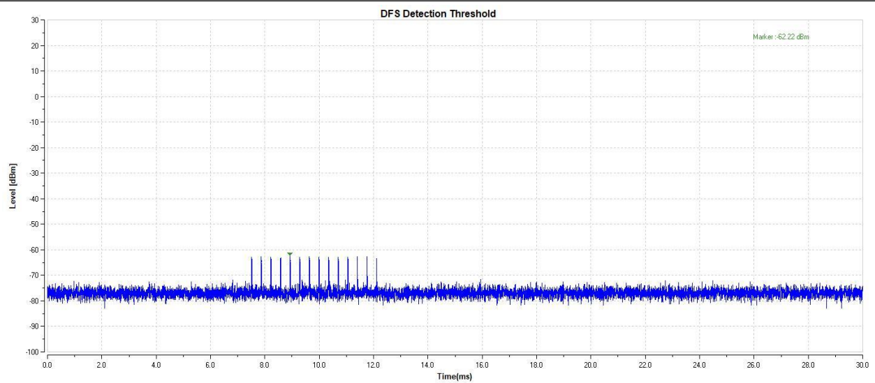
11AC80-5290-Type4-PASS
