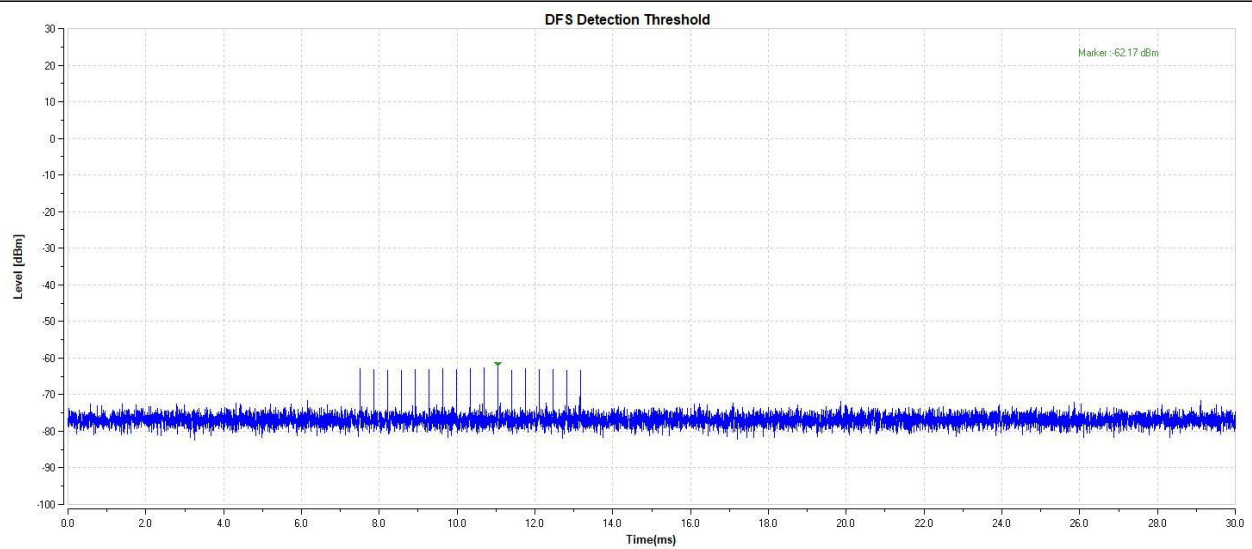
11AC80-5530-Type3-PASS
