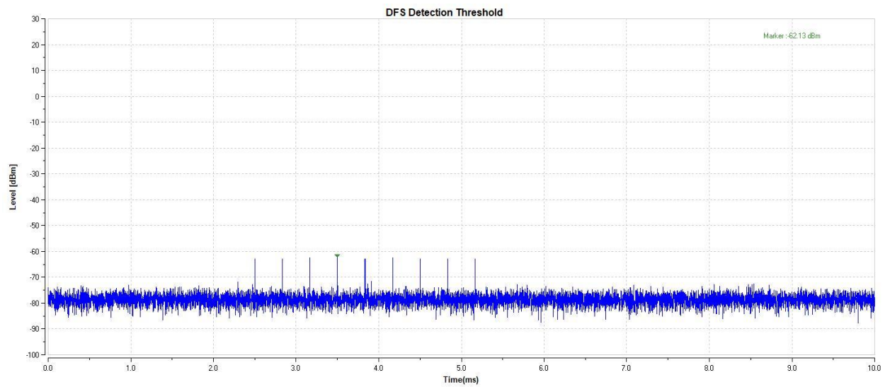
11AC80-5290-Type6-PASS
