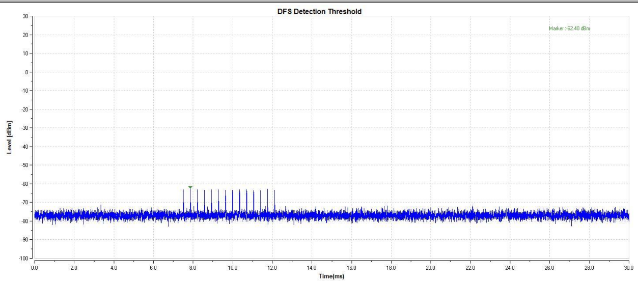
11A-5500-Type4-PASS
