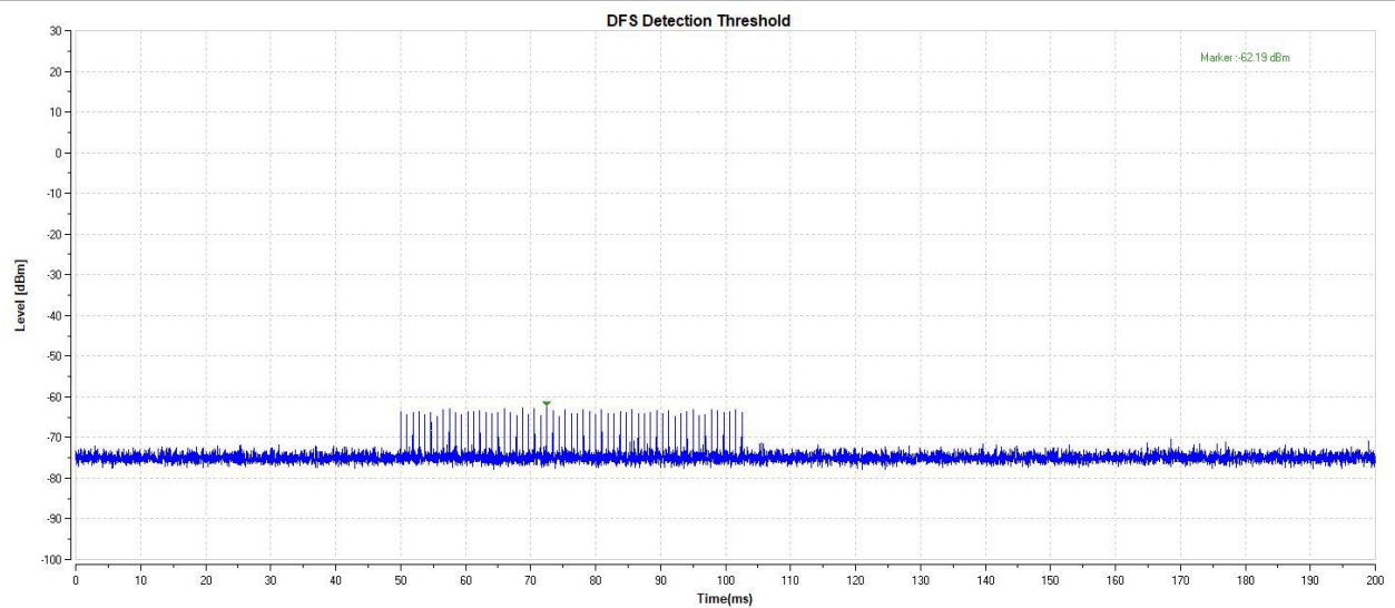
11A-5260-Type1-PASS
