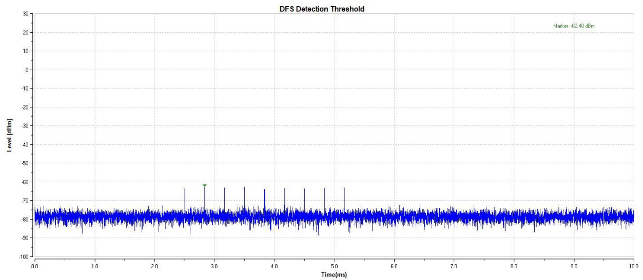
11A-5500-Type6-PASS
