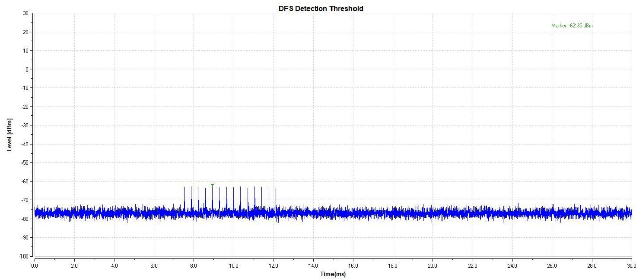
11AC80-5530-Type4-PASS
