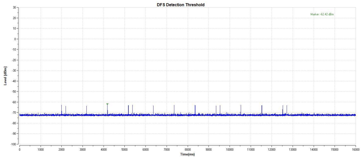
11AC80-5290-Type5-PASS
