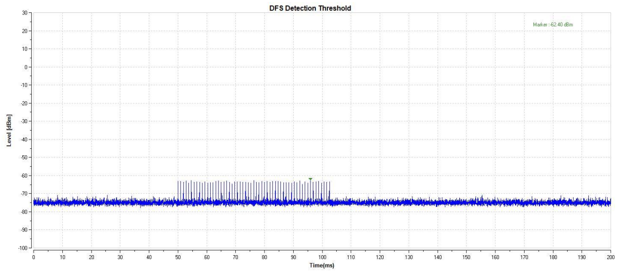
11AC80-5530-Type1-PASS
