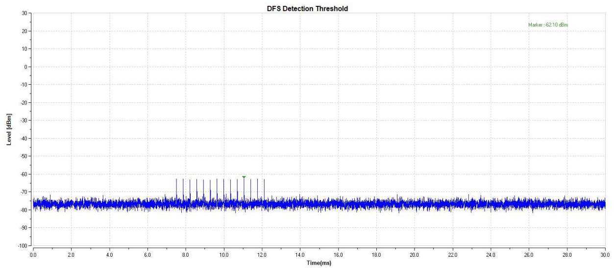
11AC160-5570-Type4-PASS
