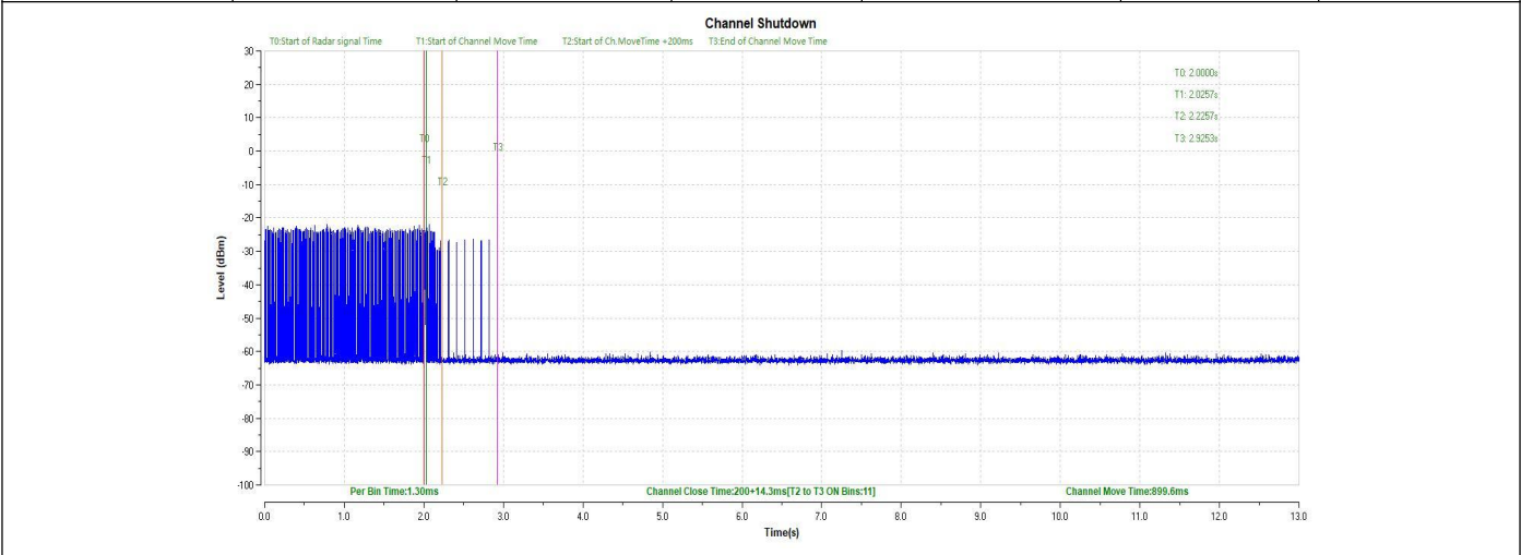
11AC80_5290
