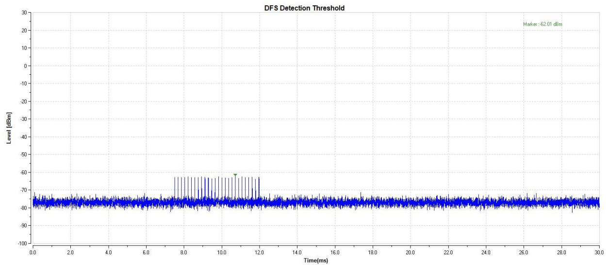
11AC80-5290-Type2-PASS
