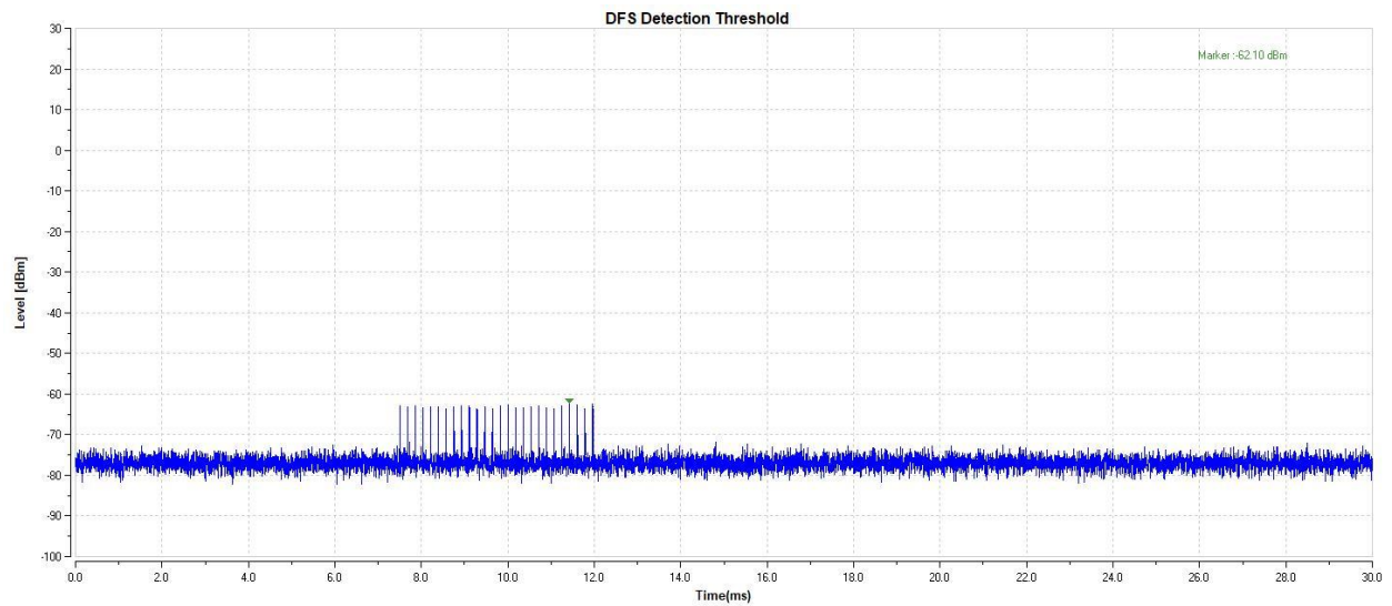
11A-5500-Type2-PASS
