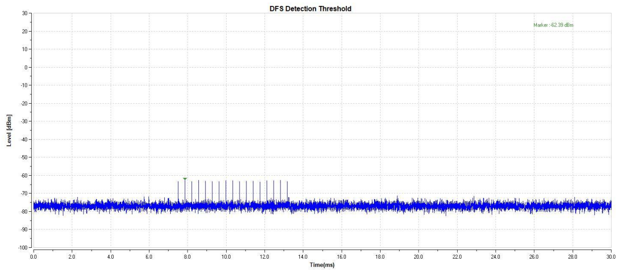
11AC80-5290-Type3-PASS
