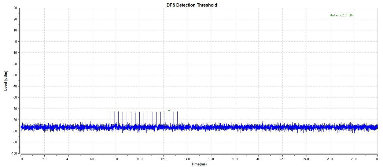
11AC160-5570-Type3-PASS
