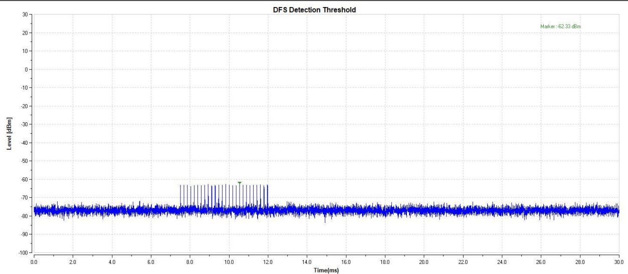
11A-5260-Type2-PASS
