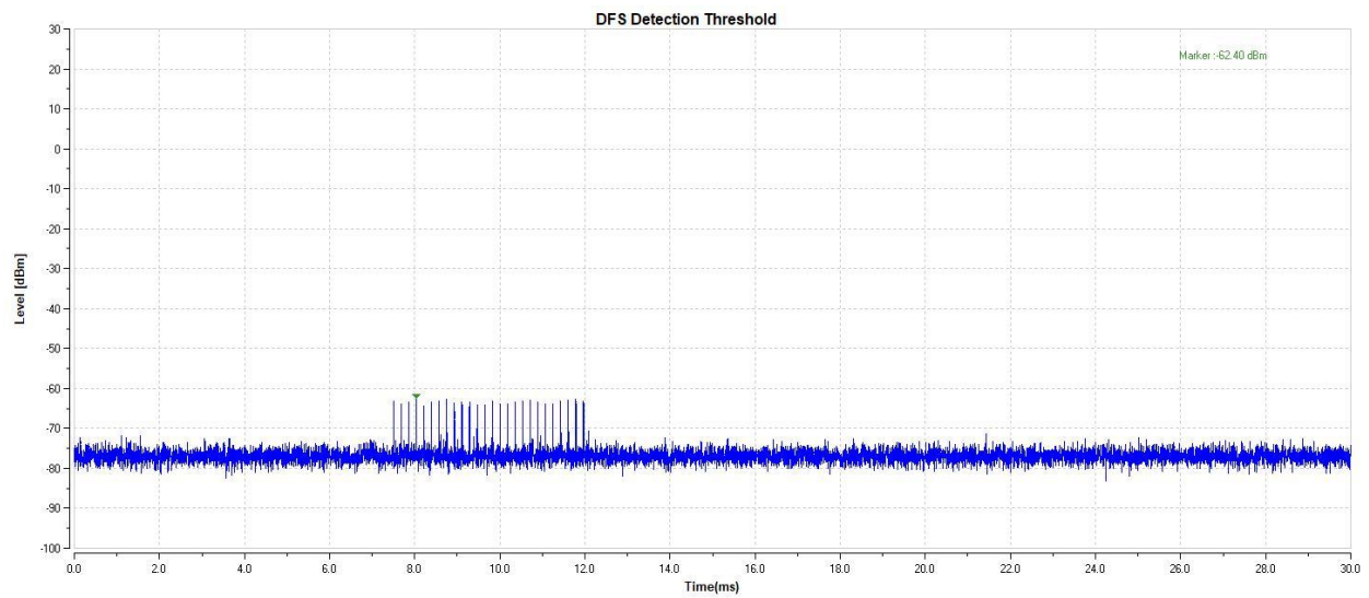
11AC80-5530-Type2-PASS
