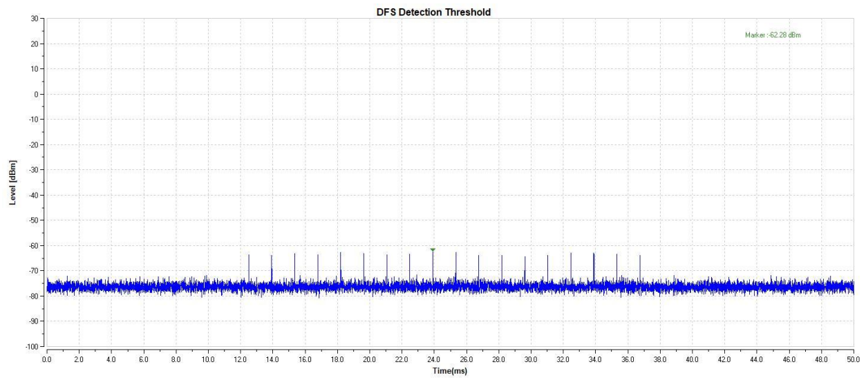
11A-5500-Type0-PASS
