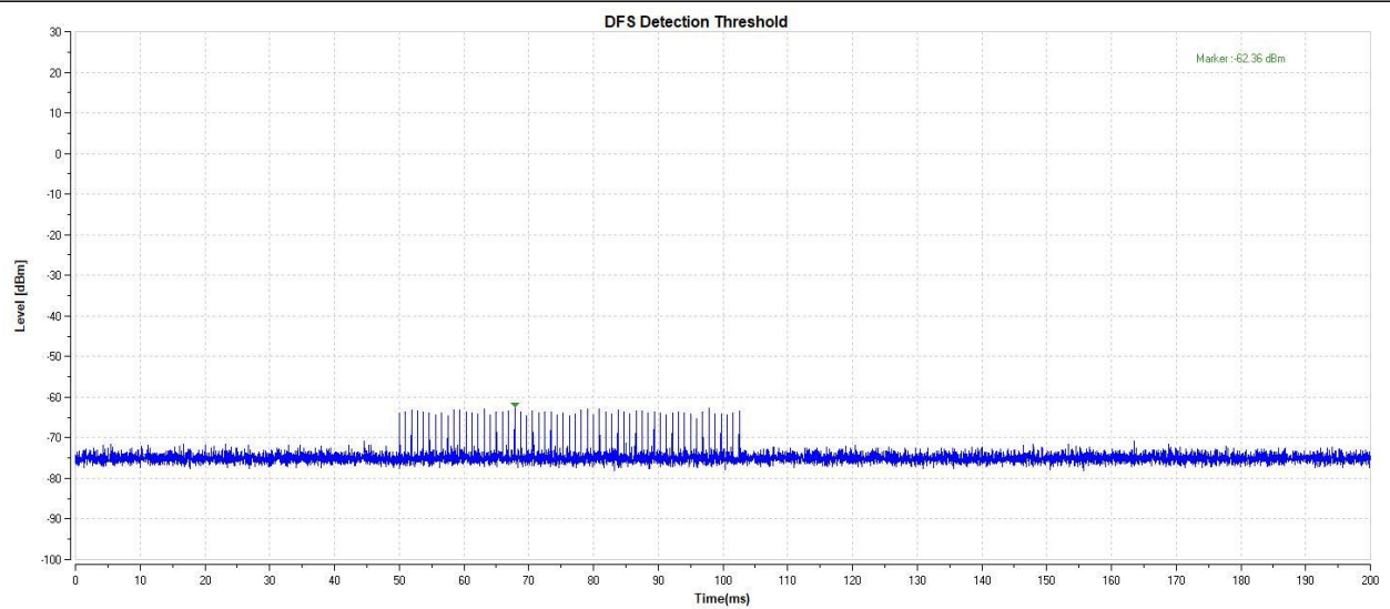
11A-5500-Type1-PASS
