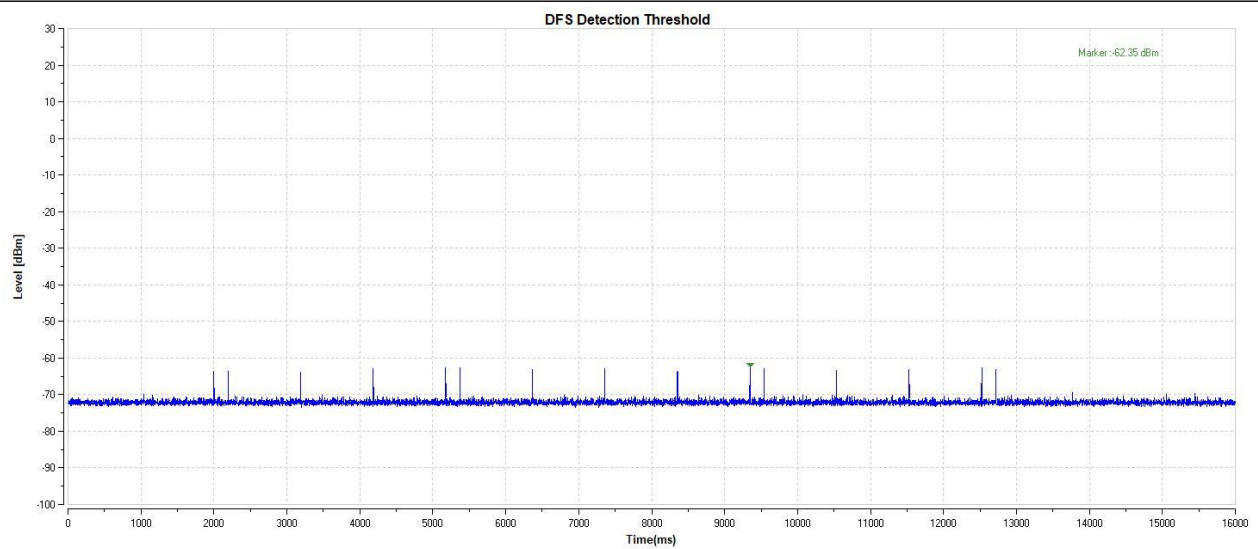
11AC160-5570-Type5-PASS
