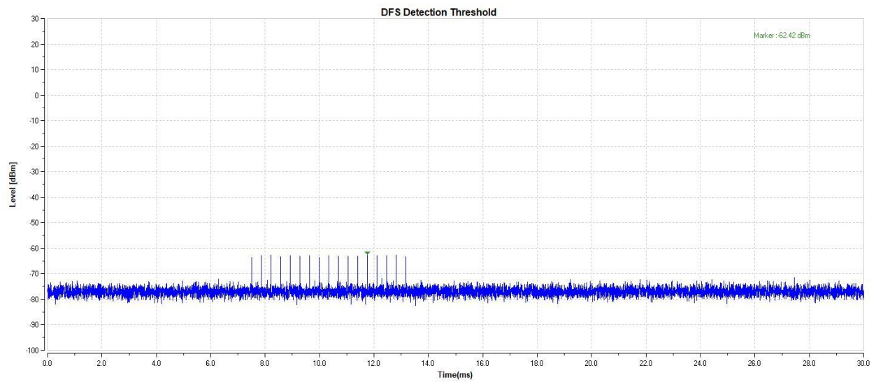
11A-5500-Type3-PASS
