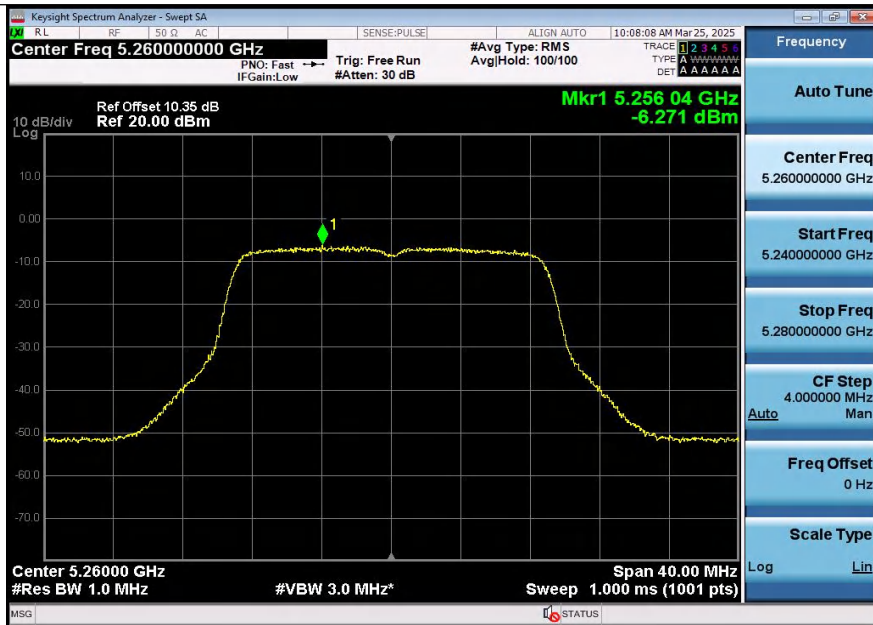
11AC20SISO-Ant2-5260-PASS
