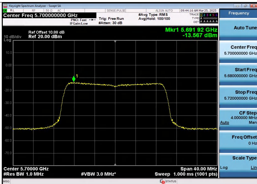
11AX20SISO-Ant2-5700-PASS
