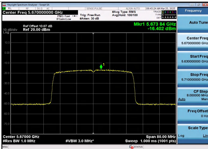
11AX40SiSO-Ant2-5670-PASS
