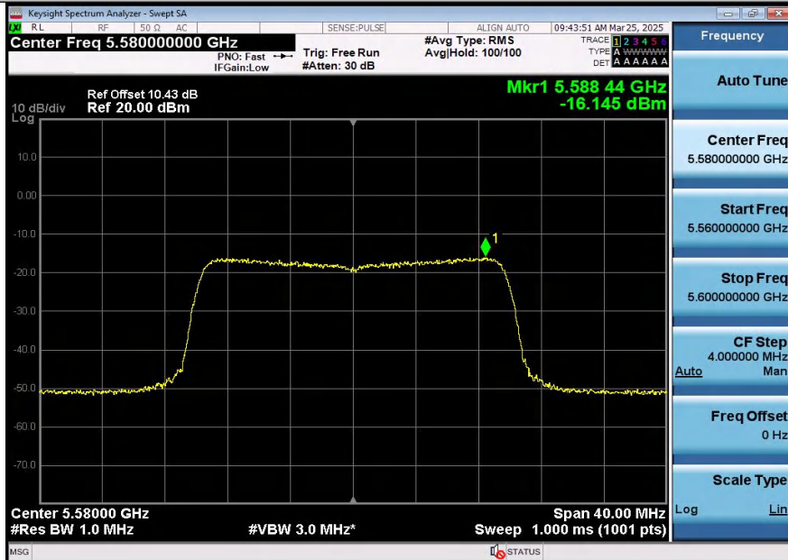
11AX20SISO-Ant2-5580-PASS
