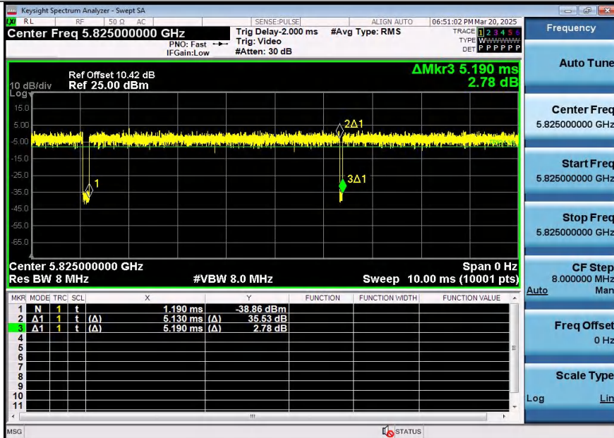
NTNV-11AX20SISO-Ant2-5825
