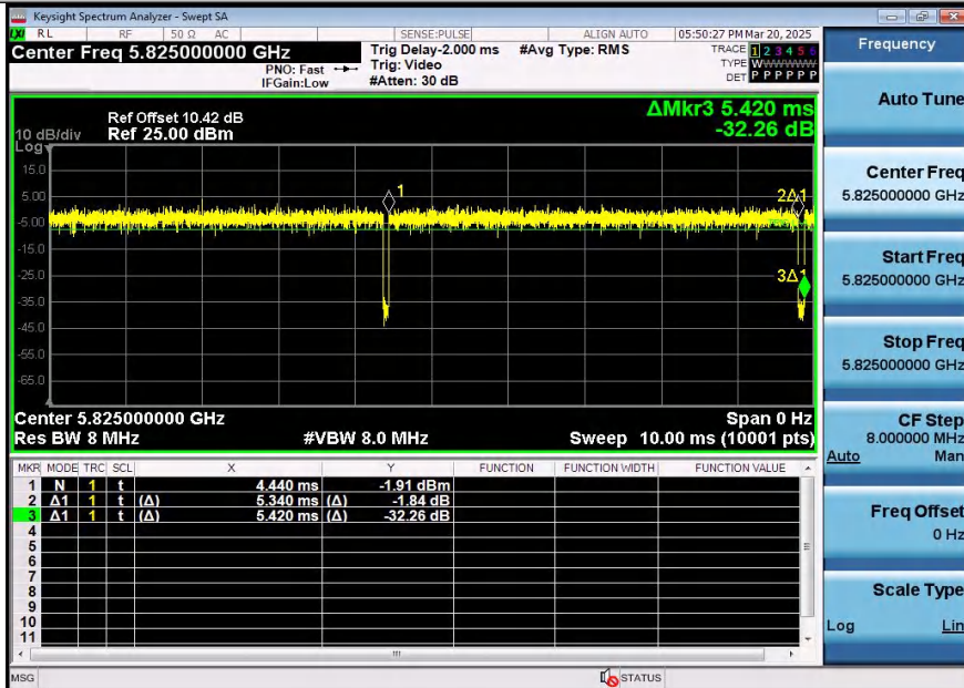
NTNV-11N20SISO-Ant2-5825
