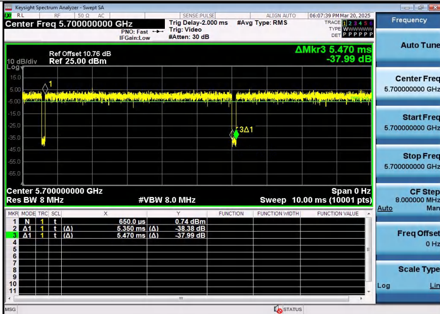
NTNV-11AC20SISO-Ant2-5700
