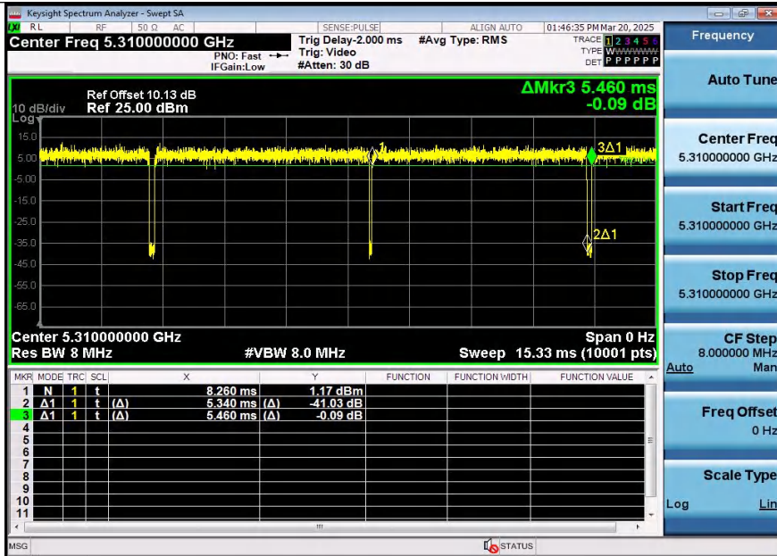
NTNV-11AC40SISO-Ant2-5310
