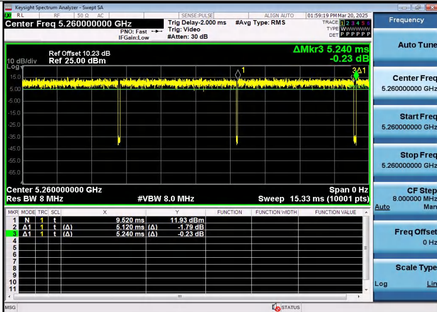
NTNV-11AX20SISO-Ant2-5260
