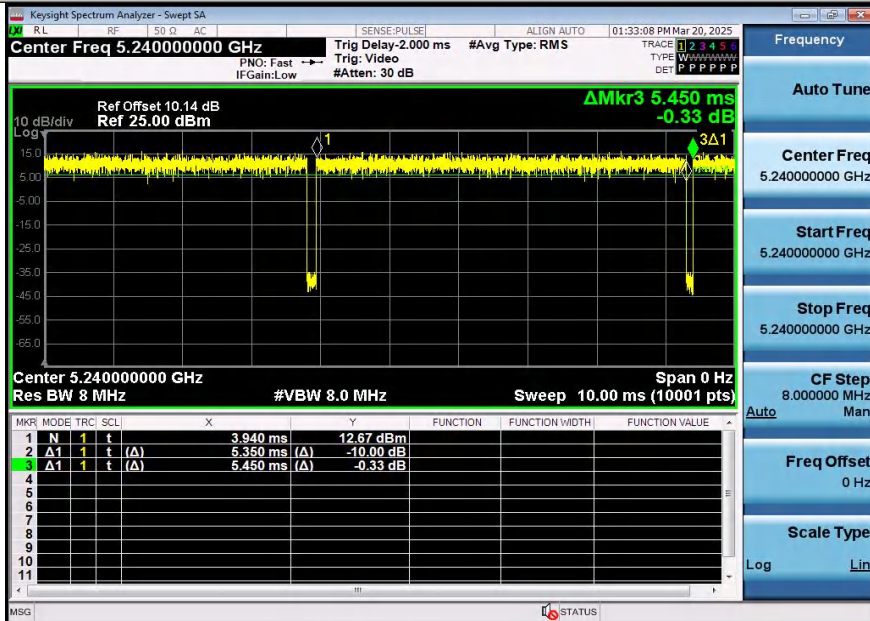
NTNV-11AC20SISO-Ant2-5240
