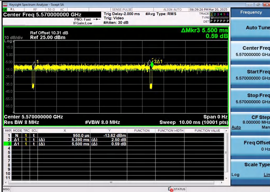
NTNV-11AC160SISO-Ant2-5570
