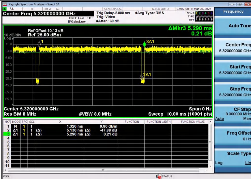
NTNV-11AX20SISO-Ant2-5320
