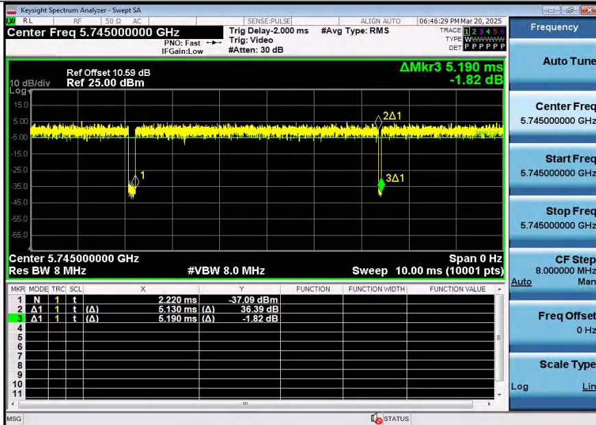
NTNV-11AX20SISO-Ant2-5745
