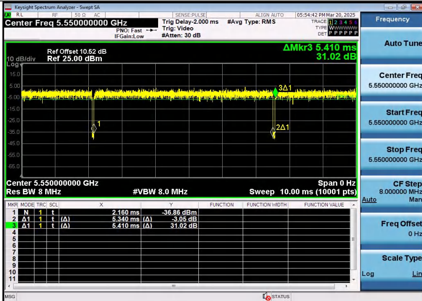
NTNV-11N40SISO-Ant2-5550
