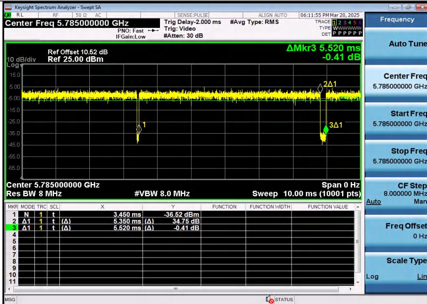
NTNV-11AC20SISO-Ant2-5785
