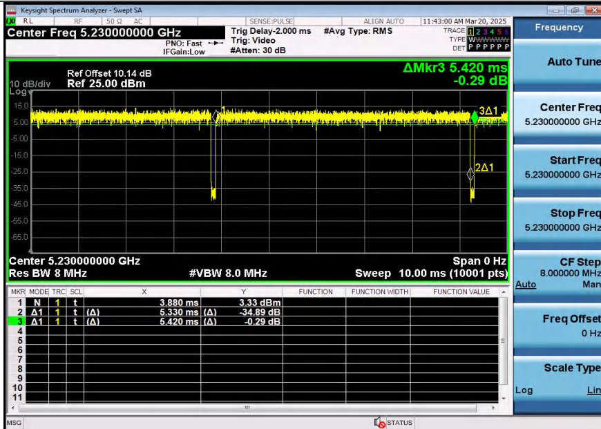
NTNV-11N40SISO-Ant2-5230
