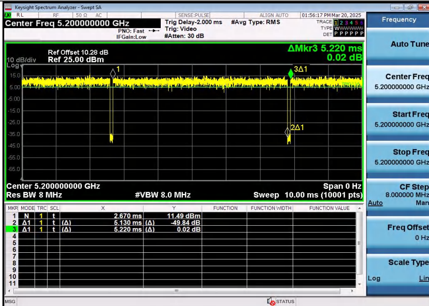
NTNV-11AX20SISO-Ant2-5200
