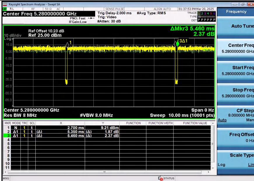
NTNV-11AC20SISO-Ant2-5280
