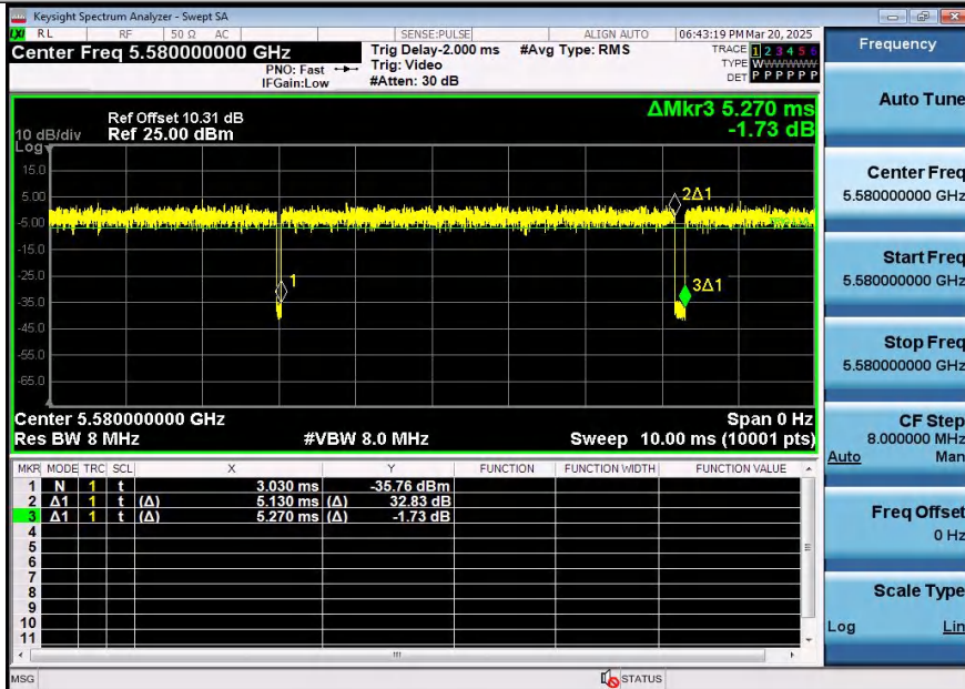
NTNV-11AX20SISO-Ant2-5580
