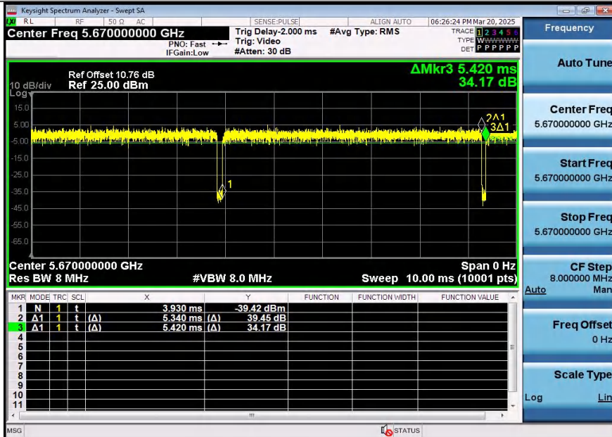
NTNV-11AC40SISO-Ant2-5670
