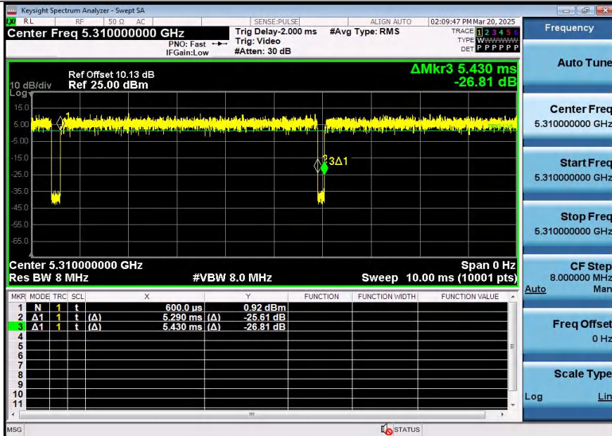
NTNV-11AX40SISO-Ant2-5310
