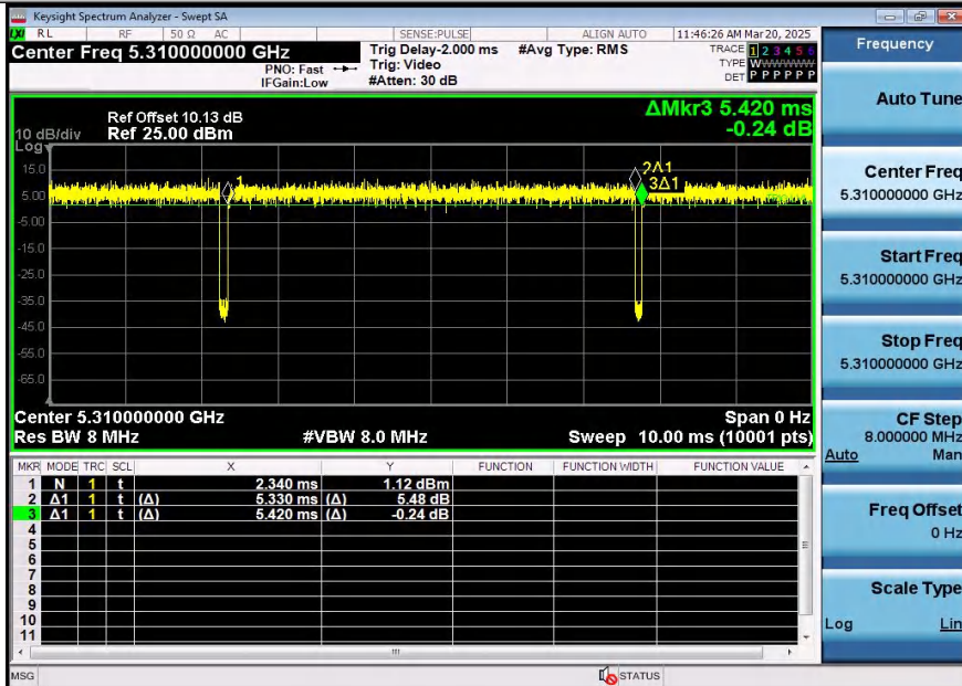
NTNV-11N40SISO-Ant2-5310
