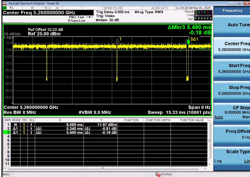
NTNV-11N20SISO-Ant2-5260
