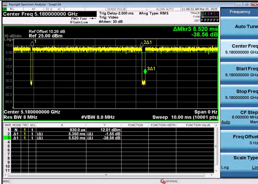
NTNV-11AC20SISO-Ant2-5180
