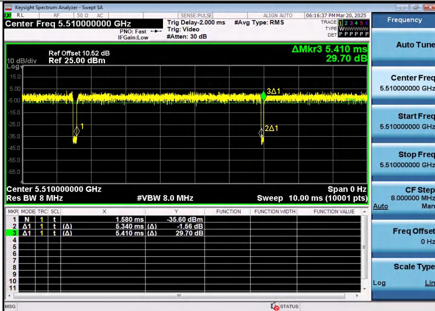
NTNV-11AC40SISO-Ant2-5510
