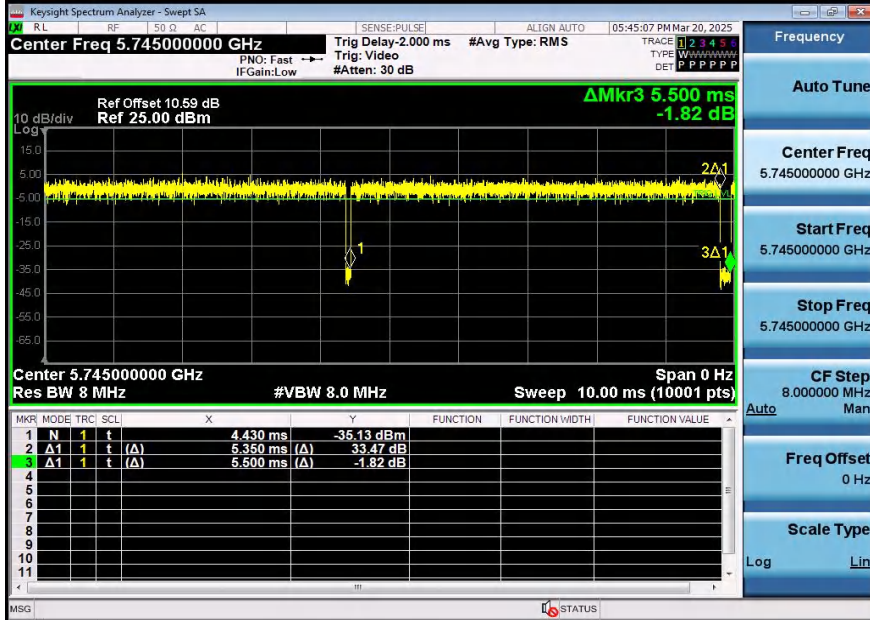
NTNV-11N20SISO-Ant2-5745
