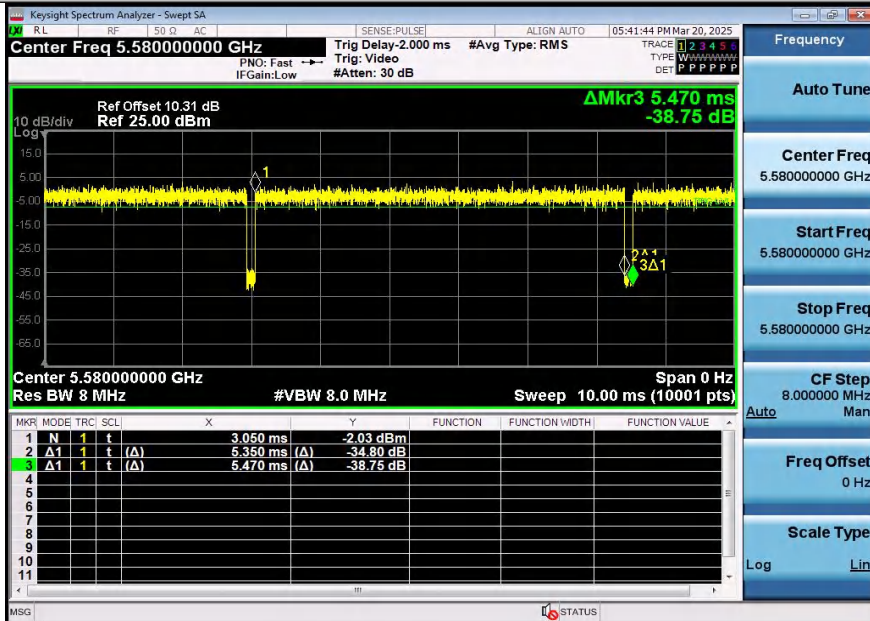
NTNV-11N20SISO-Ant2-5580
