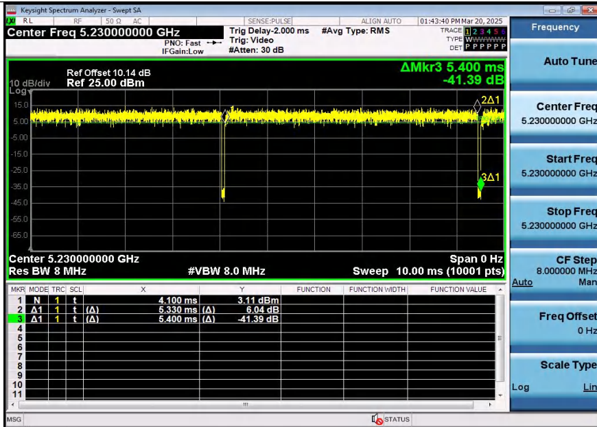
NTNV-11AC40SISO-Ant2-5230
