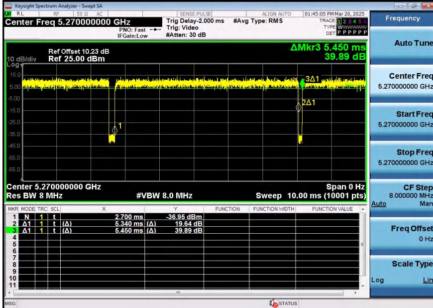
NTNV-11AC40SISO-Ant2-5270
