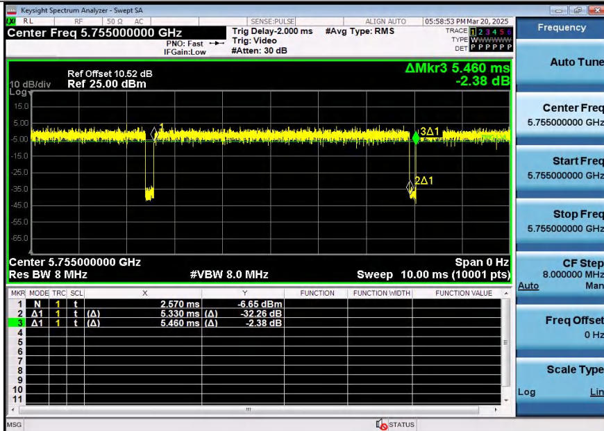
NTNV-11N40SISO-Ant2-5755
