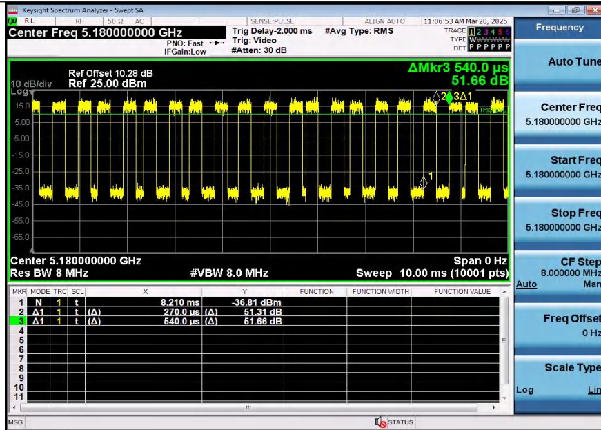
NTNV-11A-Ant2-5180
