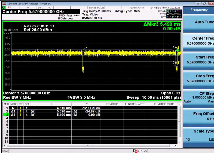
NTNV-11AC160SISO-Ant1-5570
