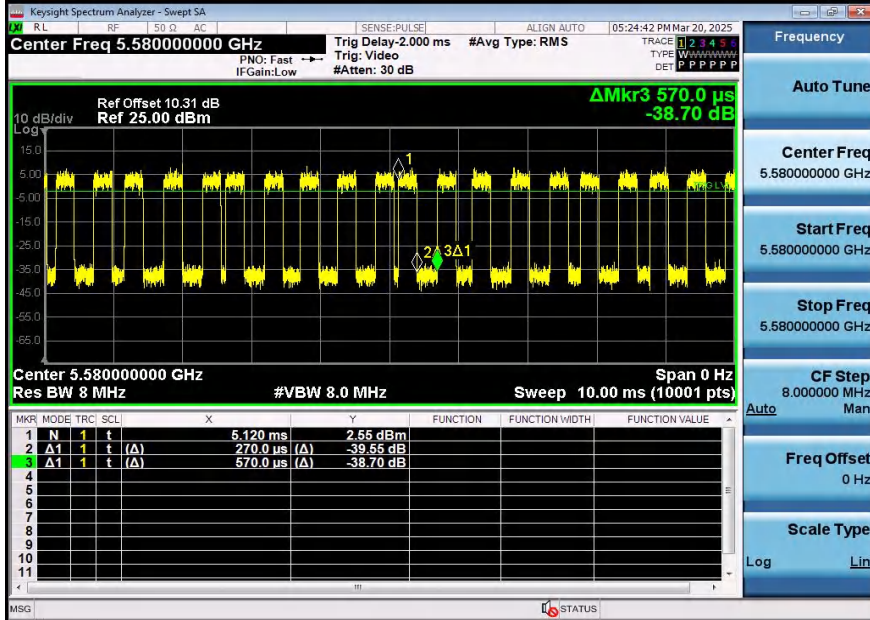
NTNV-11A-Ant2-5580
