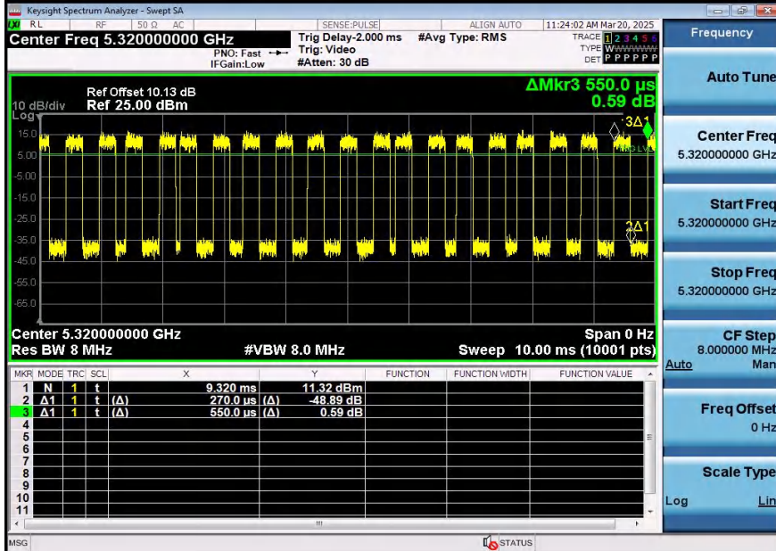
NTNV-11A-Ant2-5320
