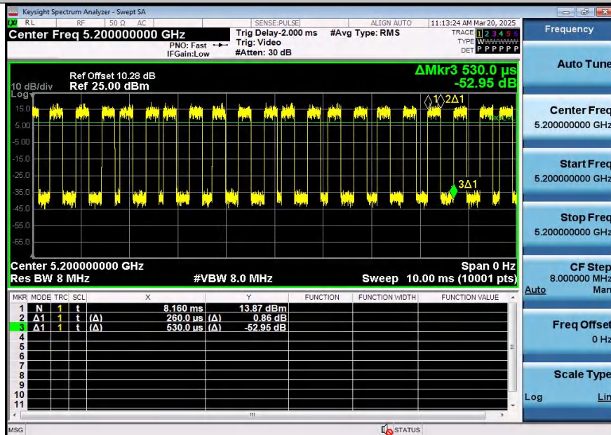
NTNV-11A-Ant2-5200
