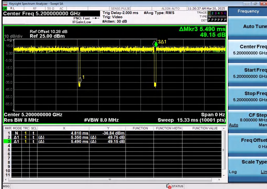
NTNV-11N20SISO-Ant2-5200
