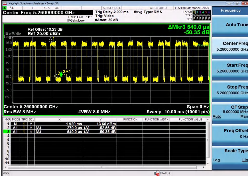
NTNV-11A-Ant2-5260
