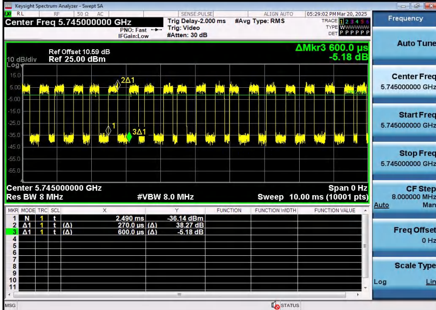
NTNV-11A-Ant2-5745
