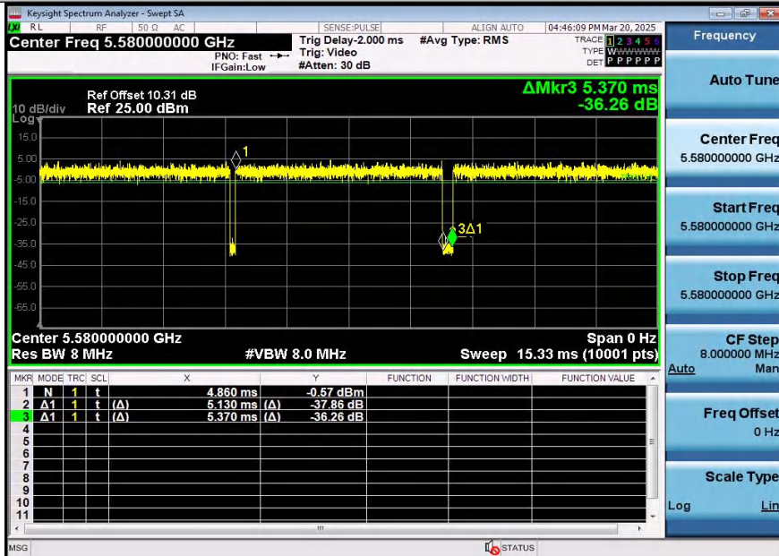
NTNV-11AX20SISO-Ant1-5580
