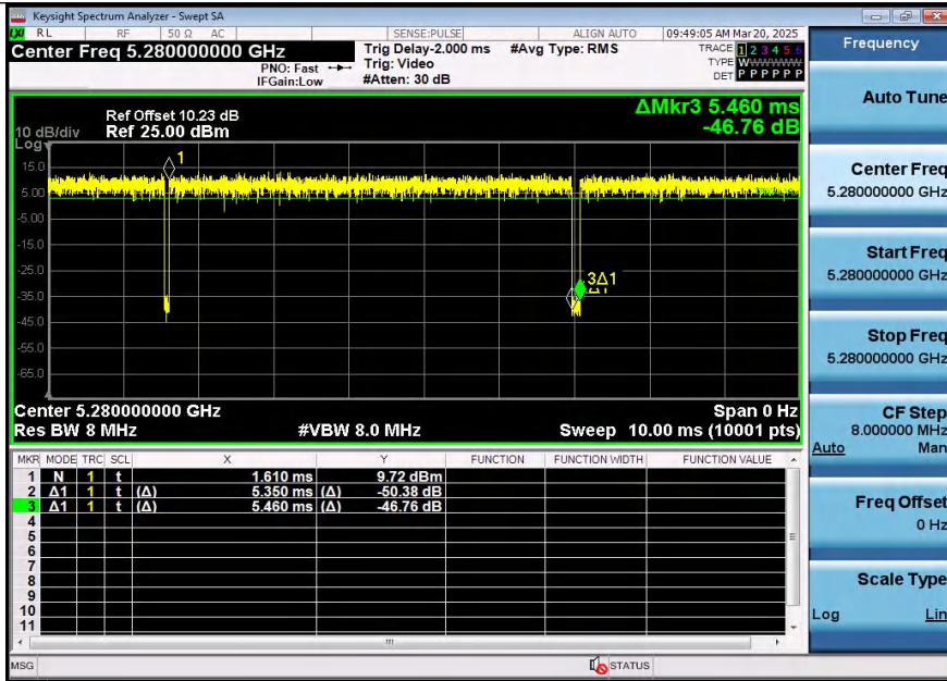
NTNV-11N20SISO-Ant1-5280
