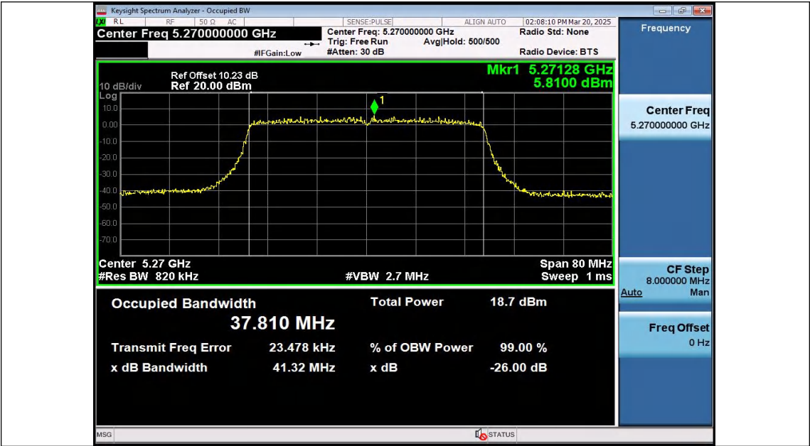
11AX40SISO-Ant2-5270
