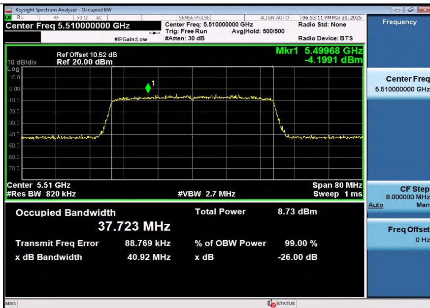
11AX40SISO-Ant2-5510
