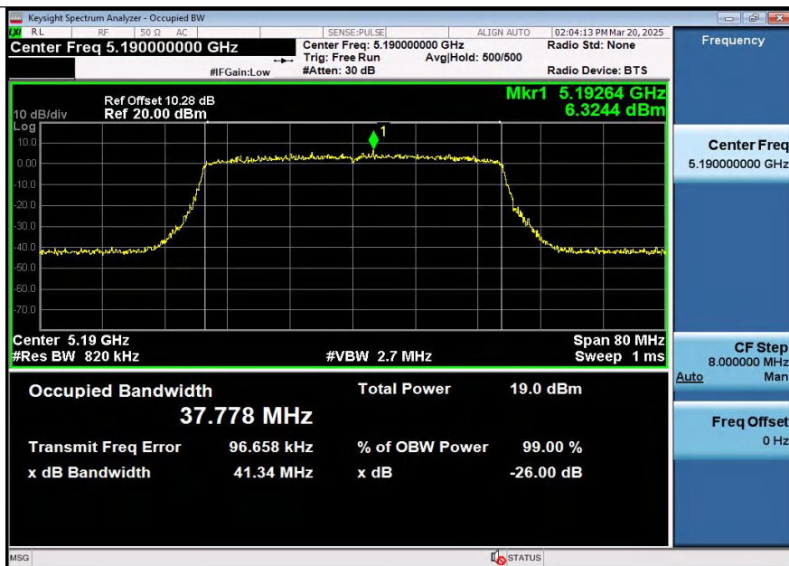
11AX40SISO-Ant2-5190
