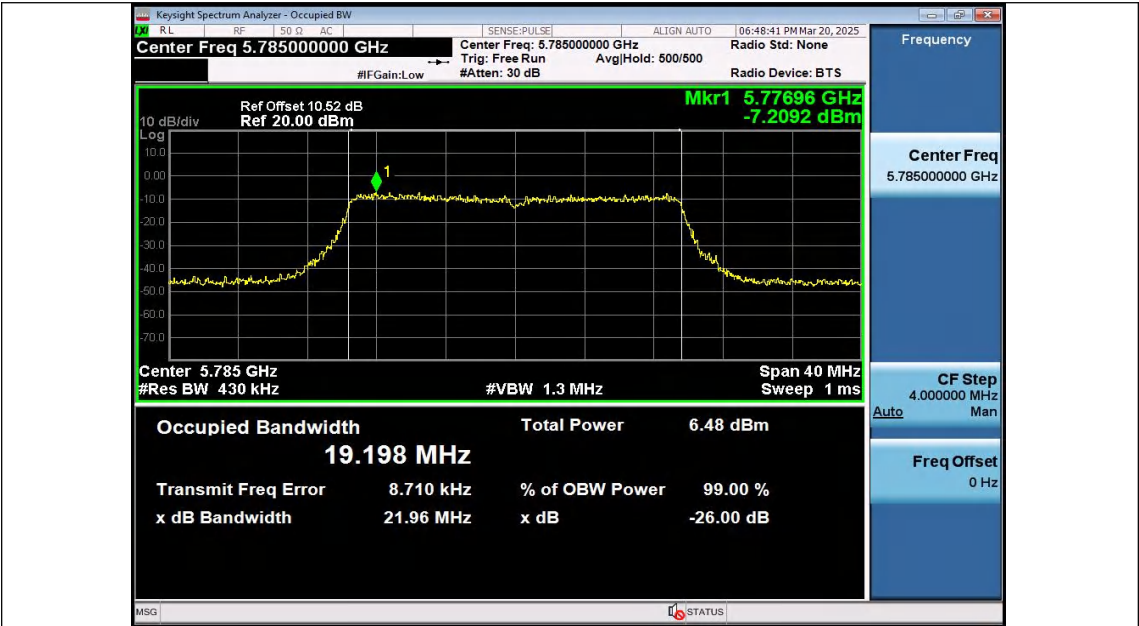
11AX20SISO-Ant2-5785
