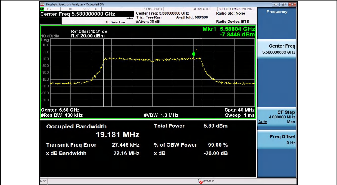
11AX20SISO-Ant2-5580
