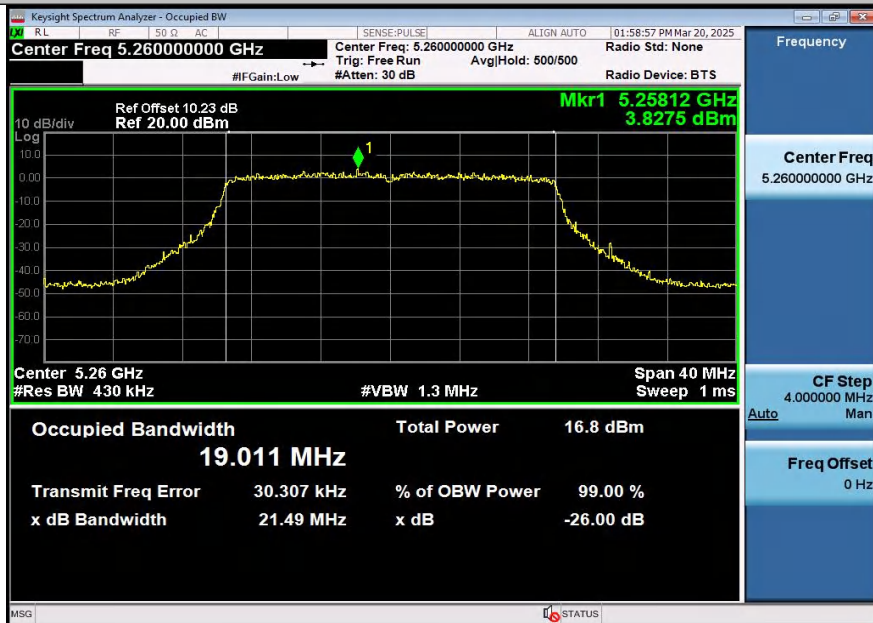
11AX20SISO-Ant2-5260
