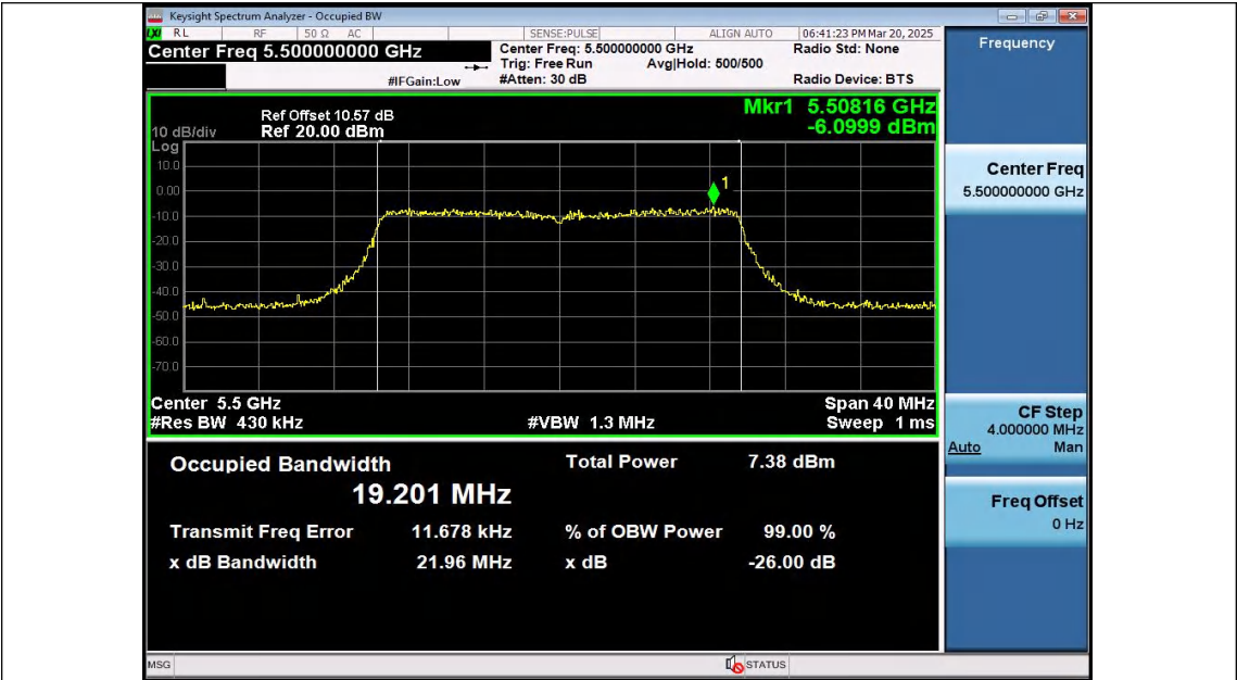
11AX20SISO-Ant2-5500
