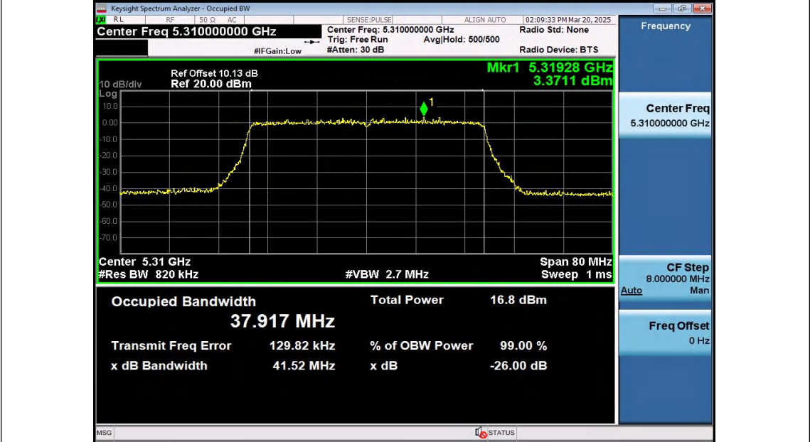
11AX40SISO-Ant2-5310
