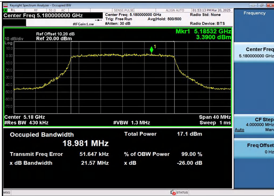
11AX20SISO-Ant2-5180
