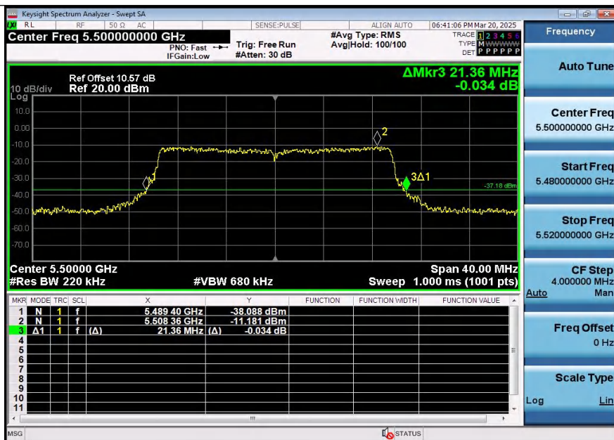
11AX20SISO-Ant2-5500
