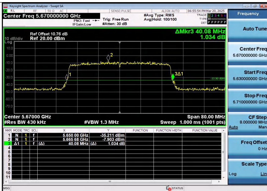
11AX40SISO-Ant2-5670
