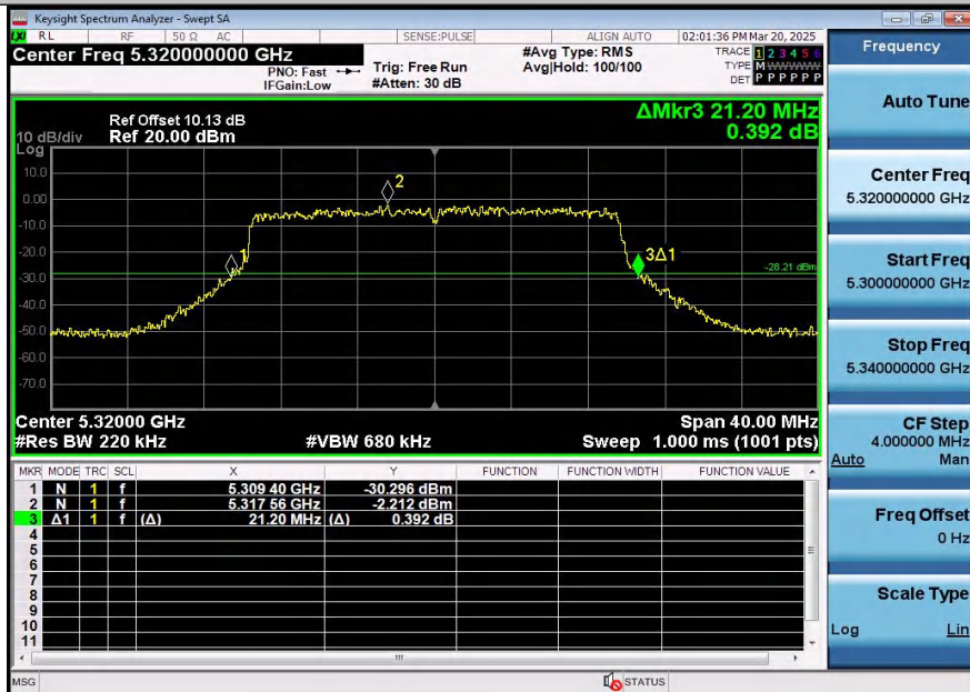
11AX20SISO-Ant2-5320
