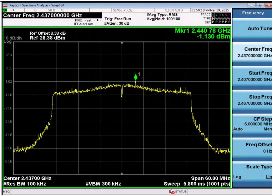
11AX40SISO-Ant1-2437-0~Reference-PASS
