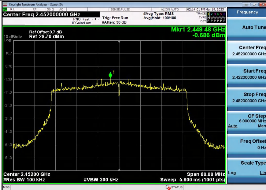
11AX40SISO-Ant1-2452-0~Reference-PASS
