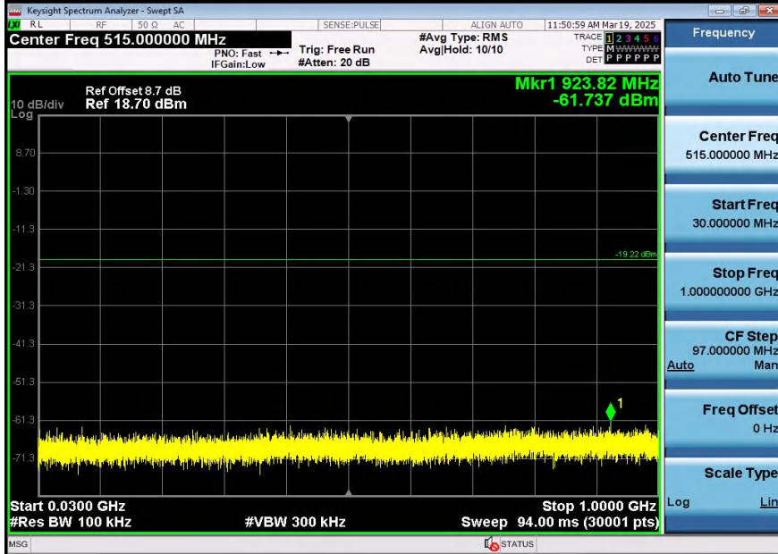
11AX20SISO-Ant1-2462-30~1000-PASS
