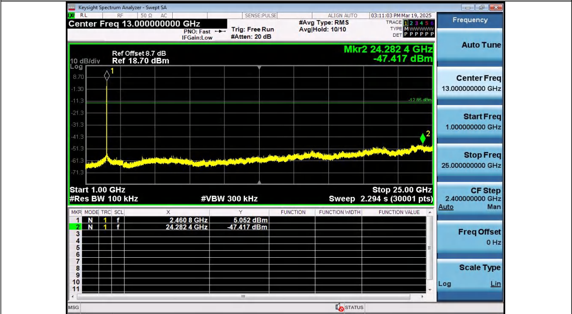
11G-Ant2-2462-1000~25000-PASS
