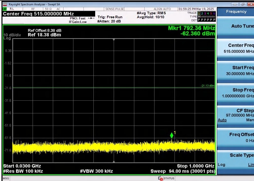
11AX40SISO-Ant1-2437-30~1000-PASS
