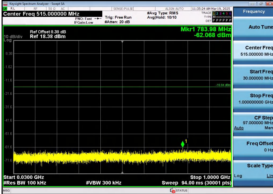
11AX20SISO-Ant1-2412-30~1000-PASS
