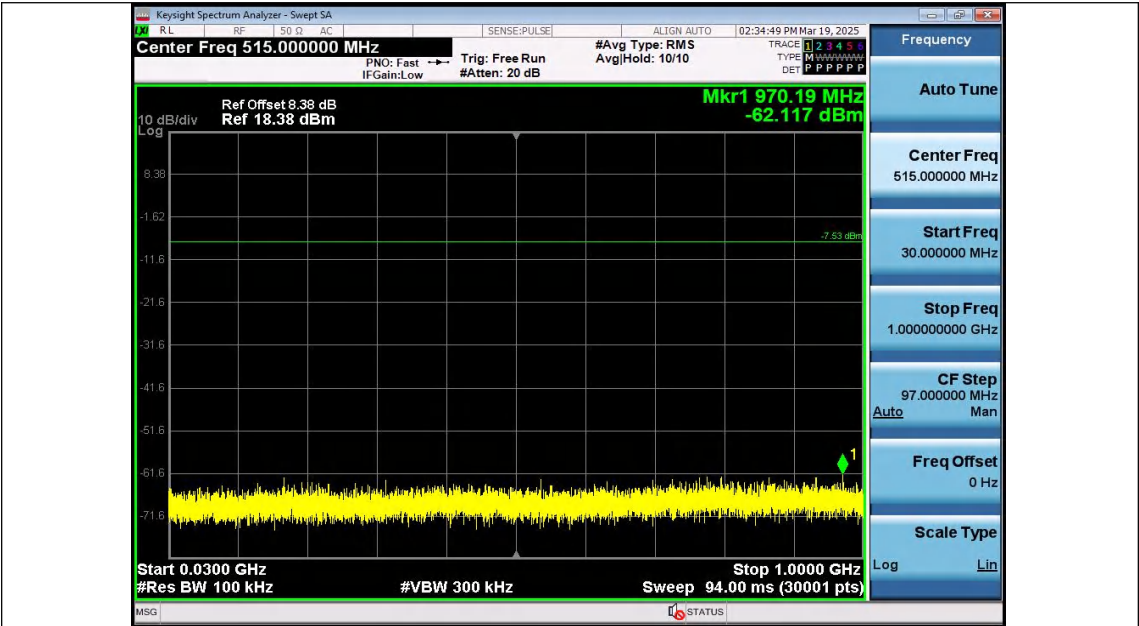
11B-Ant2-2437-30~1000-PASS
