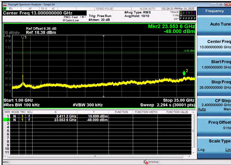
11B-Ant2-2412-1000~25000-PASS
