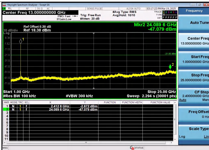
11N20SISO-Ant2-2412-1000~25000-PASS
