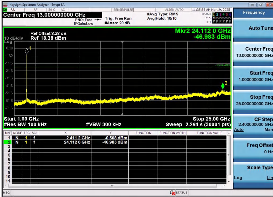
11AX20SISO-Ant1-2412-1000~25000-PASS
