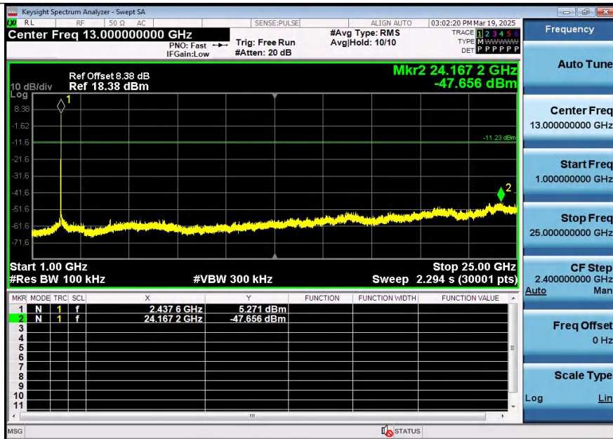
11G-Ant2-2437-1000~25000-PASS
