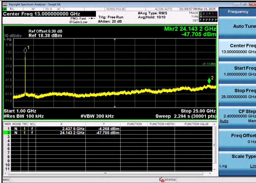
11AX40SISO-Ant1-2437-1000~25000-PASS
