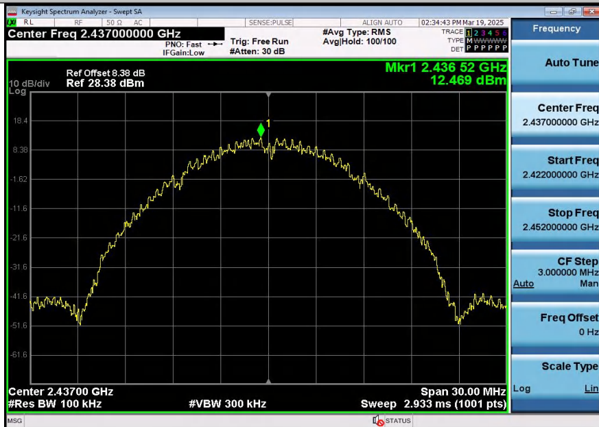
11B-Ant2-2437-0~Reference-PASS
