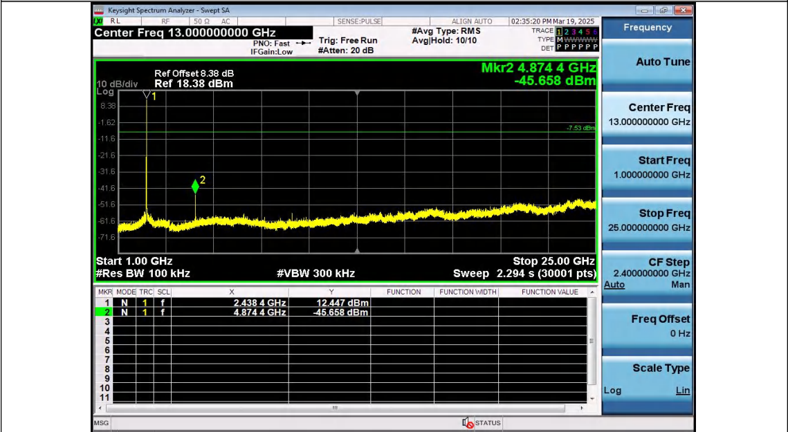
11B-Ant2-2437-1000~25000-PASS
