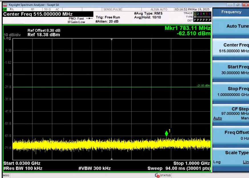
11N20SISO-Ant2-2412-30~1000-PASS
