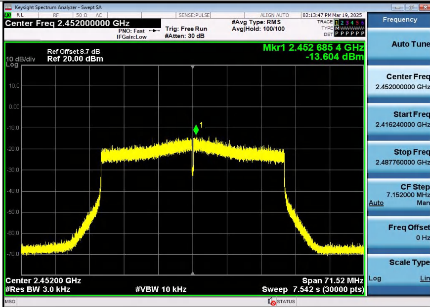
11AX40SISO-Ant1-2452-PASS
