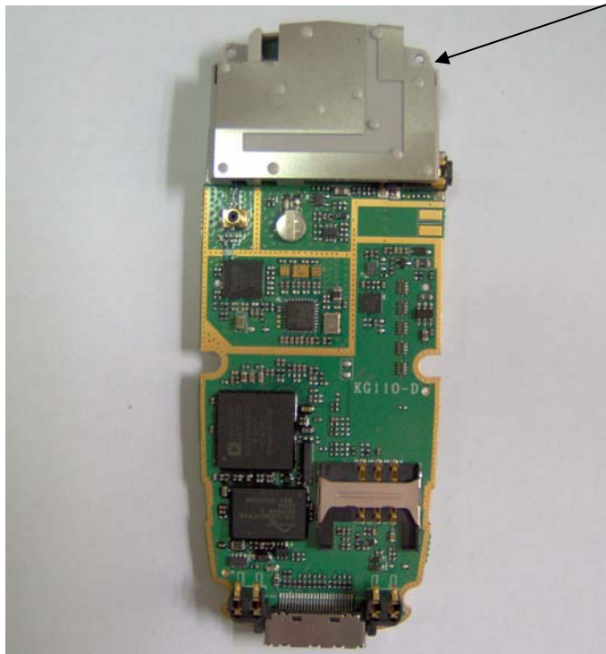
Picture 4: Back view of the PCB with the Antenna
