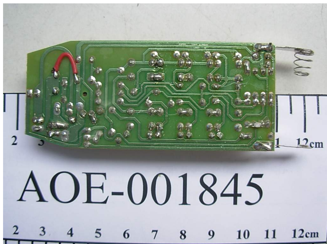
FIGURE 3 REMOTE CONTROL (M/N: RCT-08) MAIN BOARD (SOLDERED SIDE)
