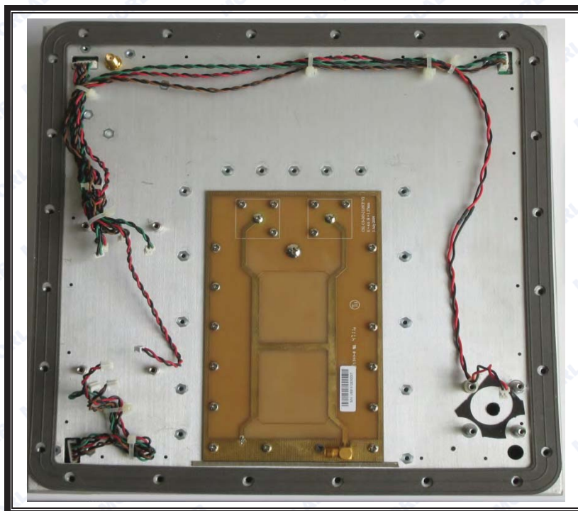
(Plot 4: Antenna 4)
